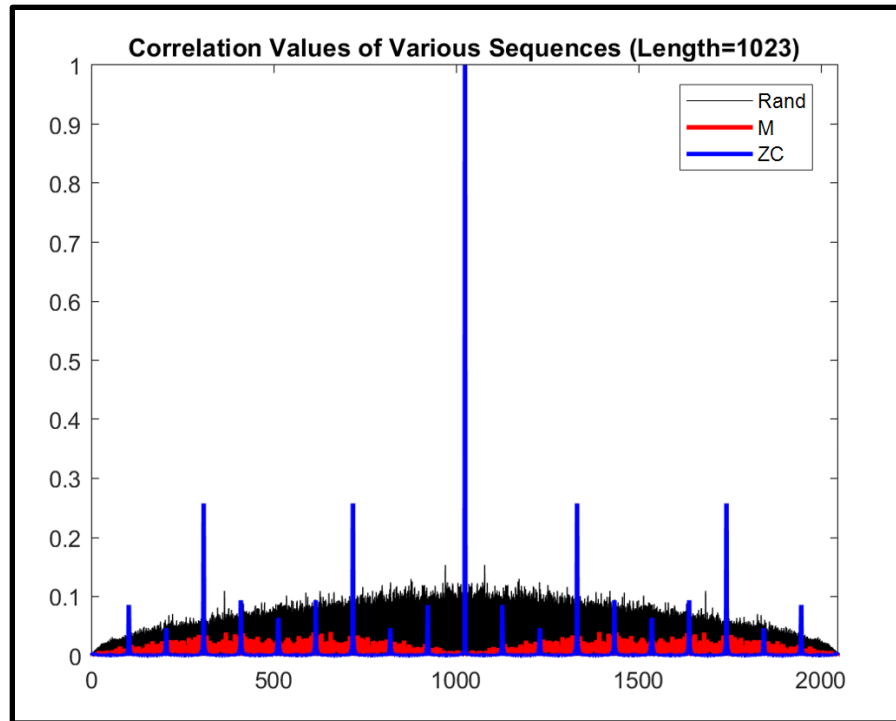
Figure 31. Combined Results of 1000 Random Sequence Autocorrelations
