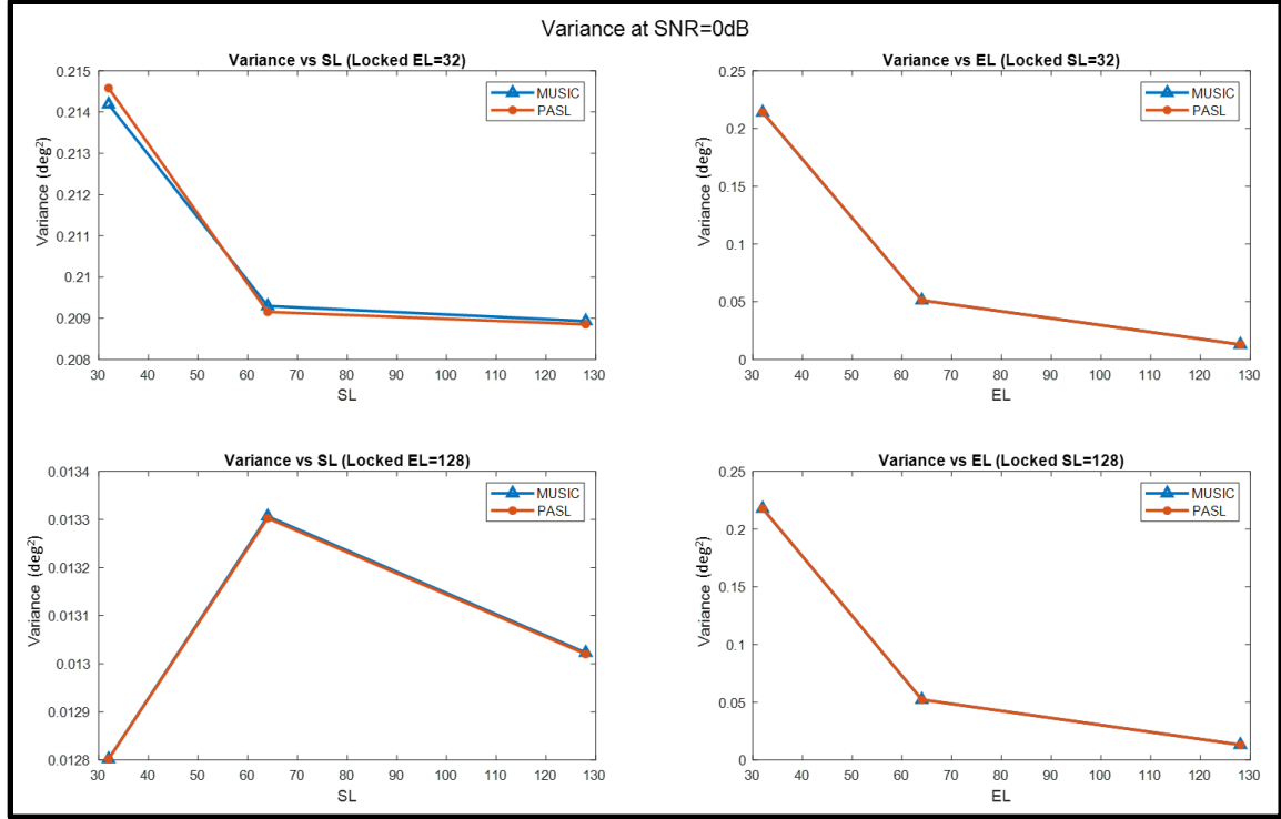
Figure 59. MUSIC and PASL DOA Variance at \text{SNR} = 0 \text{ dB}
