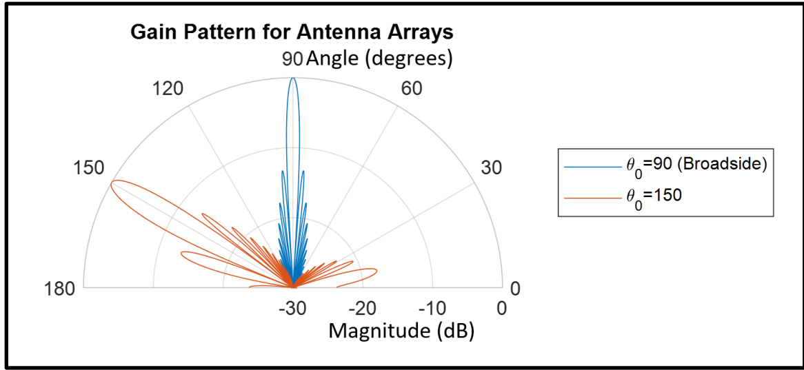
Figure 37. Effects of Scan Angle on Main Lobe HPBW
