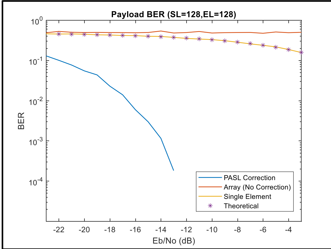
Figure 63. Payload BERs
