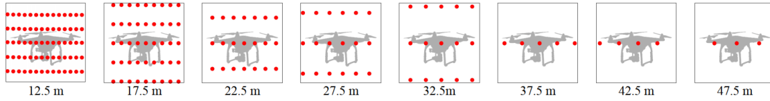
Theoretical scan patterns related to the distances between the target and the LiDAR sensor, with a target outline
