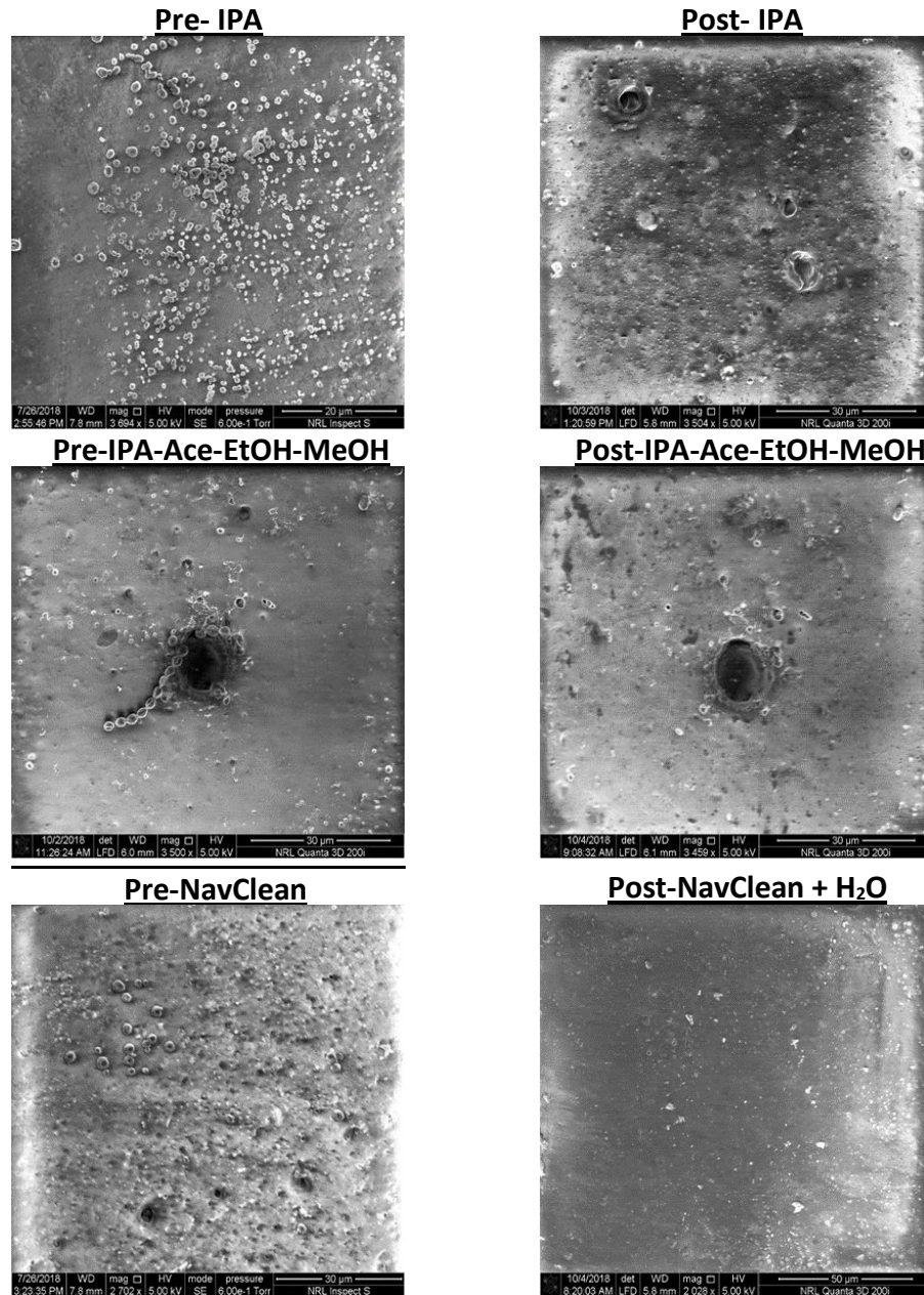
Figure 18. (Group 2): Surface conditions of inoculated chromate primer panels pre- and post-surface cleaning of isolated locations using combinations of iso-propyl alcohol (IPA), acetone (Ace), ethanol (EtOH), methanol (MeOH) and NavClean with a distilled water (dH 2 O) rinse.
