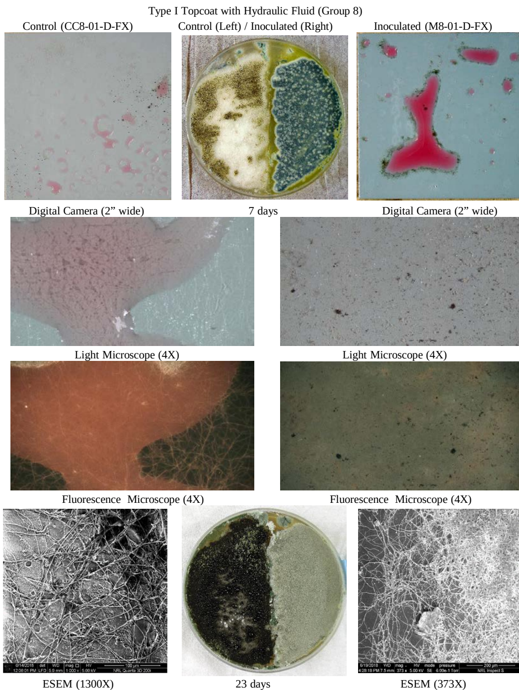
Figure 10. (Group 8): Type I topcoat panels covered with hydraulic fluid and exposed to elevated heat and humidity for 86 days without fungi (control, left) and inoculated (right). Potato dextrose agar culture plates were inoculated with swabs taken from the panels after 86-day exposure; left side of the plate was swabbed from the control panel, while the right side was swabbed from the inoculated panel. Culture plates are shown at 7 and 23 days after inoculation.
