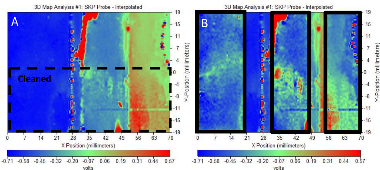
Figure 32. CPD map of Group 7 samples. Panels arranged from left to right C7, M7, and CC7. A) Full scan with color scale set to overall scan maximum scale B) Same scan data as A but with each black boxed panel section individually set to color scale maximum for just that boxed section.
