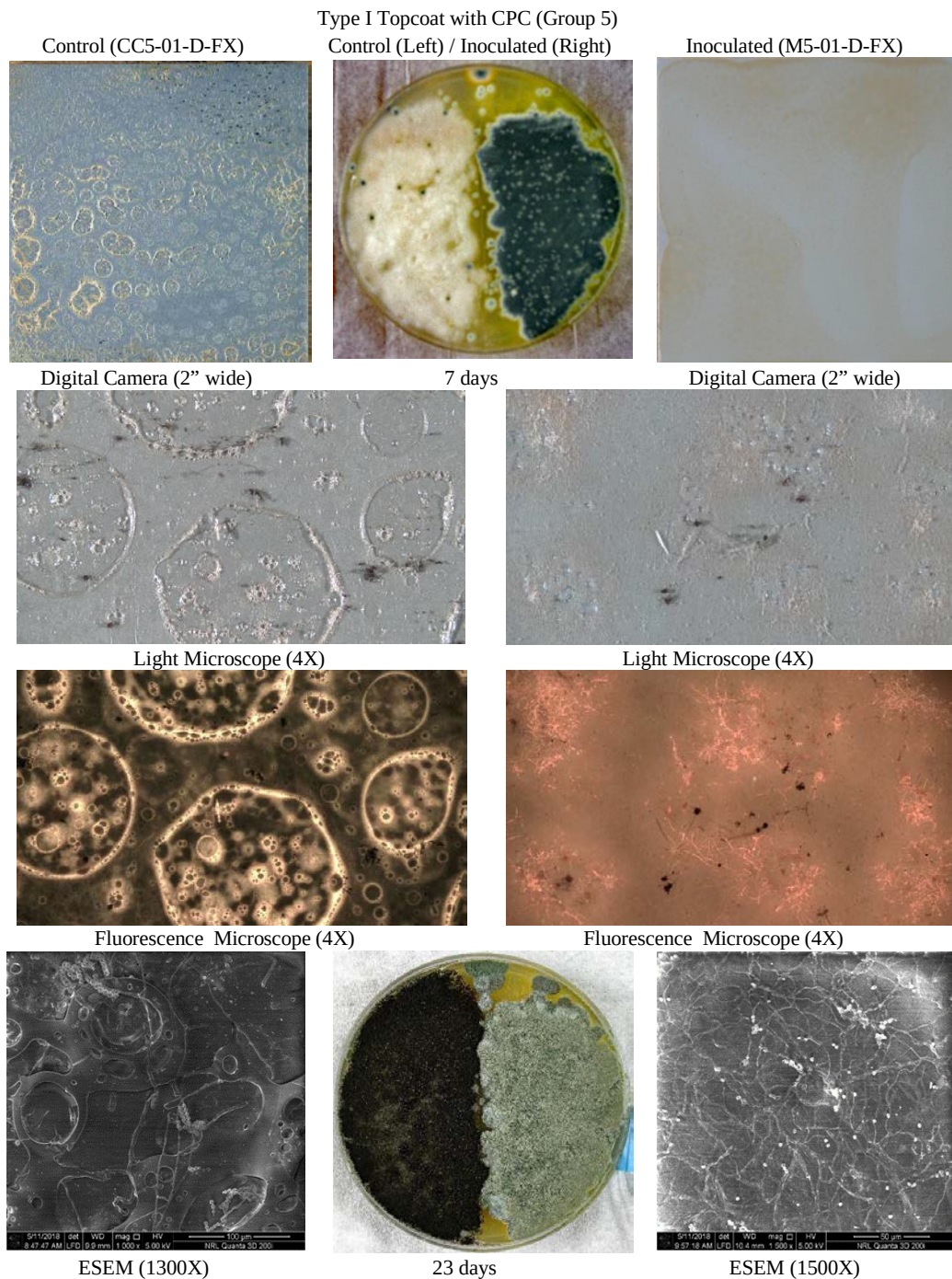
Figure 12. (Group 5): Type I topcoat panels covered with Cor-Ban 35 corrosion preventive compound (CPC) and exposed to elevated heat and humidity for 86 days without fungi (control, left) and inoculated (right). Potato dextrose agar culture plates were inoculated with swabs taken from the panels after 86-day exposure; left side of the plate was swabbed from the control panel, while the right side was swabbed from the inoculated panel. Culture plates are shown at 7 and 23 days after inoculation.
