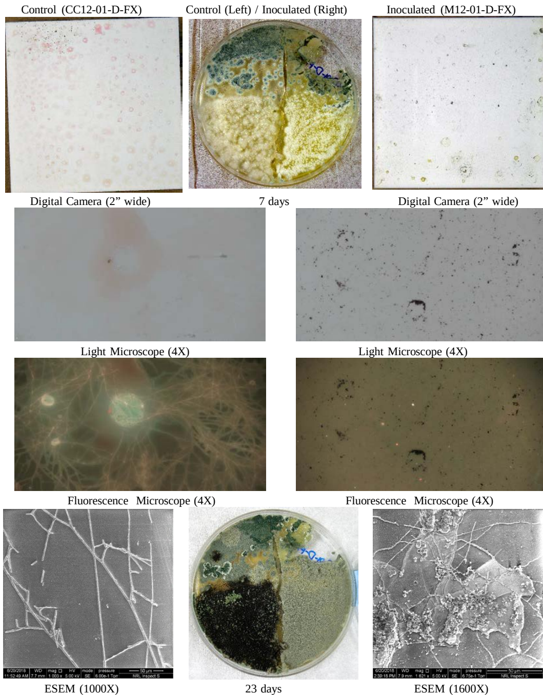
Figure 11. (Group 12): Type I topcoat panels covered with hydraulic fluid and exposed to elevated heat and humidity for 86 days without fungi (control, left) and inoculated (right). Potato dextrose agar culture plates were inoculated with swabs taken from the panels after 86-day exposure; left side of the plate was swabbed from the control panel, while the right side was swabbed from the inoculated panel. Culture plates are shown at 7 and 23 days after inoculation.
