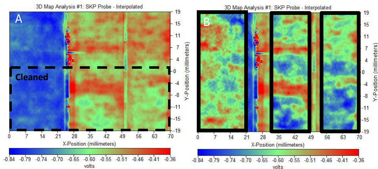
Figure 30. CPD map of Group 3 samples. Panels arranged from left to right C3, M3, and CC3. A) Full scan with color scale set to overall scan maximum scale B) Same scan data as A but with each black boxed panel section individually set to color scale maximum for just that boxed section.
