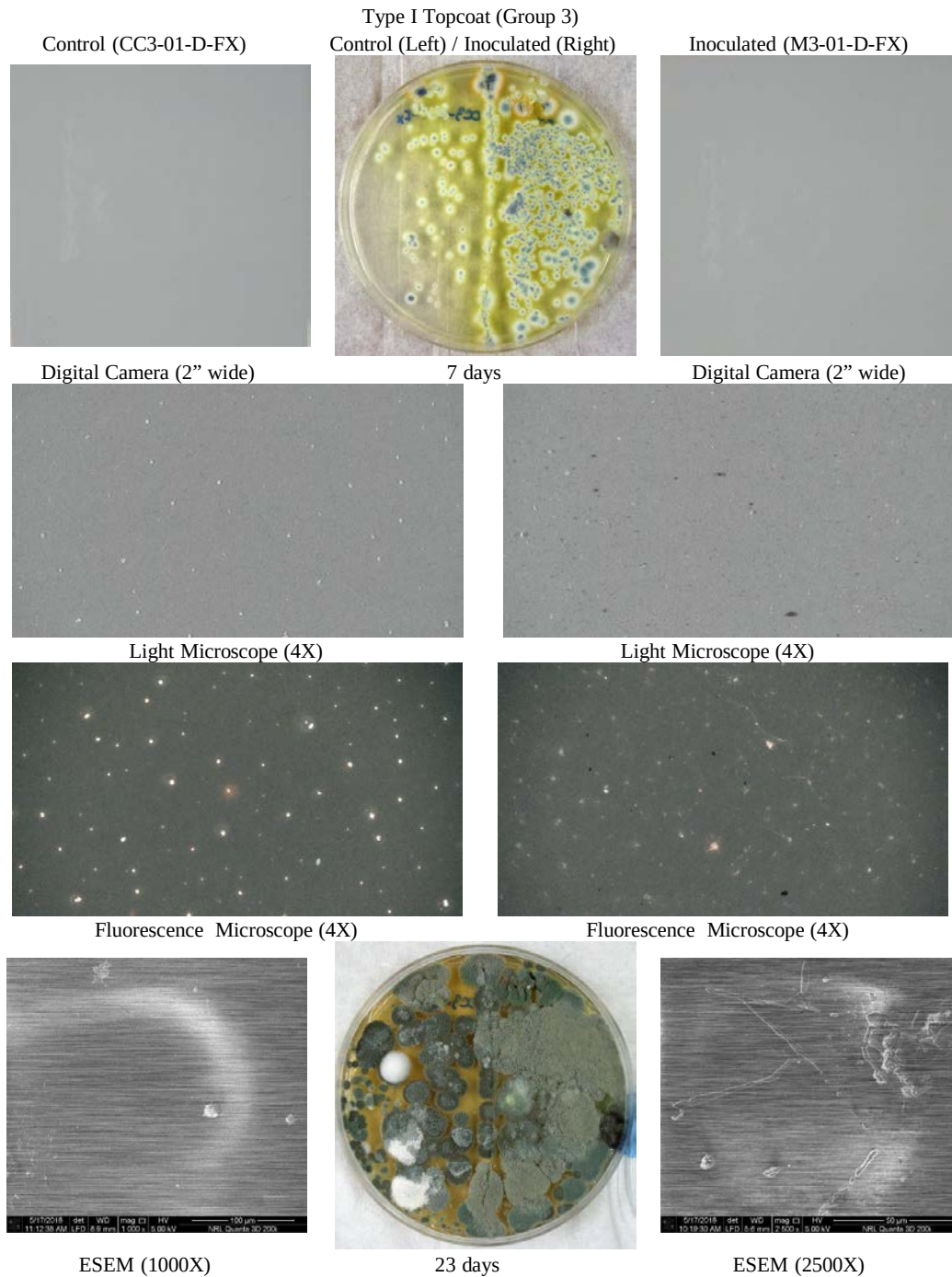
Figure 6. (Group 3): Metal panels covered with Type I topcoat exposed to elevated heat and humidity for 86 days without fungi (control, left) and inoculated (right). Potato dextrose agar culture plates were inoculated with swabs taken from the panels after 86-day exposure; left side of the plate was swabbed from the control panel, while the right side was swabbed from the inoculated panel. Culture plates are shown at 7 and 23 days after inoculation.
