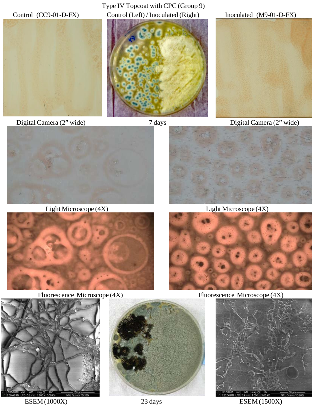
Figure 14. (Group 9) Type IV topcoat panels covered with Cor-Ban 35 corrosion preventive compound (CPC) and exposed to elevated heat and humidity for 86 days without fungi (control, left) and inoculated (right). Potato dextrose agar culture plates were inoculated with swabs taken from the panels after 86-day exposure; left side of the plate was swabbed from the control panel, while the right side was swabbed from the inoculated panel. Culture plates are shown at 7 and 23 days after inoculation.
