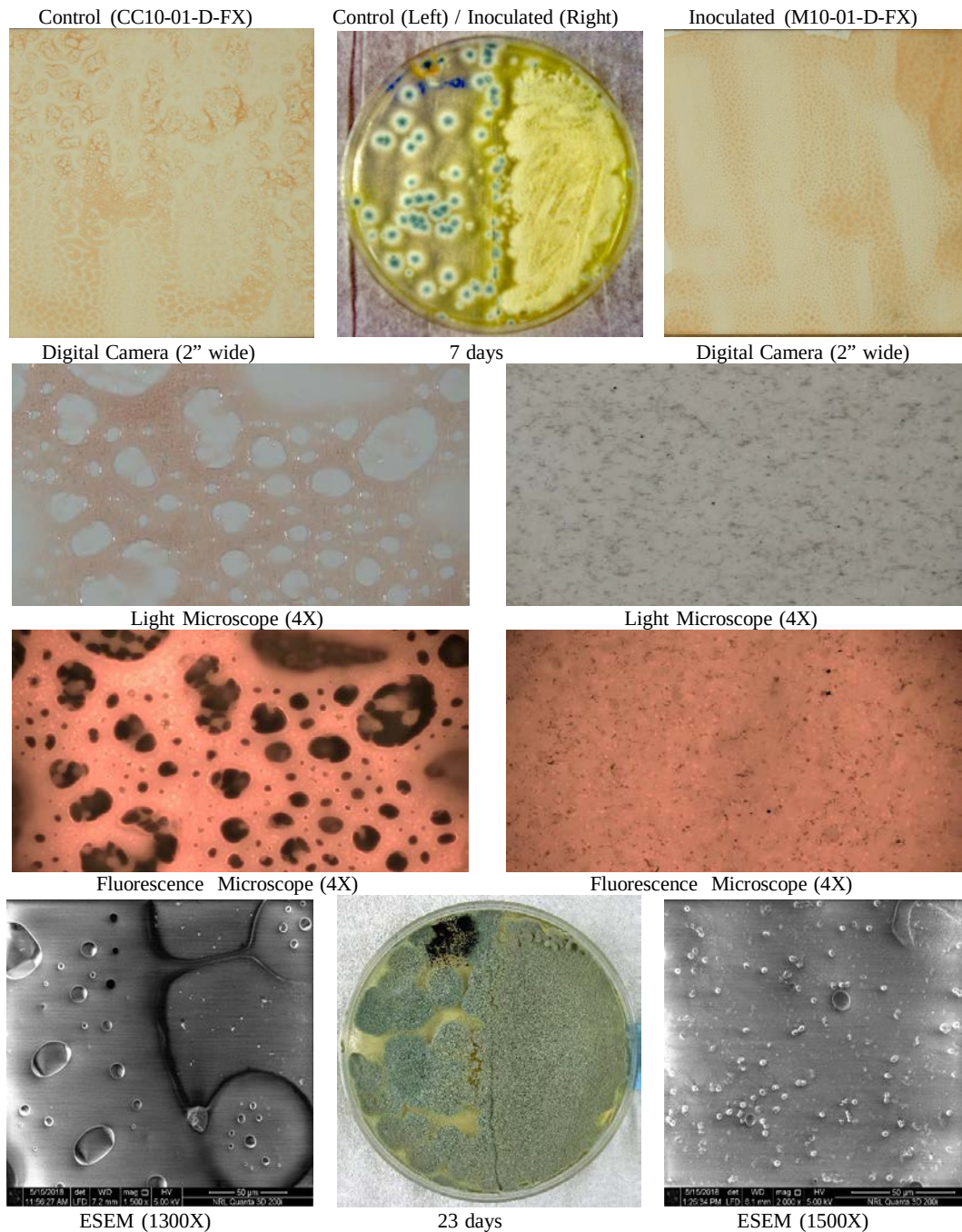
Figure 15. (Group 10) Type IV topcoat panels covered with Cor-Ban 35 corrosion preventive compound (CPC) with Omacide and exposed to elevated heat and humidity for 86 days without fungi (control, left) and inoculated (right). Potato dextrose agar culture plates were inoculated with swabs taken from the panels after 86-day exposure; left side of the plate was swabbed from the control panel, while the right side was swabbed from the inoculated panel. Culture plates are shown at 7 and 23 days after inoculation.
