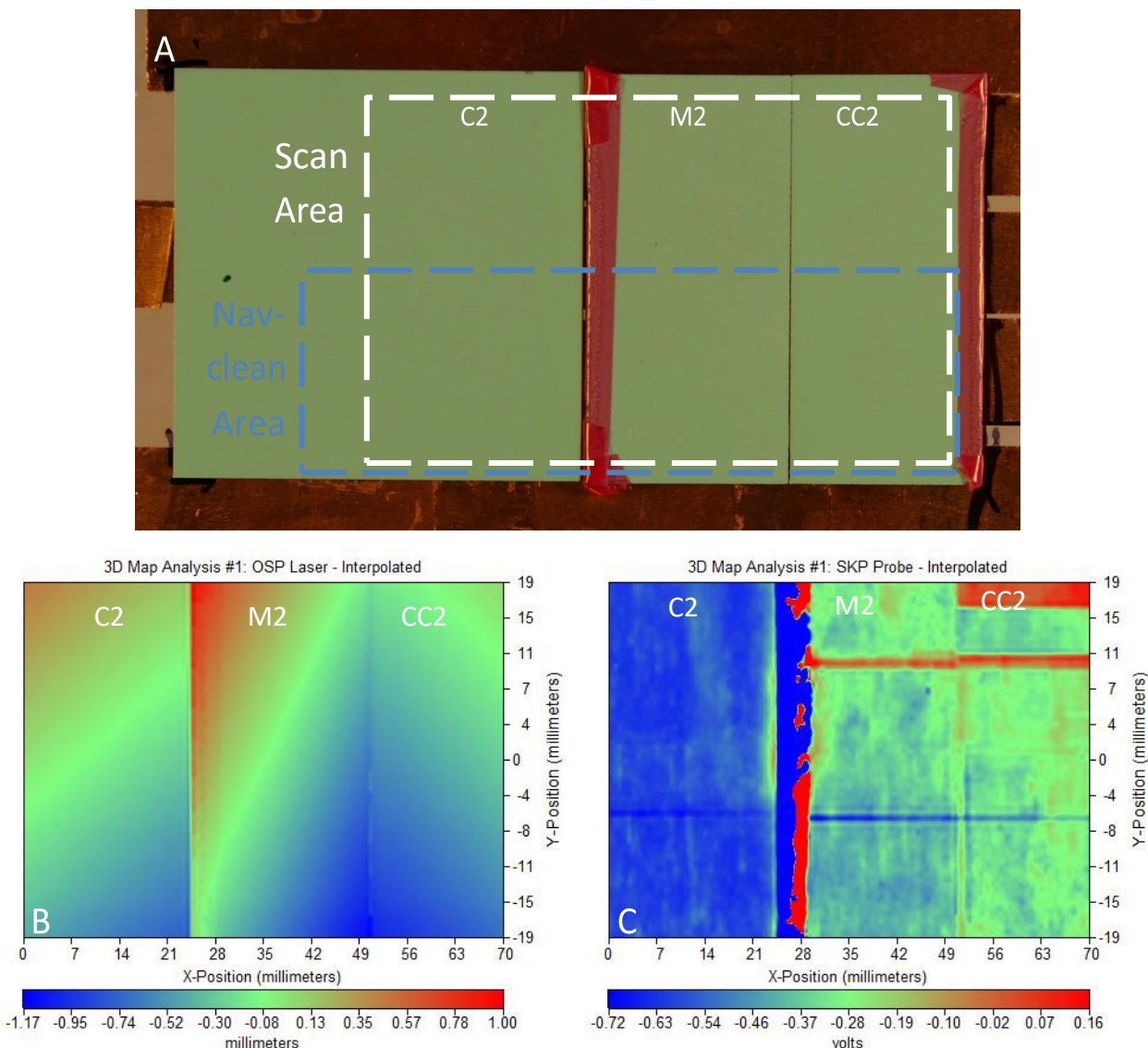
Figure 27. Samples from left to right: C2, M2, and CC2 with top half as received, bottom half cleaned with Navclean. A) Optical image B) Optical surface profilometry map, adjusted to remove gaps between panels C) SKP area map.
