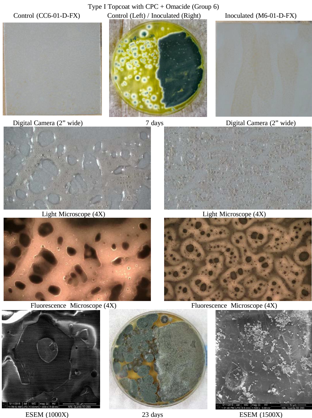
Figure 13. (Group 6): Type I topcoat panels covered with Cor-Ban 35 corrosion preventive compound (CPC) with Omacide and exposed to elevated heat and humidity for 86 days without fungi (control, left) and inoculated (right). Potato dextrose agar culture plates were inoculated with swabs taken from the panels after 86-day exposure; left side of the plate was swabbed from the control panel, while the right side was swabbed from the inoculated panel. Culture plates are shown at 7 and 23 days after inoculation.
