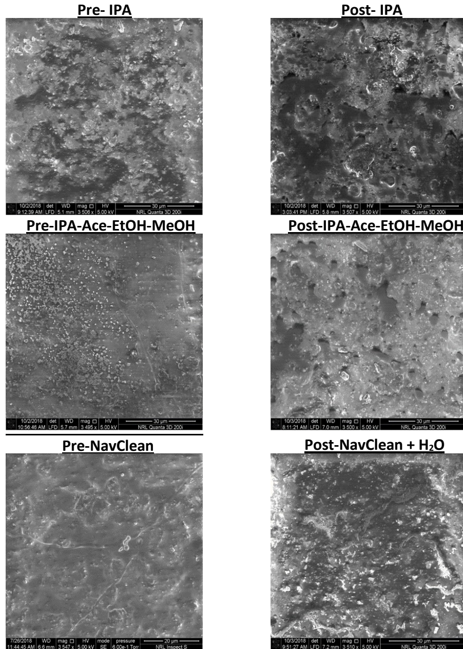
Figure 17. (Group 1): Surface conditions of inoculated chromate primer panels pre- and post-surface cleaning of separate isolated locations using combinations of iso-propyl alcohol (IPA), acetone (Ace), ethanol (EtOH), methanol (MeOH) and NavClean with a distilled water (dH 2 O) rinse.
