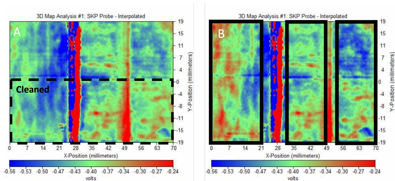
Figure 28. CPD map of Group 1 samples. Panels arranged from left to right C1, M1, and CC1. A) Full scan with color scale set to overall scan maximum scale B) Same scan data as A but with each black boxed panel section individually set to color scale maximum for just that boxed section.
