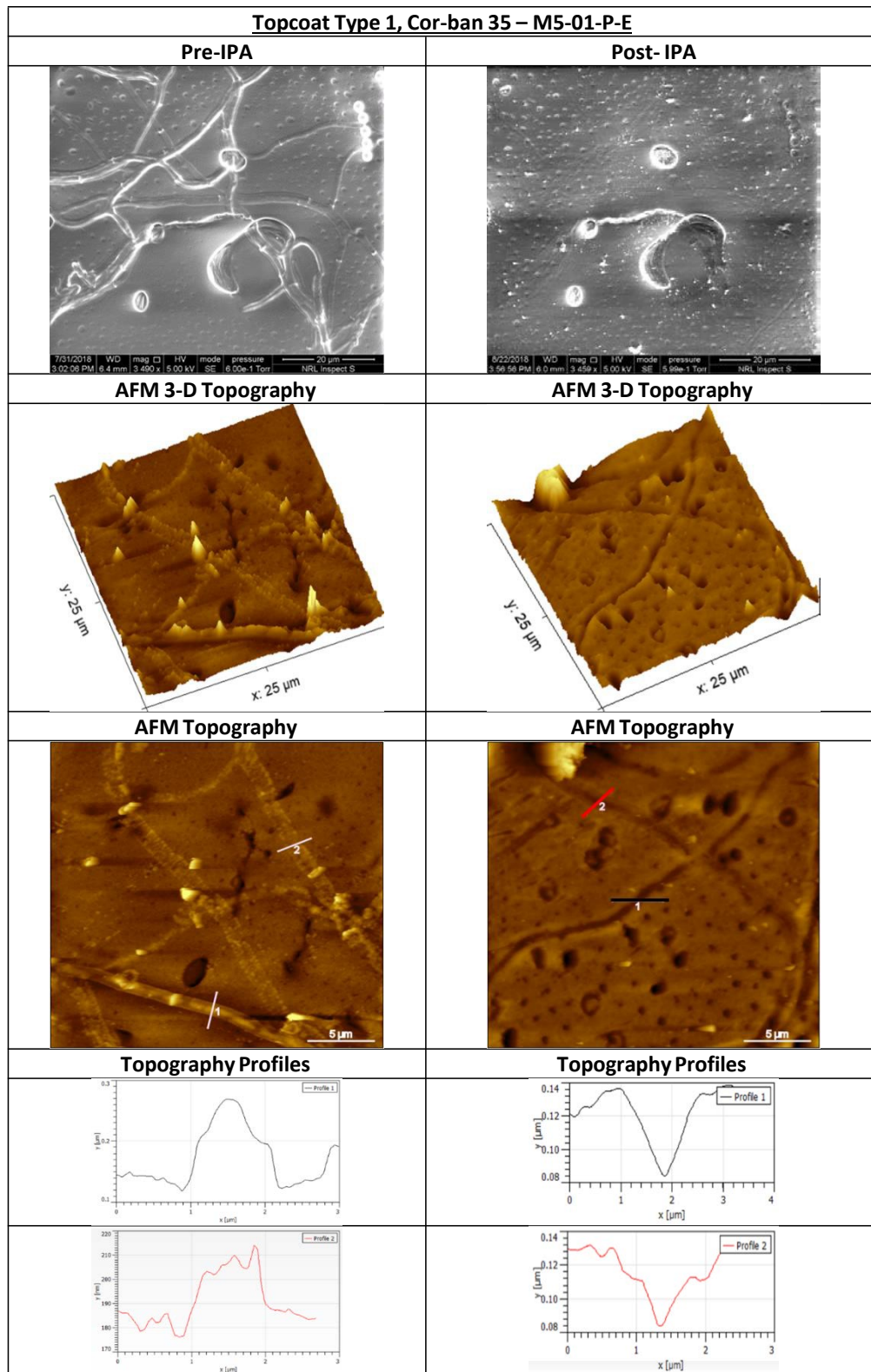
Figure 21. (Group 5): Electron microscopy (top) and atomic force microscopy images (middle) and profiles (bottom) of Type I topcoat with CPC and fungal inoculation pre- and post-cleaning with isopropyl alcohol (IPA).
