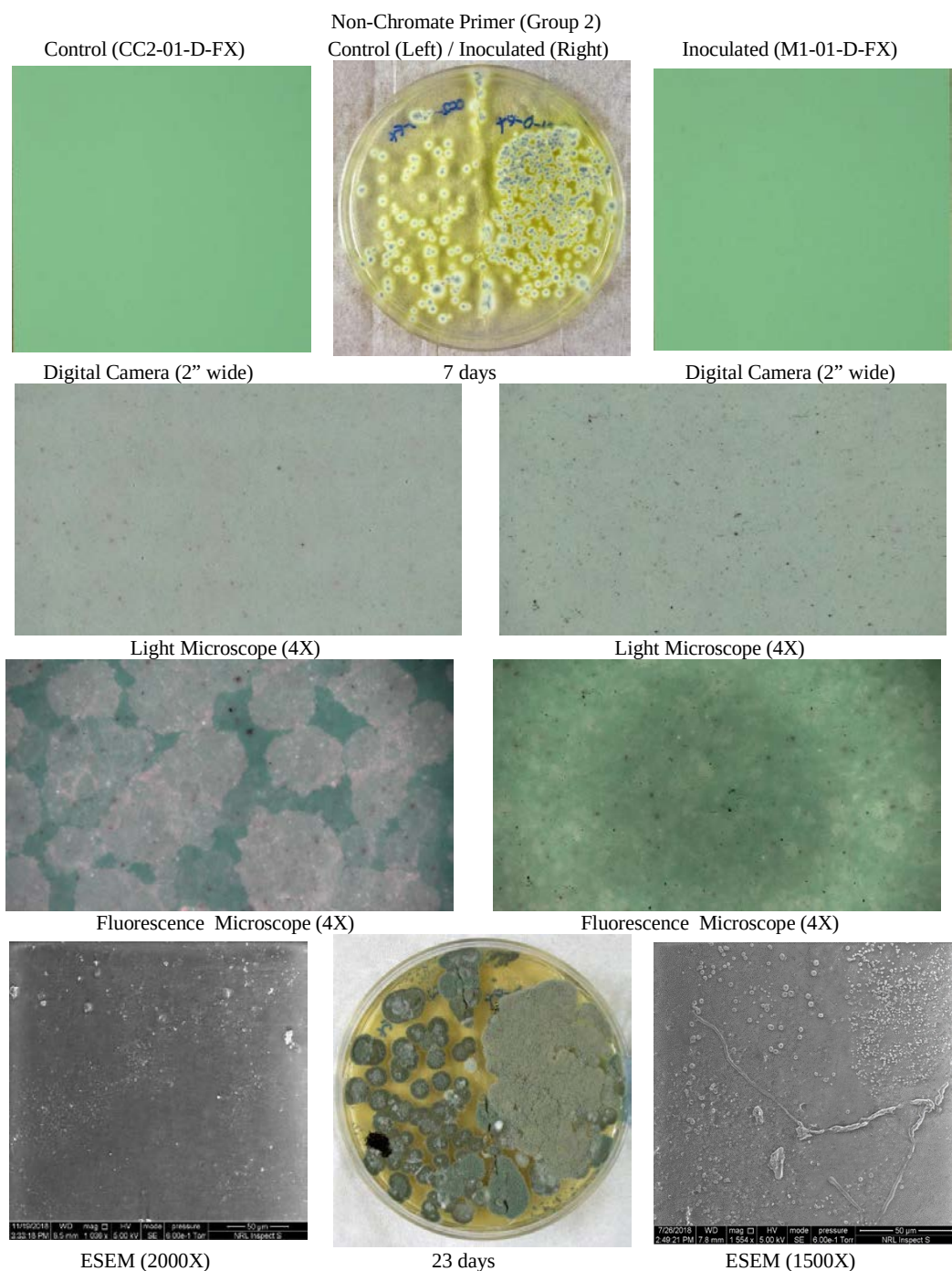
Figure 5. (Group 2): Metal panels covered with non-chromate primer exposed to elevated heat and humidity for 86 days without fungi (control, left) and inoculated (right). Potato dextrose agar culture plates were inoculated with swabs taken from the panels after 86-day exposure; left side of the plate was swabbed from the control panel, while the right side was swabbed from the inoculated panel. Culture plates are shown at 7 and 23 days after inoculation.
