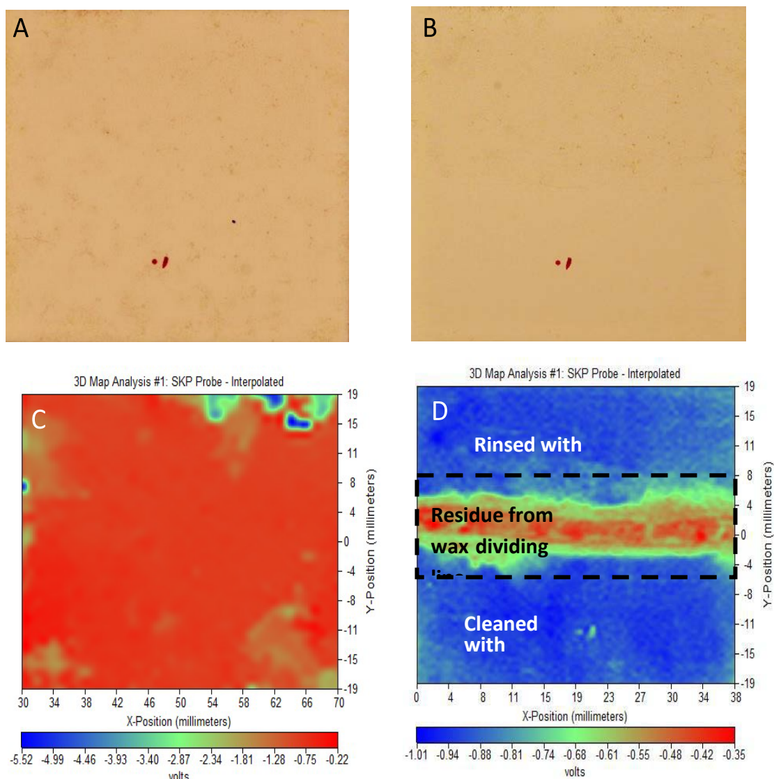
Figure 35. Mold exposed panel with coating type 4, different panel than shown in Figure 32 but with same exposure conditions A) Optical Image before cleaning, with red sharpie marker points. B) Optical Image after bottom half cleaned with NavClean, top half rinsed with water, with red sharpie marker points C) SKP scan before cleaning, without marked points D) SKP scan after cleaning, with marked points and wax residue dividing line across center.
