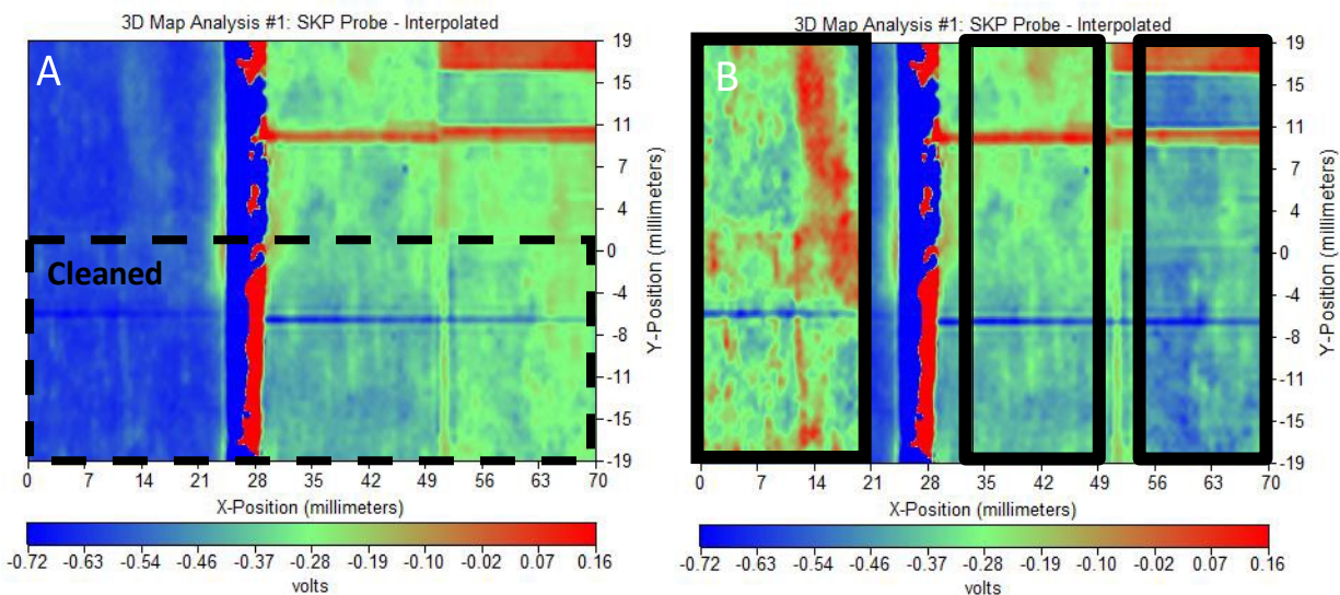
Figure 29 CPD map of Group 2 samples. Panels arranged from left to right C2, M2, and CC2. A) Full scan with color scale set to overall scan maximum scale B) Same scan data as A but with each black boxed panel section individually set to color scale maximum for just that boxed section.
