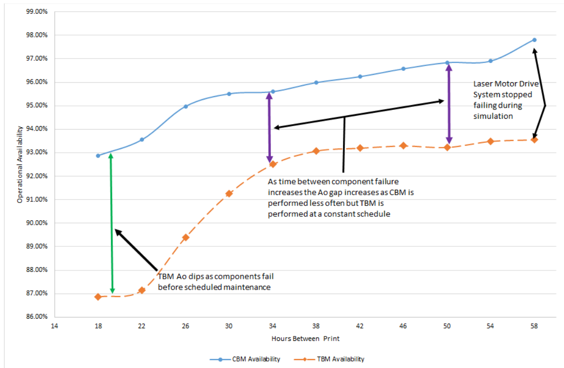
Figure 26. Ao for CBM and TBM with Laser Drive Motor System (~20% MTTF)
