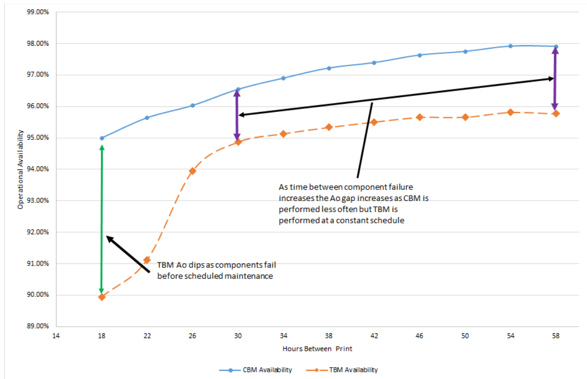
Figure 29. Ao for CBM and TBM without Laser Drive Motor System (-20% MTTF)
