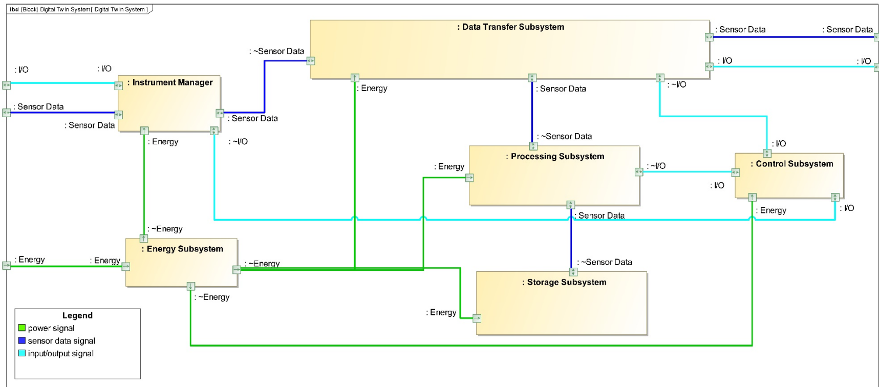
Figure 18. Internal Block Diagram for DT System
