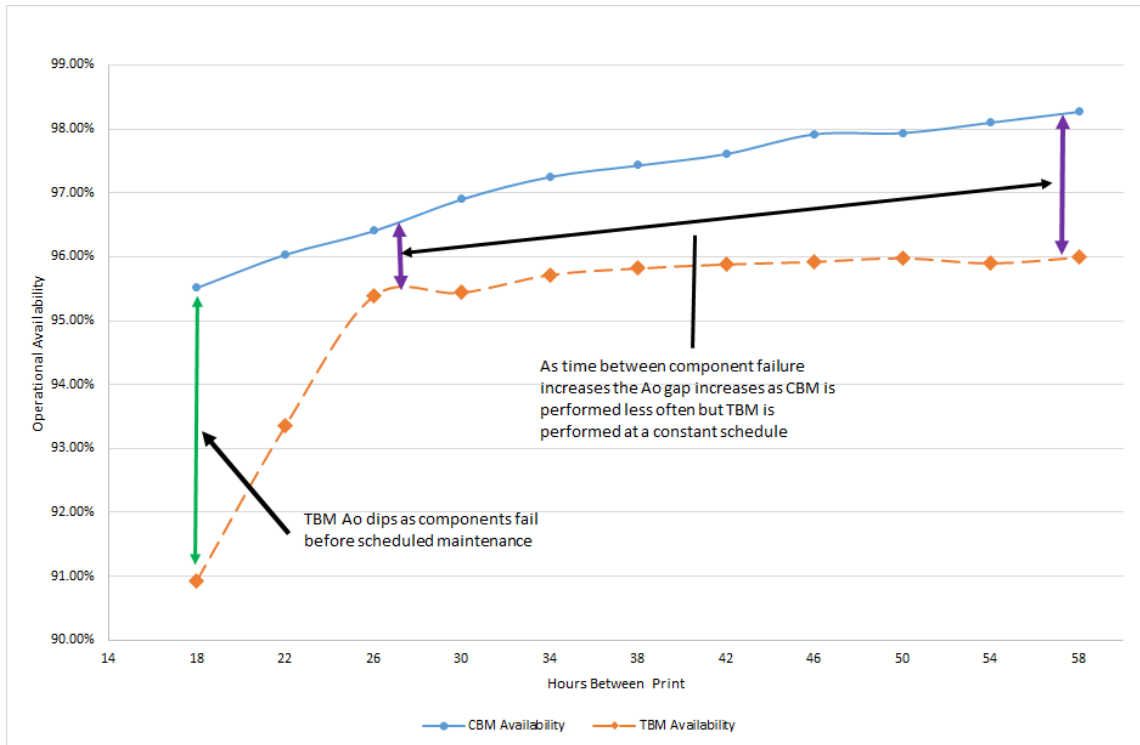
Figure 27. Ao for CBM and TBM without Laser Drive Motor System (+20% MTTF)
