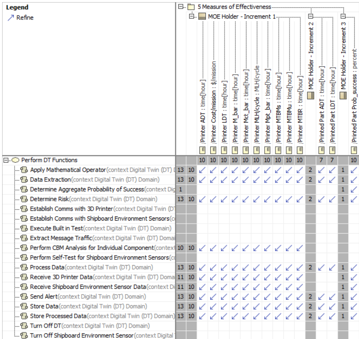
Figure 23. MOE to Activities (RRM)
