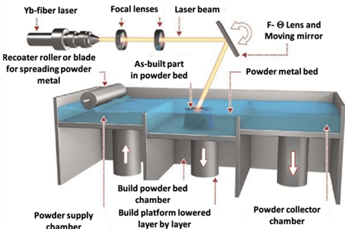
Figure 2. Typical Laser Powder Bed Fusion Printer. Source: Özel et al. (2020).
