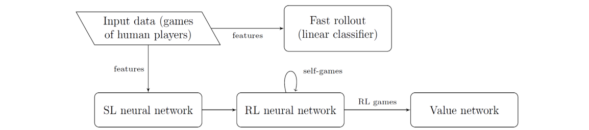
Figure 55. Learning Pipeline of AlphaGo (SL=Supervised Learning, RL=Reinforcement Learning). Source: Hölldobler, Möhle, and Tiginova (2017, fig. 5).
