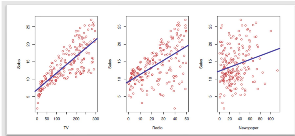
Figure 45. Sales as a Function of Budget. Source: James et al. (2017, 16).
