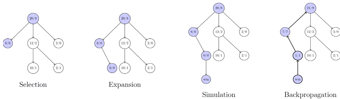
Figure 54. MCTS (All Visits/Winning Visits is the Value in Each Node).
