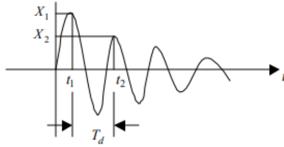
Figure 84. Successive Peaks for Logarithmic Decrement. Source: [61].
