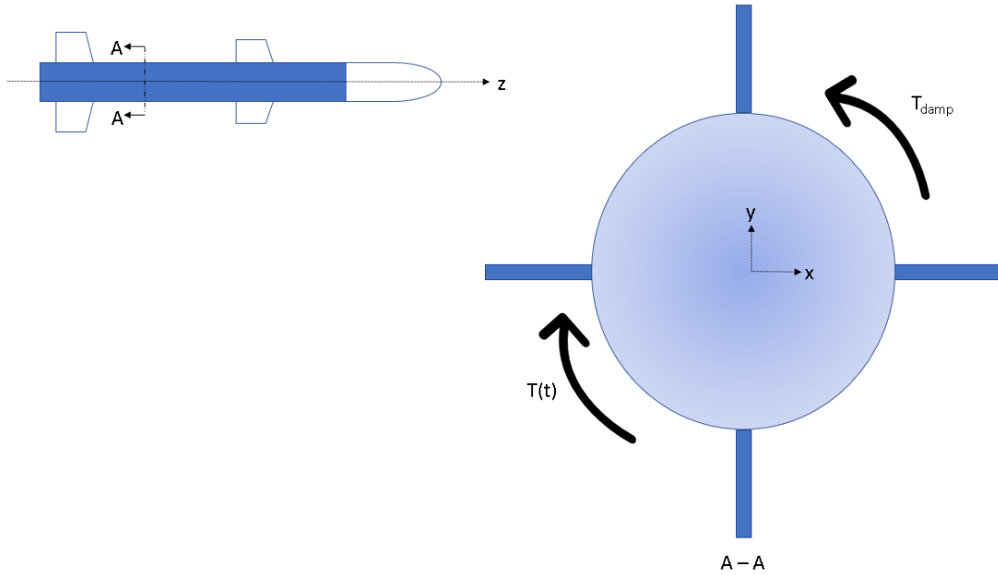
Figure 10. Rocket Cross-Section
