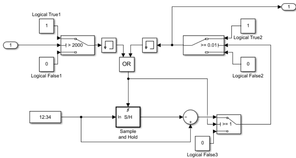
Figure 102. Activation Block Expanded.
