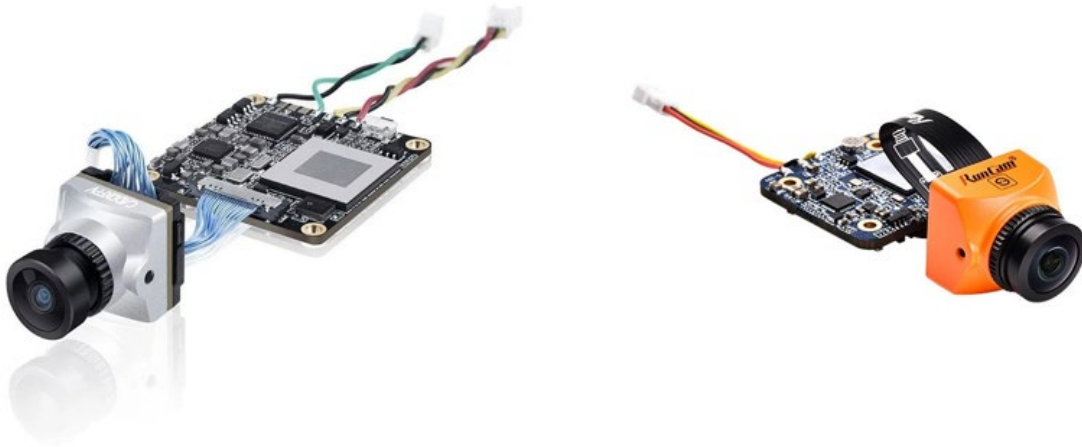
Figure 59. Caddx Lorriss 4K Camera (left) and RunCam Split Mini 2 (right). Source: [53] (left) and [54] (right).
