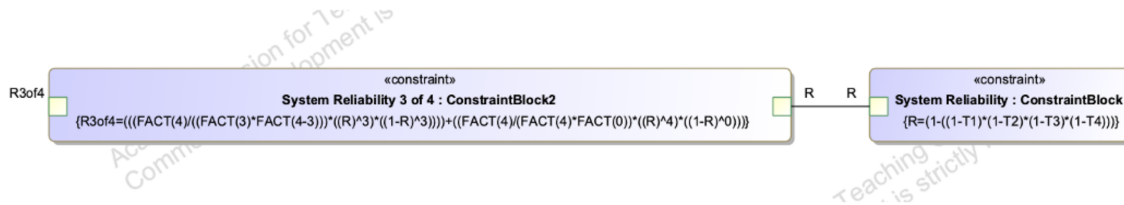
Figure 4.4. Parametric diagram of fuel turbine system showing 3 of 4 system reliability
