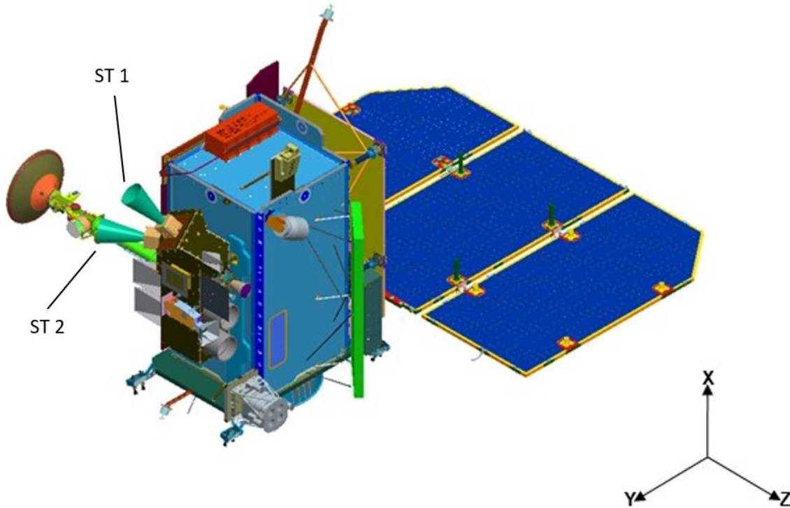
Figure 2.2. Body coordinate system. Source: [5].
