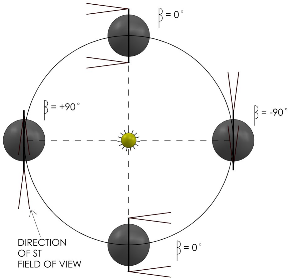
Figure 2.5. Relationship between beta angle ( \beta ) and star tracker occultations
