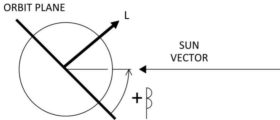
Figure 2.4. Beta angle definition
