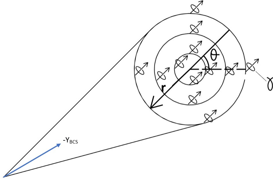
Figure 3.4. Cone of freedom for -y -axis pointing to Sun vector
