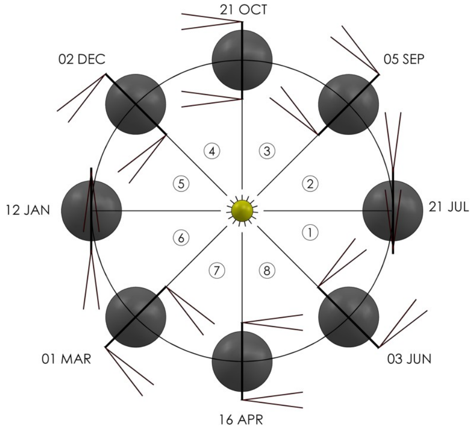
Figure 3.10. Bi-quarterly attitude update scheme based on Moon position
