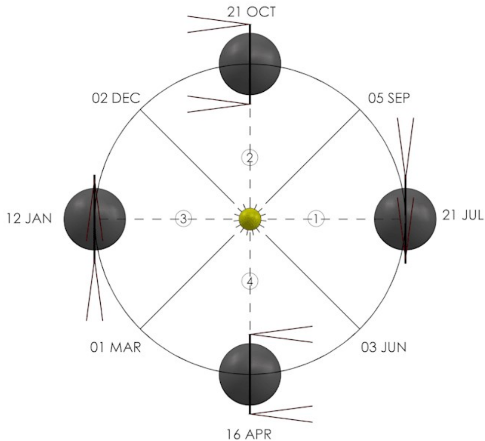
Figure 3.9. Quarterly attitude update scheme based on Moon position
