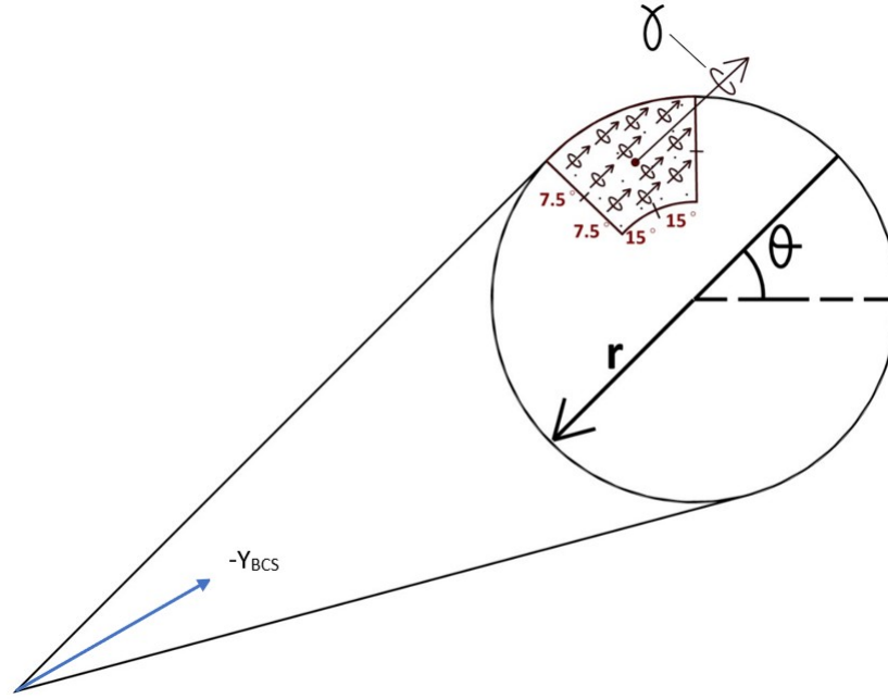
Figure 4.1. High fidelity segmented cone of freedom for -y -axis pointing to Sun vector
