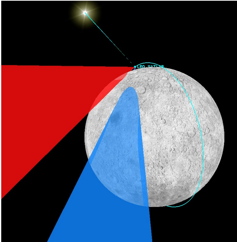
Figure 3.1. Simultaneous ST occultations represented as an access in STK (red FOR = ST1; blue FOR = ST2)
