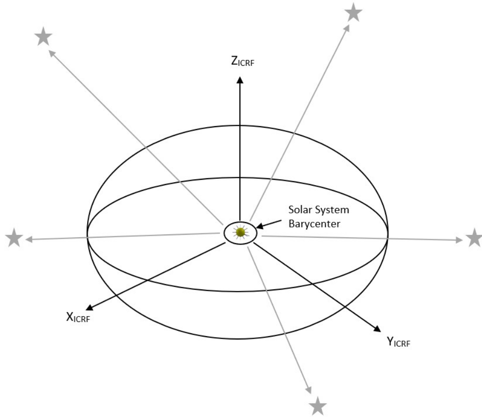
Figure 2.1. International Celestial Reference Frame. Adapted from [4].
