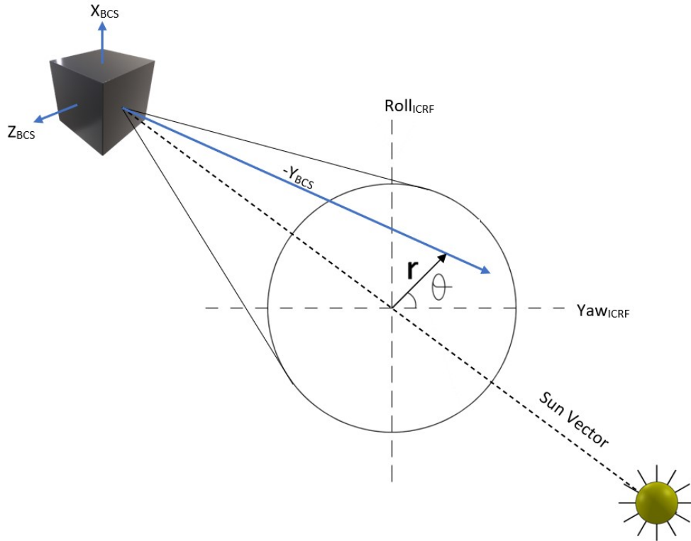
Figure 3.3. Relationship between polar coordinates, the BCS, and the Sun vector
