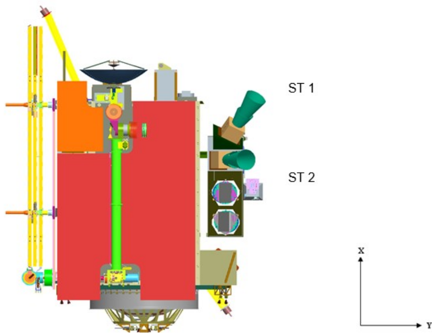
Figure 2.3. LRO ST locations. Source: [5].
