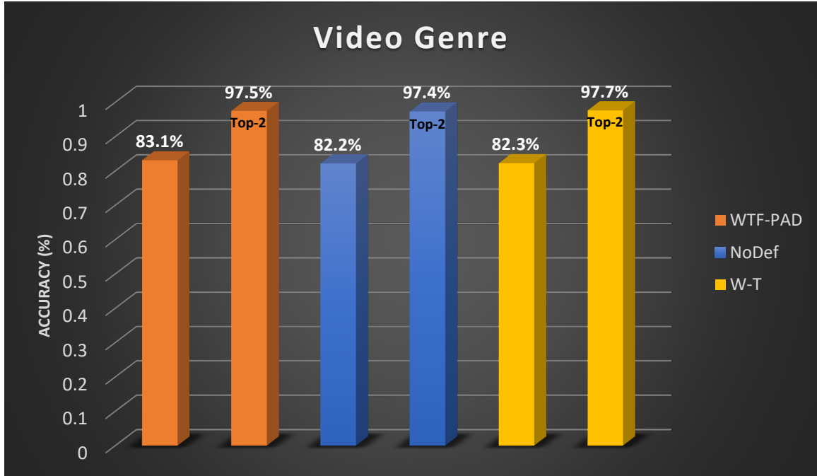
Figure 9. Attack accuracy on predicting YouTube video genre
