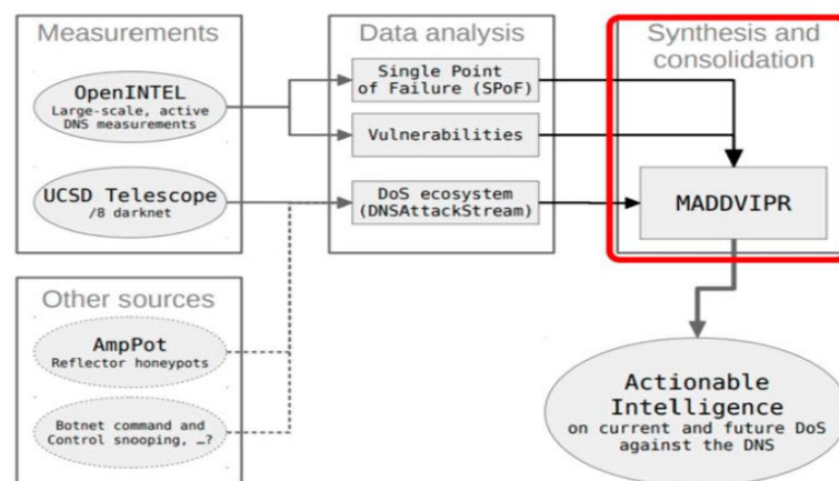
Figure 2. MADDVIPR Architecture
