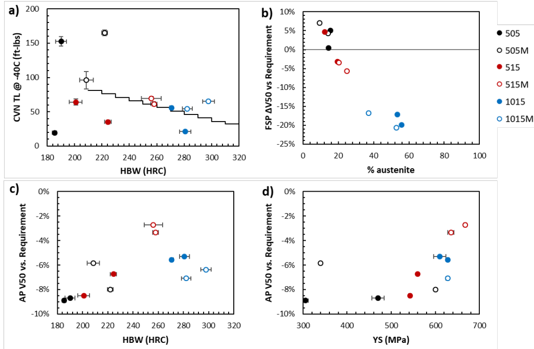
Fig. 18 Performance of Phase 3 alloys compared to MIL-DTL-12560K minimum requirements: a) CVN as a function of hardness, b) FSP performance vs. volume percent austenite, and AP performance as a function of c) hardness and d) yield strength
