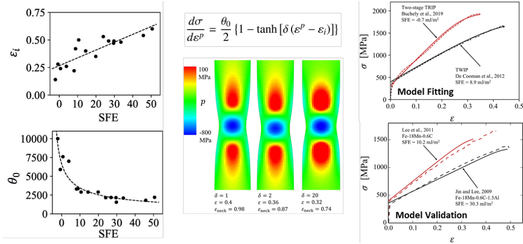
Fig. 7 Model relationship to predict hardening response \left(\frac{d\sigma}{d\varepsilon^p}\right) with parameters (\varepsilon_i \text{ and } \theta_0) demonstrated as a function of SFE along with model fitting and validations
