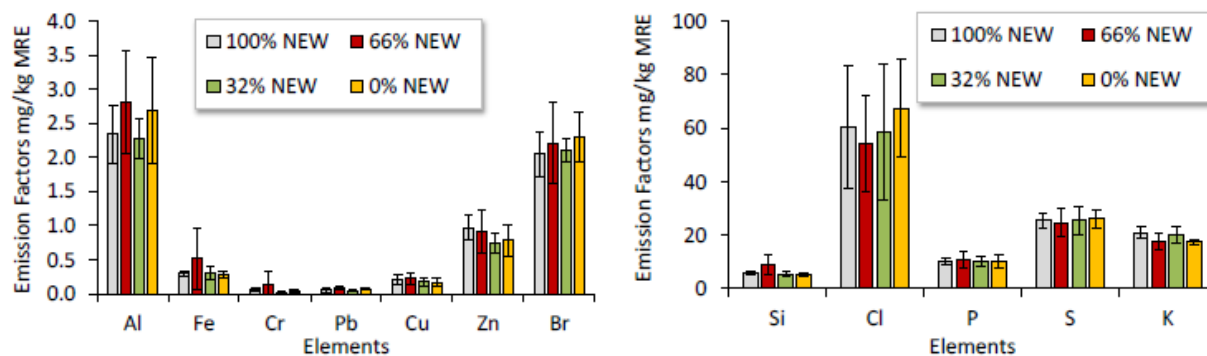
Figure 111. Major metal and trace /element emission factors from open burning of MREs
