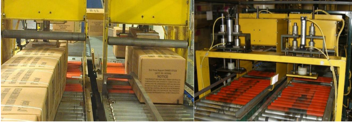
Figure 66. Case mixing equipment developed by AmeriQual Packaging (left) and a view of the front gate (right)
