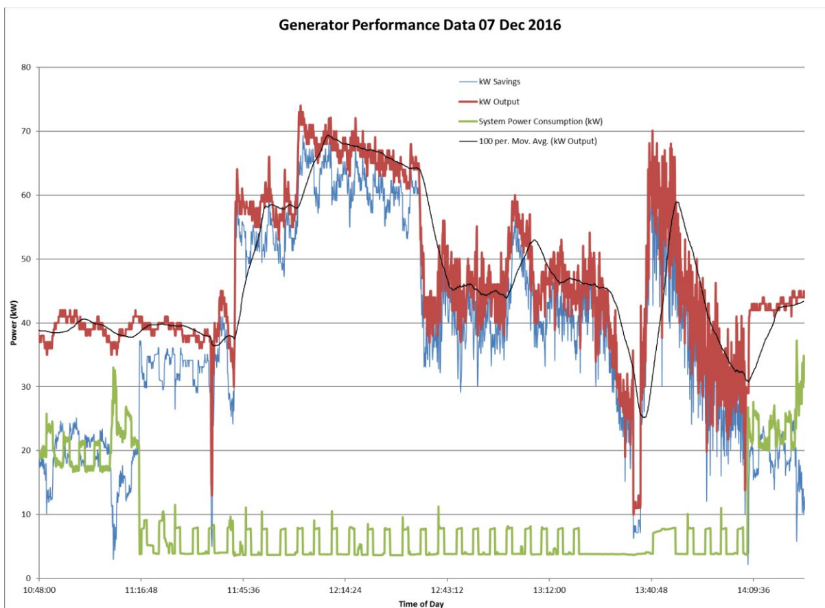
Figure 106. Generator performance data for the trial feedstock on 12/7/2016
