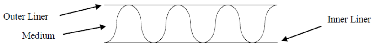
Figure 4. Combined board structure for corrugated fiberboard
