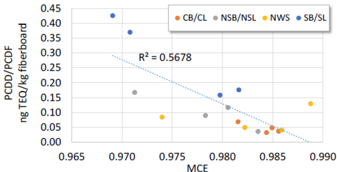
Figure 117. Fiberboard PCDD/PCDF emission factors versus modified combustion efficiency (MCE)
