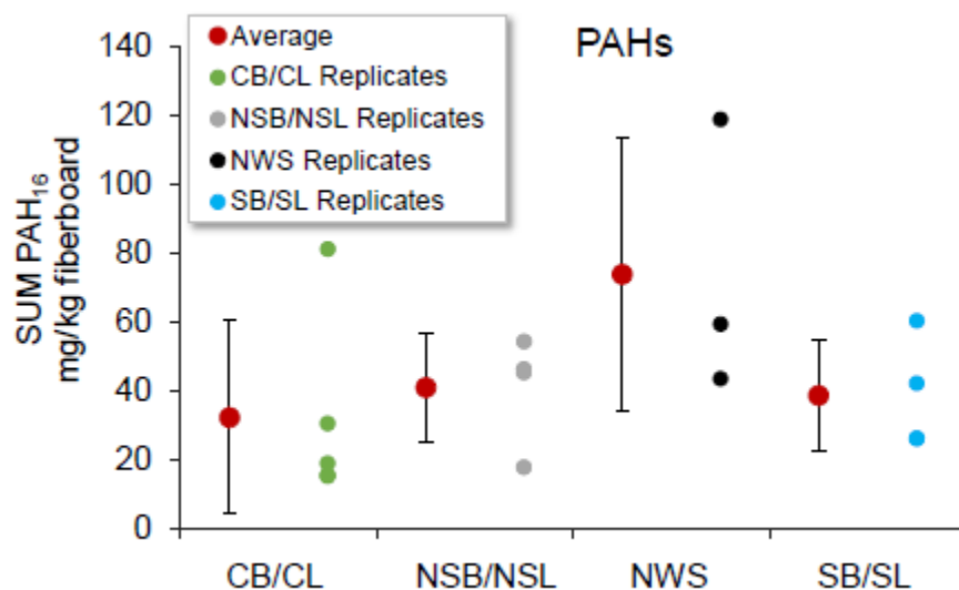
Figure 115. PAH emission factors from open burning of fiberboard packaging. Error bars represent 1 standard deviation.
