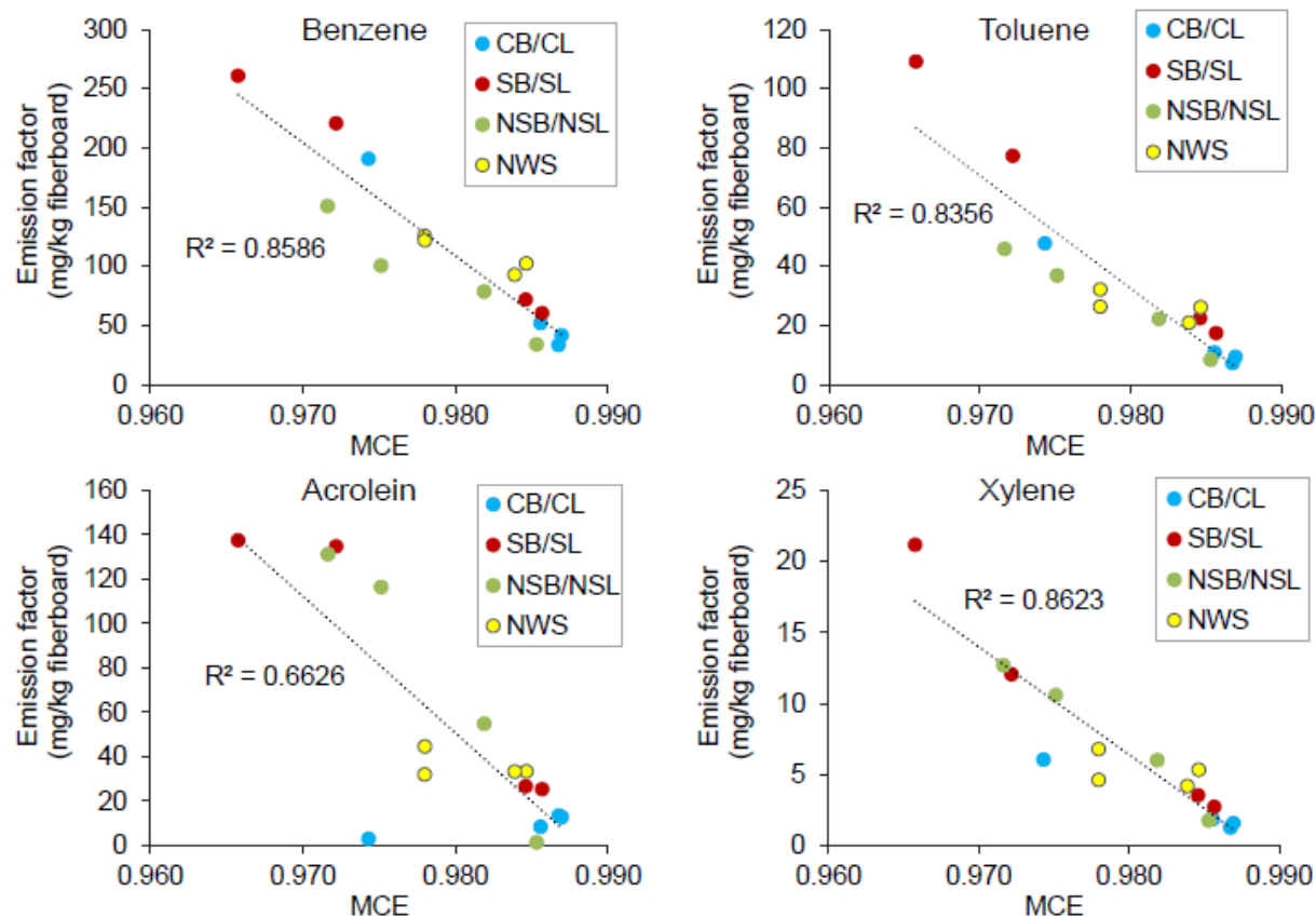
Figure 113. Select VOCs versus modified combustion efficiency (MCE)
