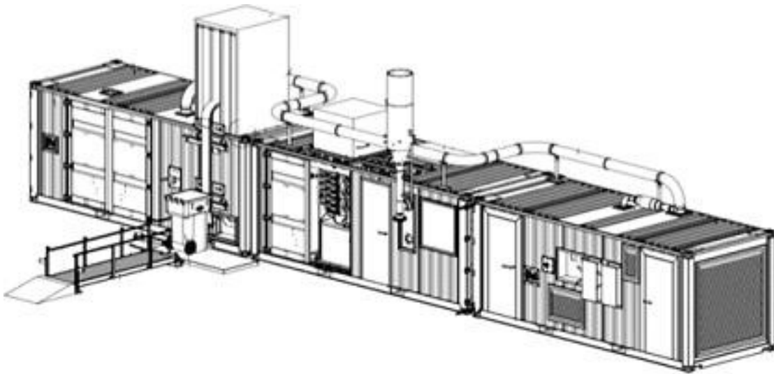
Figure 41. Full BWEC system design in the demonstration configuration (with optional cartfeeder system)
