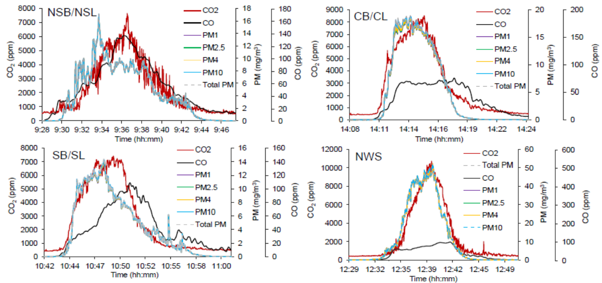
Figure 108. Typical traces of PM, CO, and CO 2 throughout each of the fiberboard type burns
