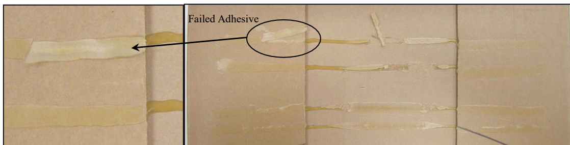
Figure 62. Adhesive application onto corrugated case (Note the failure of adhesive to bond to coated material)
