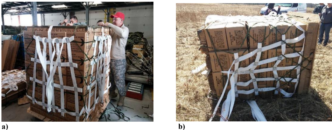
Figure 95. Rigging the corrugated pallets a) before and b) after
