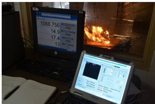
Figure 48. Monitoring of Continuous Emission Monitors (CEMs), SVOC flow rate, temperature, and canister pressure during a burn
