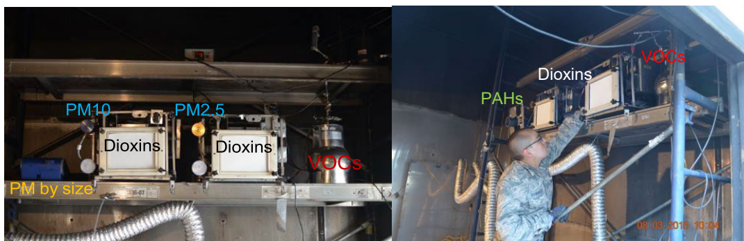
Figure 47. Flyer sampling instruments.
