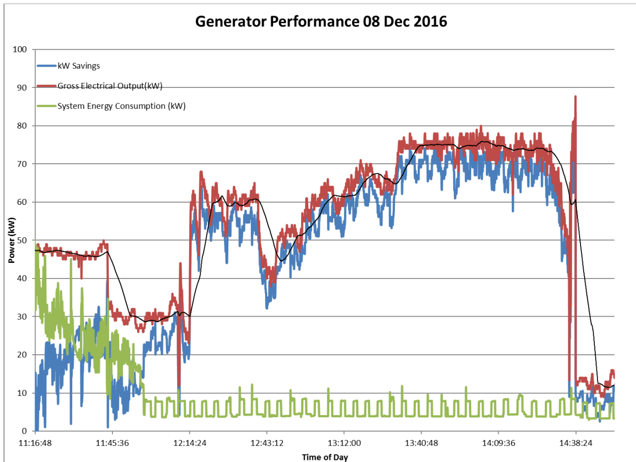
Figure 107. Generator performance data for the control feedstock on 12/8/2016
