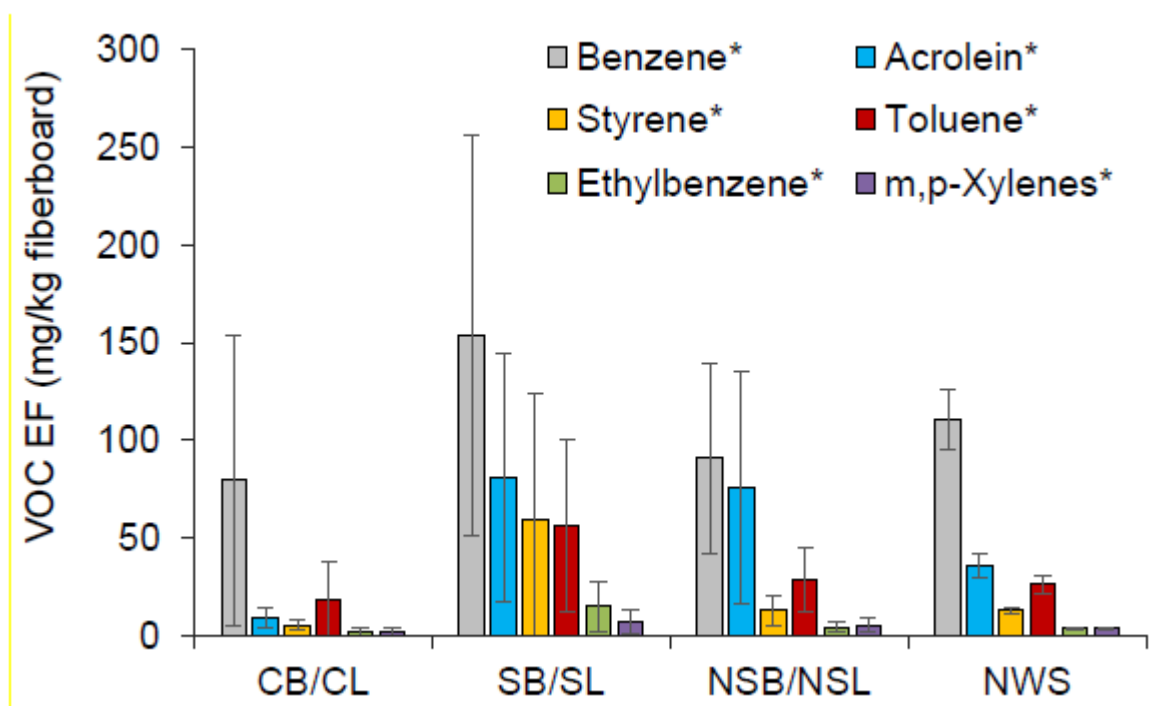
Figure 112. Select VOCs and their emission factors for the different fiberboard types. * = on EPA's list of hazardous air pollutants
