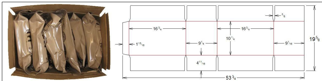
Figure 26. MRE Solid Fiberboard Case
