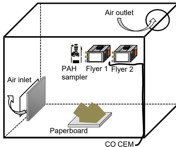
Figure 44. Schematic of open burn test facility. Not to scale
