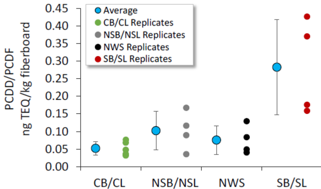
Figure 116. PCDD/PCDF emission factors from open burning of fiberboard packaging. Error bars represent 1 standard deviation
