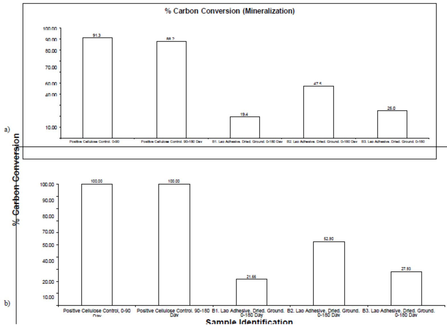
Figure 93. ASTM D5338 – 180-Day Compost Exposure a) before and b) after normalization to cellulose.
