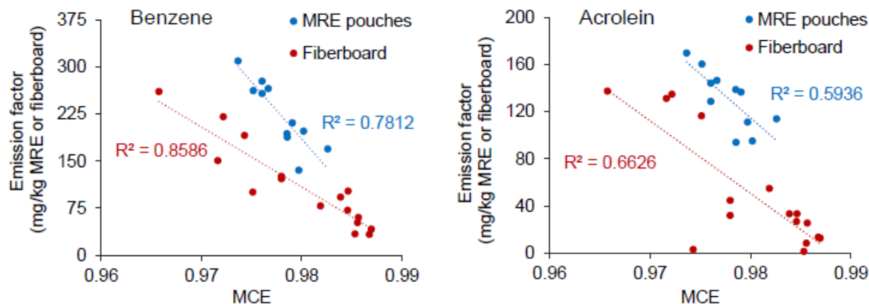
Figure 114. Benzene and acrolein vs. MCE for all MRE waste compositions and fiberboard type burns
