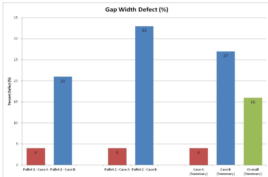
Figure 128. Percent defect based on excessive gap width (cases with 0.75 inch or greater gap between the major flaps are failed)
