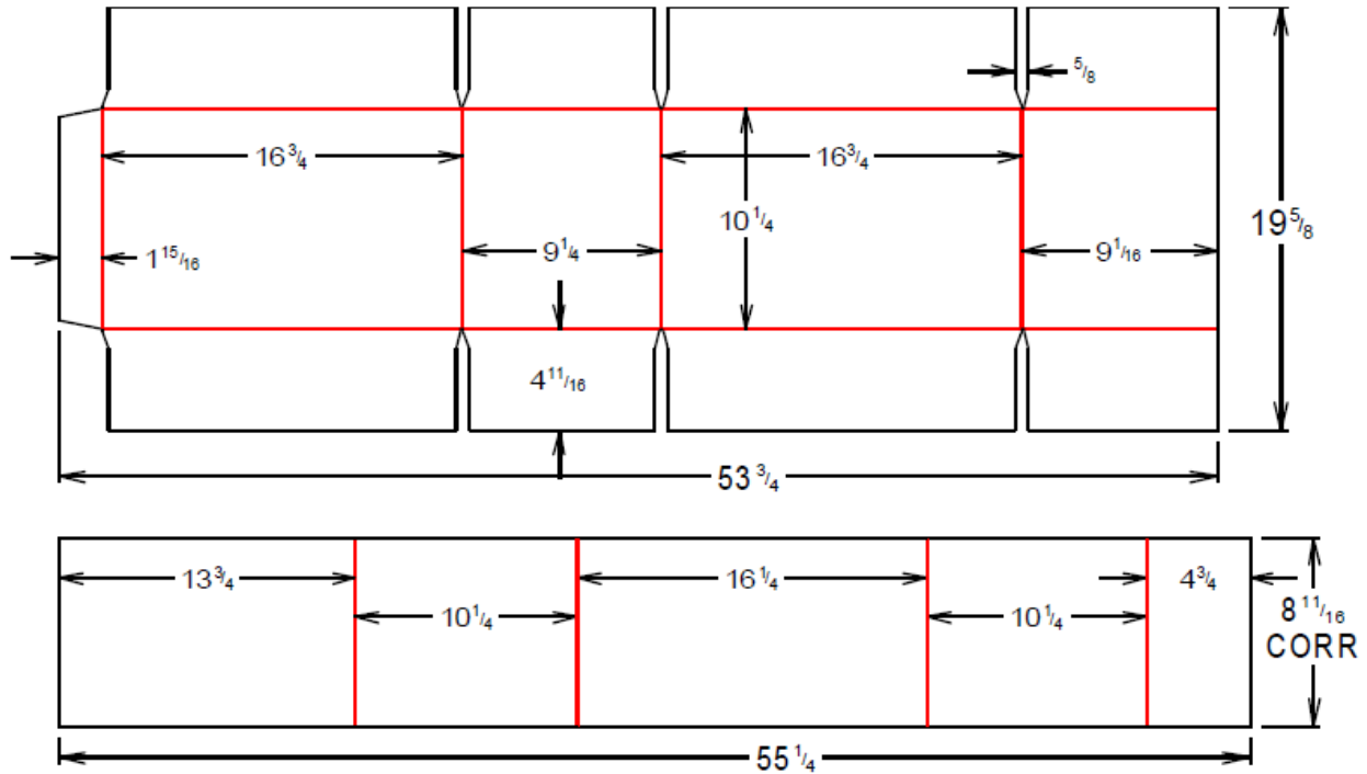
Figure 3. MRE solid fiberboard case (corrugated insert (bottom))
