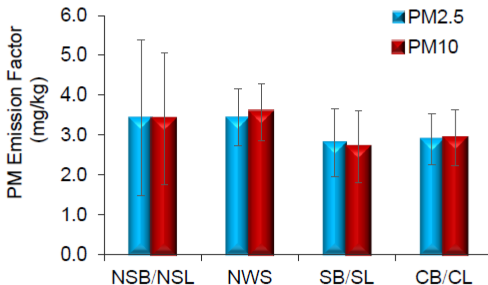
Figure 110. PM 2.5 and PM 10 emission factors from open burning of fiberboard. Error bars represent 1 STDV
