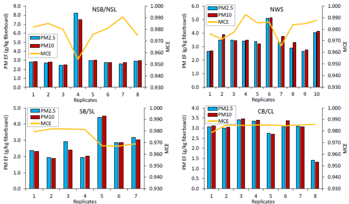
Figure 109. PM 2.5 and PM 10 emission factors and modified combustion efficiency (MCE) for each replicate
