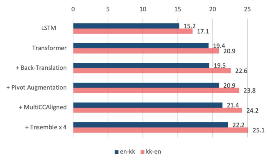
Figure 20. BLEU Scores on English↔Kazakh ANALYSIS Test Set.
