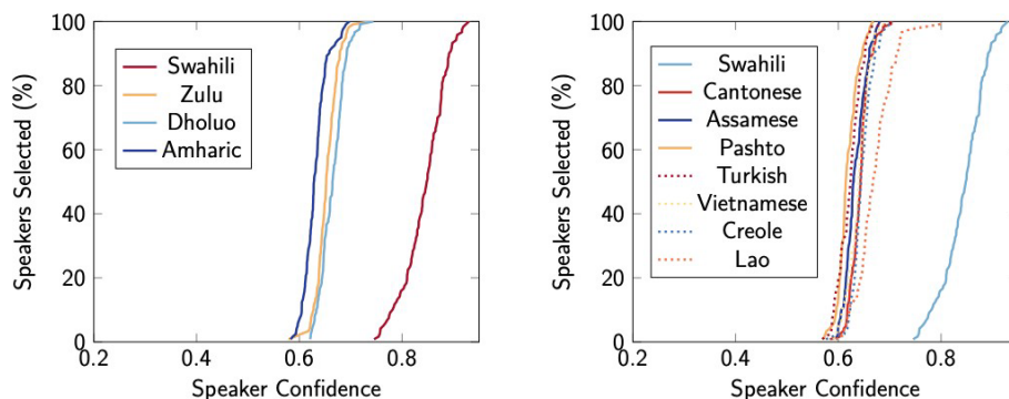
Figure 18. Confidence-Based Language Verification for Swahili: Percentage of Documents (Speakers) below a Confidence Threshold.
