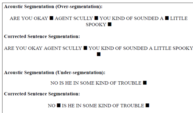
Figure 14. Example Acoustic Segmentation Errors and their Corrections.
