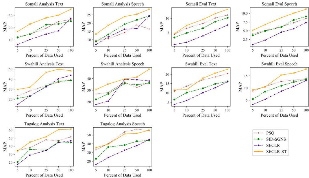
Figure 24. Ablation Study Results of SECLR and SECLR-RT Model Performances as a Function of Sub-Sampling Percentages. X-Coordinate uses the Log Scale.
