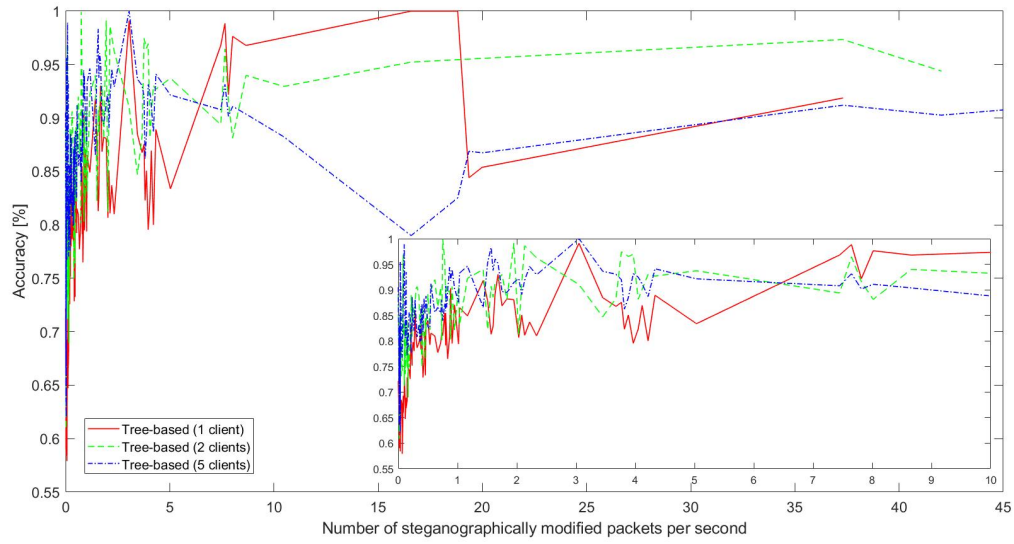
Figure 12: Accuracy of the detection depending on the number of the steganographically modified packets ('Tree-based' method).
