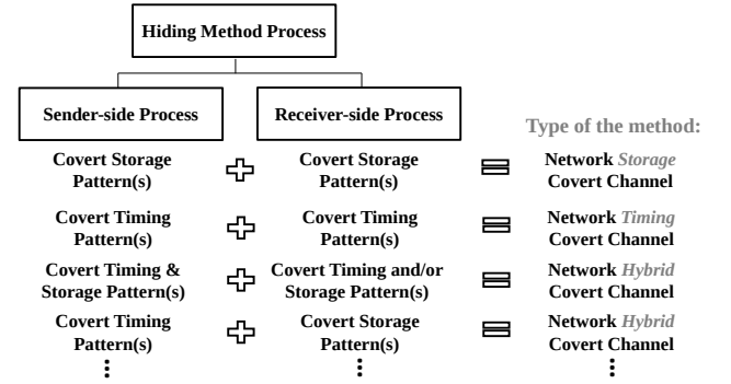
Figure 3: Improved aspects of the existing pattern-based taxonomy.
