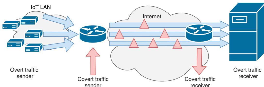
Figure 5: Assumed threat model, i.e. DNCC in the IoT environment.
