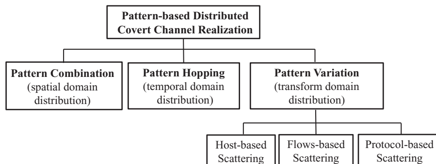
Figure 1: Classification of pattern-based distributed network covert channel realization [24].
