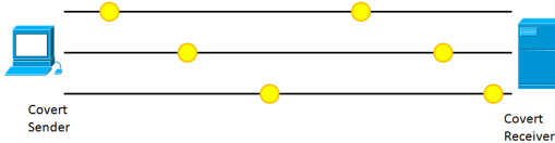
Figure 2: Multi-flow distribution for realizing a single (distributed) network covert channel.
