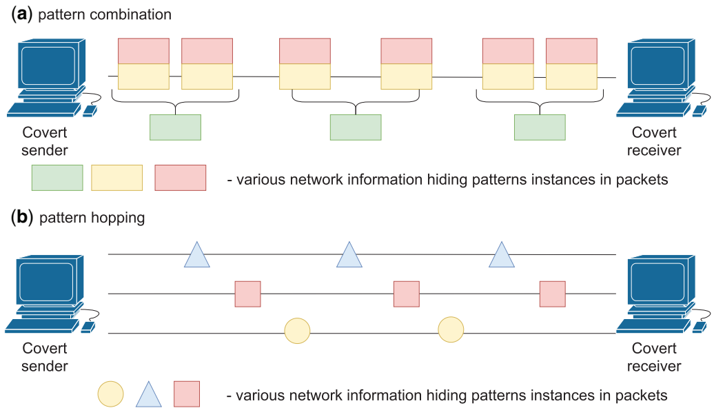
Figure 2: Illustration of the (a) pattern combination and (b) pattern hopping concepts.
