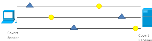
Figure 3: Multi-flow pattern hopping for realizing a single (distributed) network covert channel.
