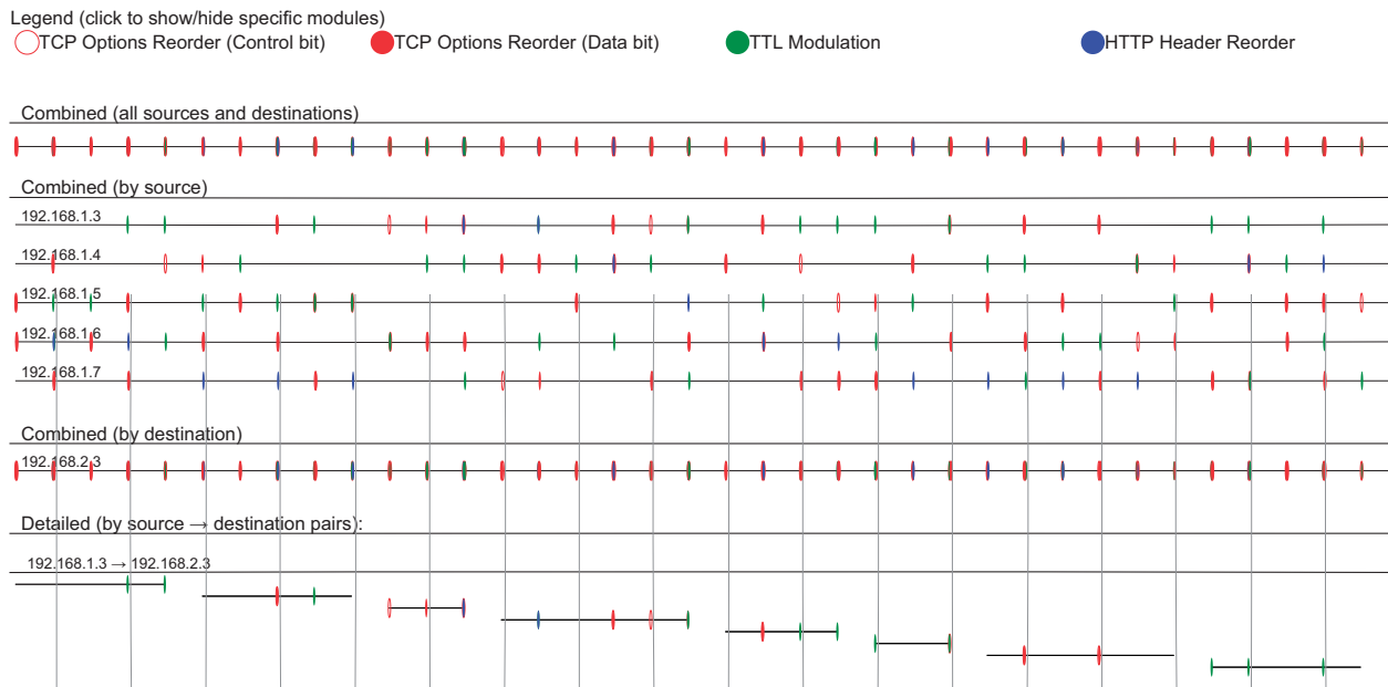
Figure 7: Automatically generated plot presenting particular packet modifications in connections used by DNCC (included in the dataset).
