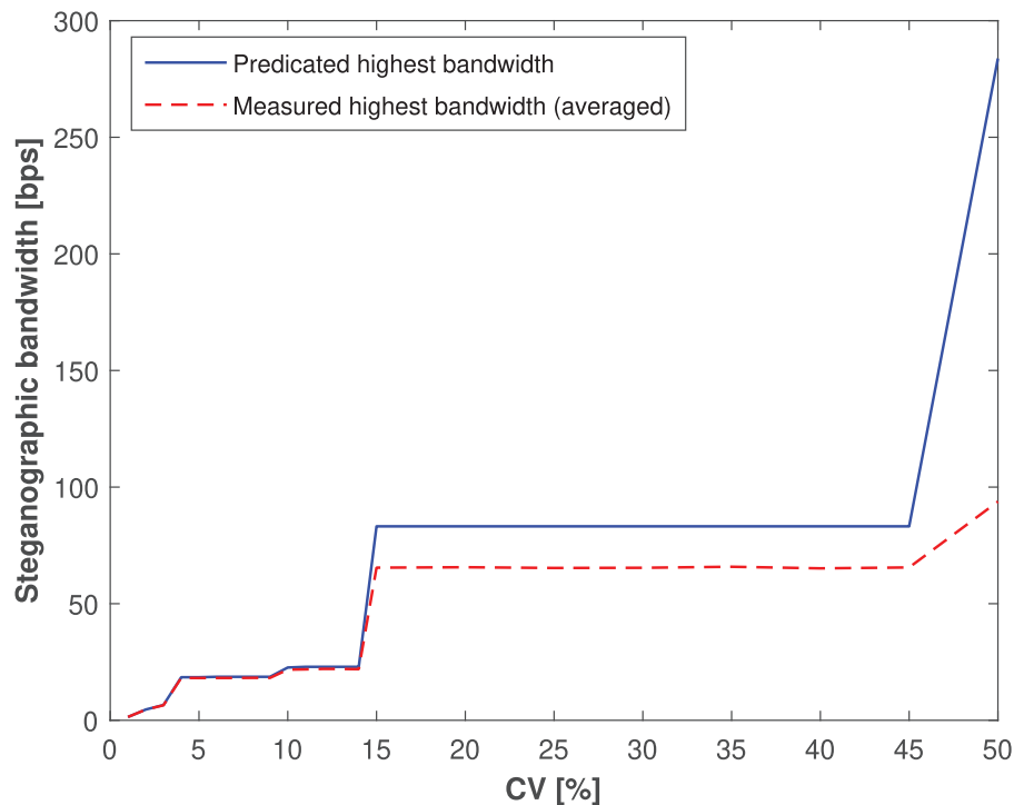
Figure 9: Predicted and measured covert data rate depending on the CV value.
