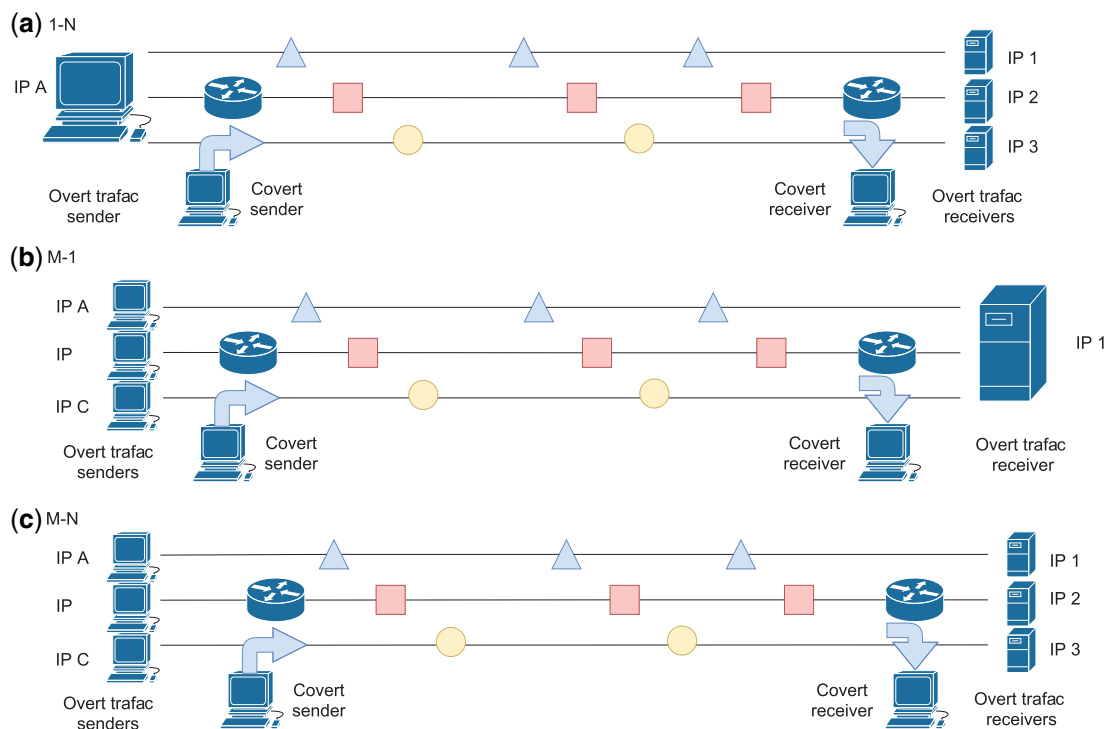
Figure 4: Comparison of the enhanced DNCC scenario: (a) one-to-many (1: N), (b) many-to-one (M: 1) and (c) many-to-many (M: N).
