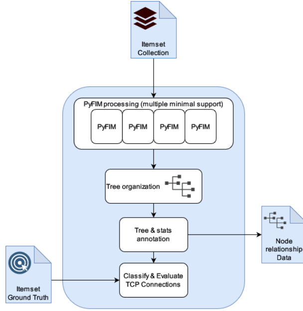
Figure 4: Tree-based approach pipeline: the individual item sets are grouped by the Frequent Itemsets algorithm and this grouping is performed in multiple attempts with different minimal support parameter.
