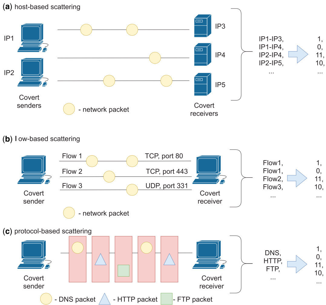
Figure 3: Illustration of the pattern variation techniques (a) host-based scattering, (b) flow-based scattering and (c) protocol-based scattering.
