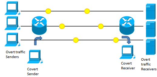
Figure 4: Injection of secret bits into the data streams of various overt traffic senders.
