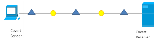
Figure 1: Pattern hopping – the simplest enhancement to the information hiding patterns i.e. various patterns used within one connection (defined in [3])
