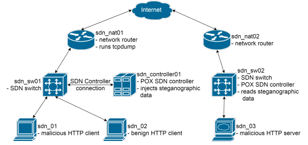
Figure 7: Experimental test-bed.
