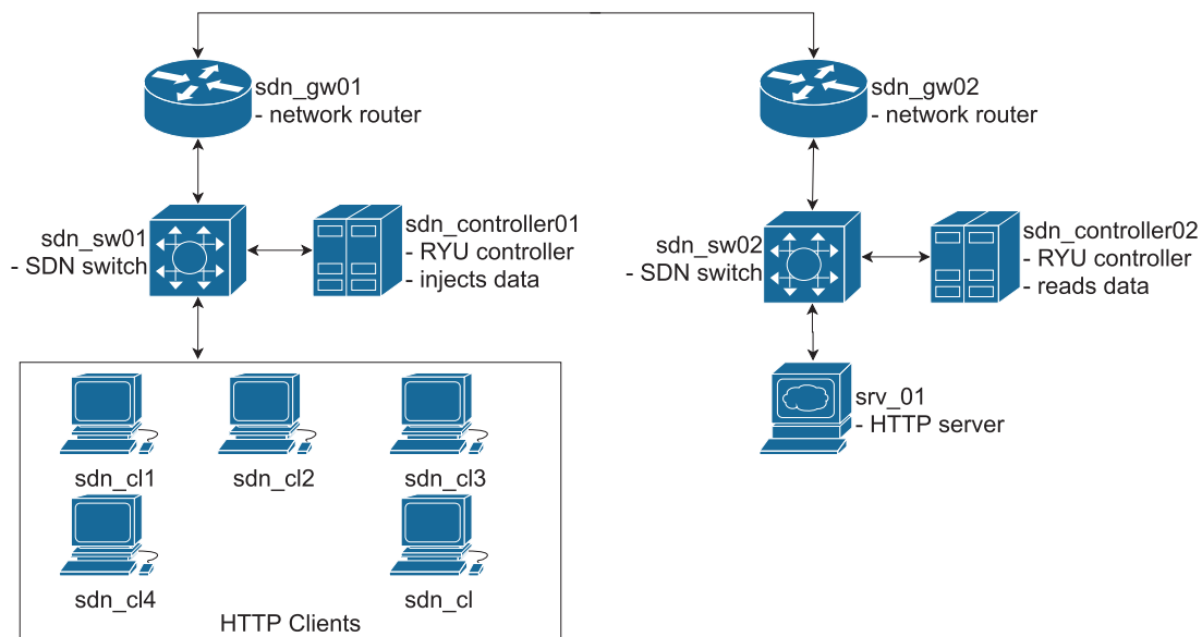
Figure 6: Utilized experimental testbed.
