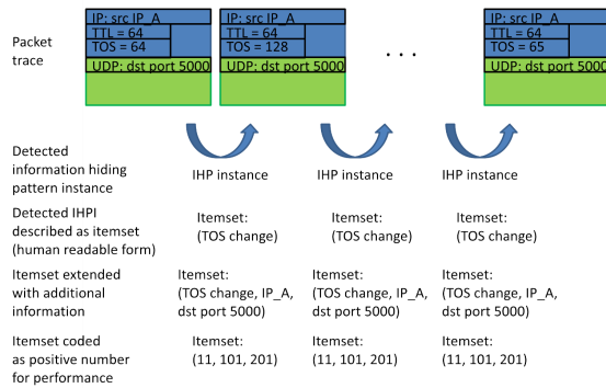
Figure 5: Exemplary packets' trace for the ToS-based covert channel and the steps of pre-processing from the detection of IHPI to the coded item sets.
