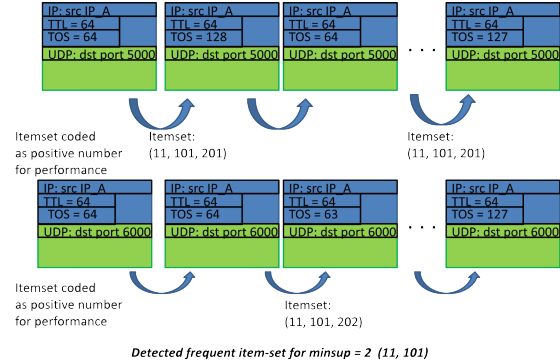
Figure 6: Distributed covert channel realization using two independent streams (multi-stream transmission), coded item sets associated with IHPIs and detected frequent item set.
