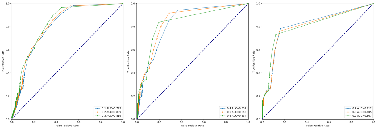
Figure 9: ROC plots for the Tree-based detection method for various ratios of suspicious children in the tree.
