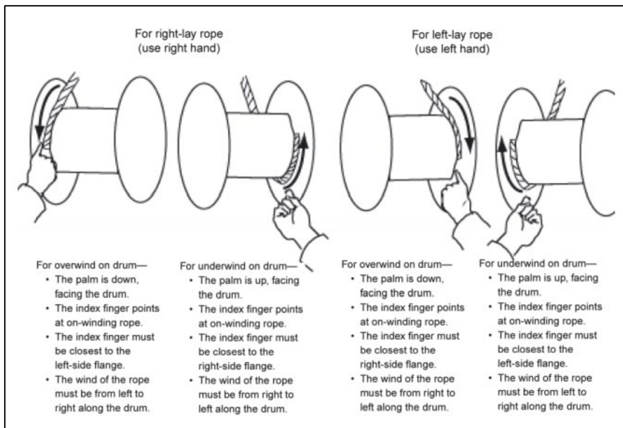
Figure 2. Determining starting flange of wire cable, reproduced from TM 3-34.86, Rigging Techniques, Procedures, and Applications.
