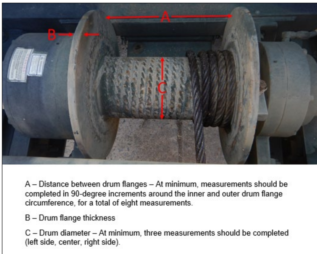
Figure 1. Winch measurement locations and recommended minimum number of measurements.
