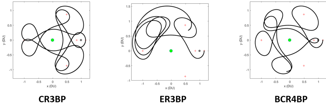
Figure 30: Propagation of Cislunar Periodic Orbit 9 via all Dynamical Models
