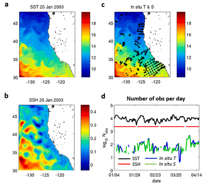
Fig. 1. The ROMS-CCS configuration used in the EAKF and 4D-Var experiments. The SST and SSH on a date close to the start of each experiment are shown in (a) and (b), respectively. The locations of all in situ hydrographic observations collected during the Jan–April 2003 period are shown in (c), and time series of \log_{10} of the number of observations of each type available during each 24-hour period are shown in (d). Here and throughout the paper, units are as follows: temperature (deg C), SSH (m), and salinity (nondimensional).
