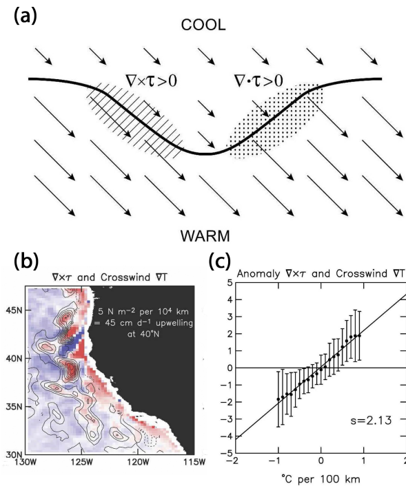
Figure 1: (a) A schematic representation of the influence of an SST front on wind stress. Regions of enhanced wind stress curl ( \nabla \times \tau ) and wind stress divergence ( \nabla \cdot \tau ) are indicated in relation to the orientation of the wind direction
