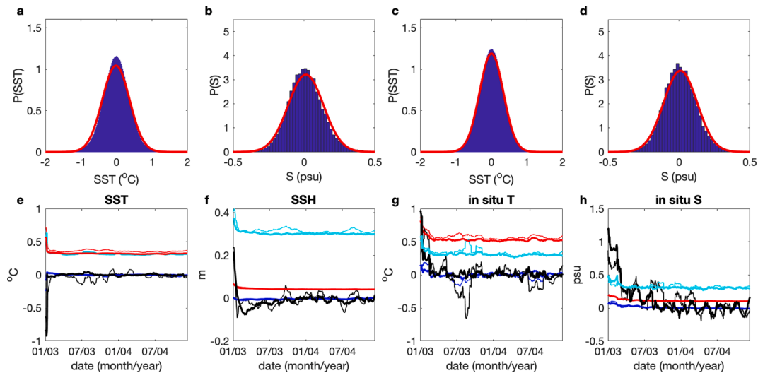
Fig. 13. Probability density functions (pdfs) of the Jan 2003–Dec 2004 innovations in (a) 4D-Var SST, (b) 4D-Var in situ S, (c) EAKF SST and (d) EAKF in situ S. The red line shows the pdf for a normal distribution with the same mean and standard variation. Time series of the first four moments of the innovation pdfs computed over a 15-day moving window for the EAKF (thick lines) and 4D-Var (thin lines) for (e) SST, (f) SSH, (g) in situ T and (h) in situ S. The pdf mean is shown in blue, the standard deviation in red, the skewness in black and the kurtosis scaled by a factor of 0.1 in cyan. (For interpretation of the references to color in this figure legend, the reader is referred to the web version of this article.)
