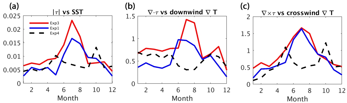
Figure 5: Time series of the regression coefficients ( aka coupling strength ) between (a) SST and wind stress magnitude, (b) the downwind SST gradient and \nabla \cdot \tau , and (c) the crosswind SST gradient and \nabla \times \tau . Regression coefficients are computed from the spatially high-pass filtered fields, and in all cases wind stress was computed by accounting for the relative motion of the ocean and atmosphere. Results are shown for Exp1 (blue line), Exp3 (red line), and Exp4 (black dashed line). For comparison with Fig. 1c, the units of the regression coefficients are based on SST in ^{\circ}\text{C} , SST gradients in ^{\circ}\text{C} per 100 km, and wind stress divergence/curl in \text{N m}^{-2} per 10^4 km.
