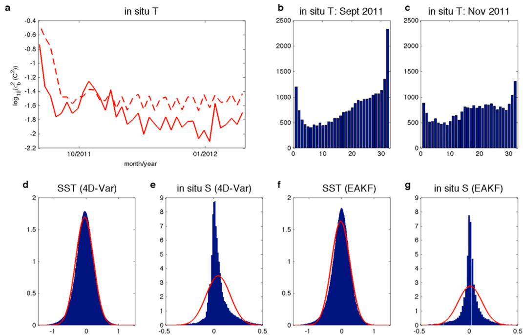
Fig. 22. Diagnostics of 4D-Var and EAKF analyses for ROMS-IO. (a) Time series of \log_{10}(\sigma_b^2) (solid red line) and \log_{10}(\text{Tr}(\Sigma_c)/N) (red dashed line) for in situ temperature observations in the 4D-Var analysis. (b) and (c) Rank histograms in the EAKF analysis based on all the in situ temperature observations during Sep and Nov. (d)–(g) Probability density functions (pdfs) of the Sep 2011–Jan 2012 innovations in (d) 4D-Var SST, (e) 4D-Var in situ S, (f) EAKF SST and (g) EAKF in situ S. (For interpretation of the references to color in this figure legend, the reader is referred to the web version of this article.)
