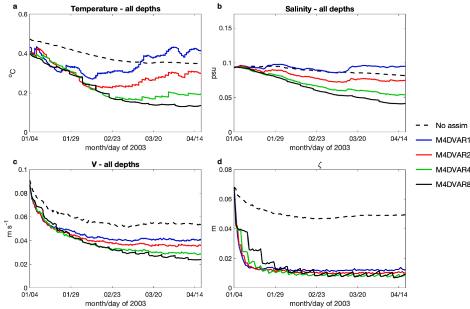
Fig. 8. Time series of the RMS error in (a) temperature, (b) salinity, (c) meridional velocity and (d) SSH for experiments using 1-day (blue line), 2-day (red line), 4-day (green line) and 8-day (black line) data assimilation windows. Also shown is the case where no data were assimilated (black dashed line). (For interpretation of the references to color in this figure legend, the reader is referred to the web version of this article.)
