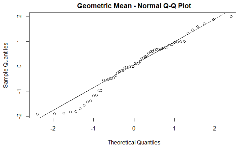
Figure 24. Case Study A, Experiment I: Geometric Mean Normality Plot
