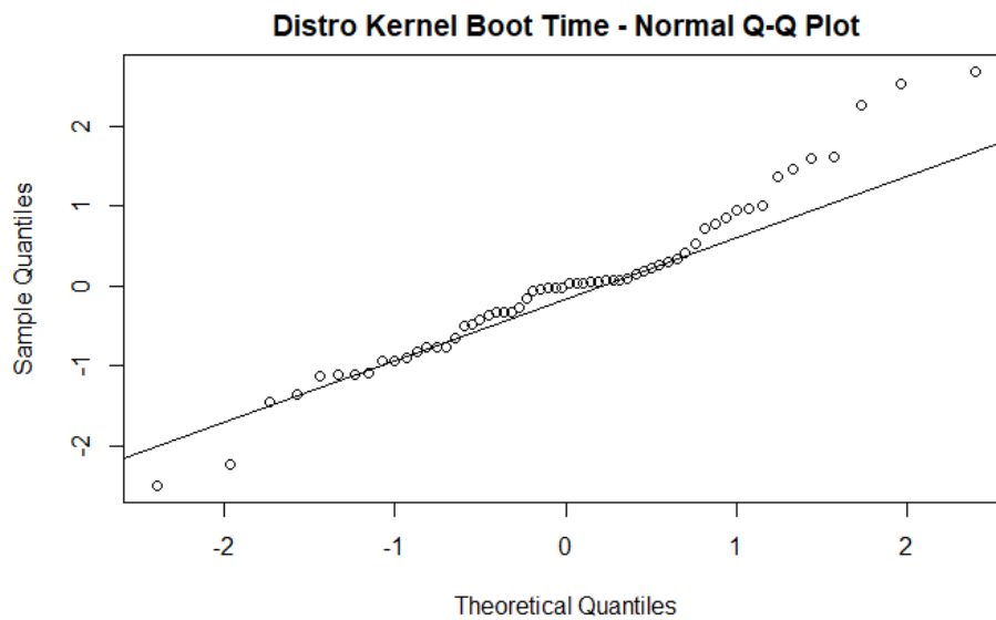
Figure 29. Case Study B, Experiment II: Distro Kernel Boot Time Normality Plot
