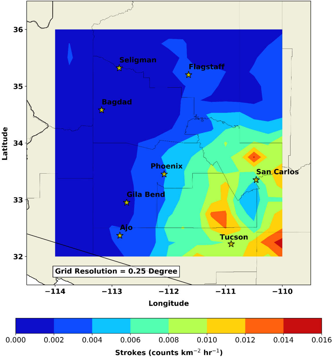
Figure 26. Arizona CP Forecast August 2019.
