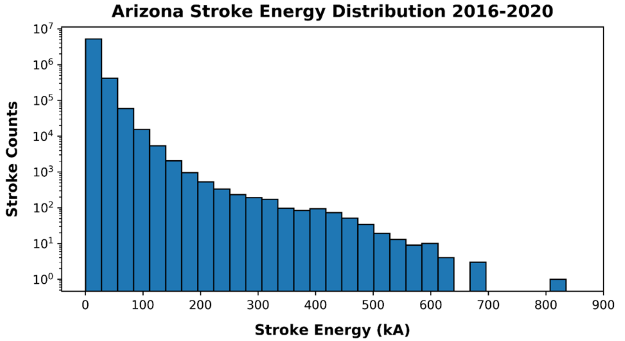
Figure 6. Arizona Stroke Energy Distribution 2016-2020.
