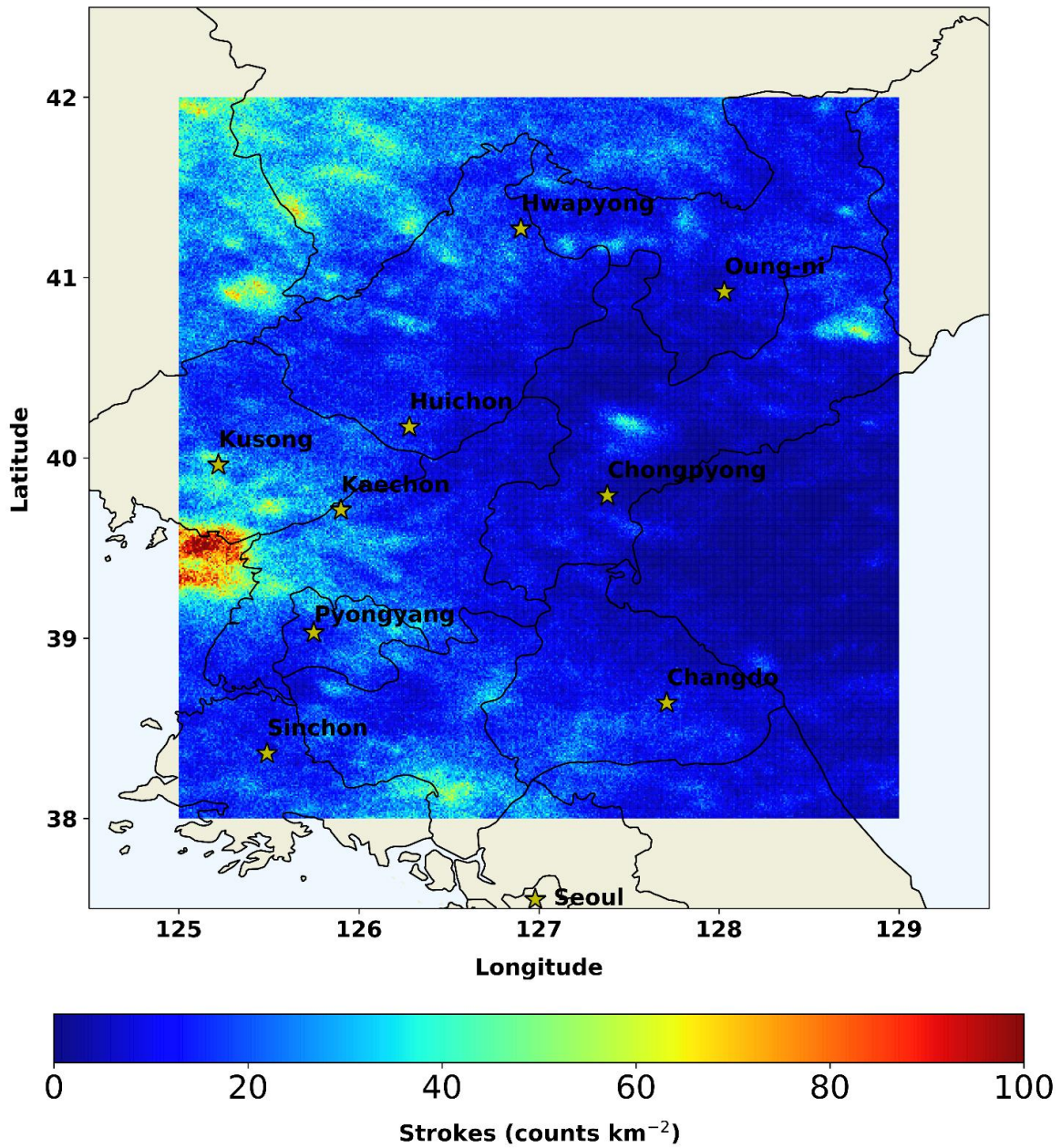
Figure 12. North Korea Stroke Density 2016-2020.
