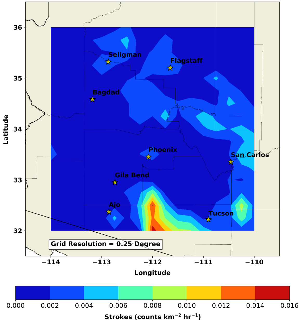
Figure 25. Arizona Observed Strokes August 2019.
