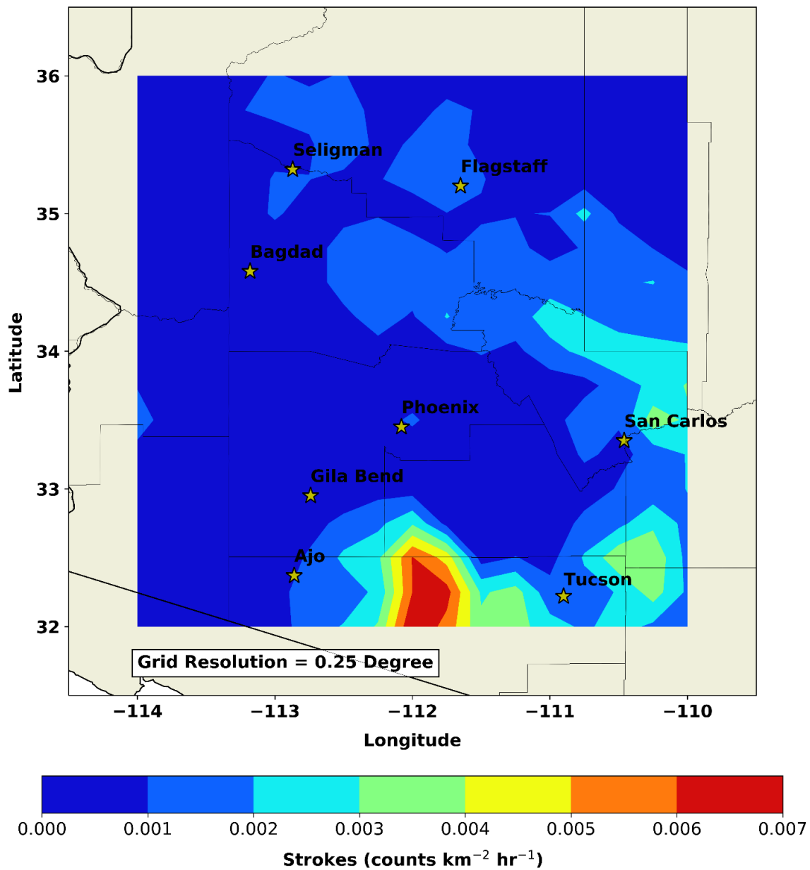
Figure 28. Arizona Observed Strokes JJA 2019.
