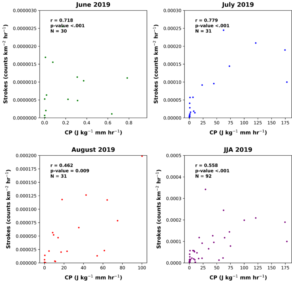
Figure 16. Arizona CP to Stroke Correlation: June 2019 (top left), July 2019 (top right), August 2019 (bottom left), JJA 2019 (bottom right).
