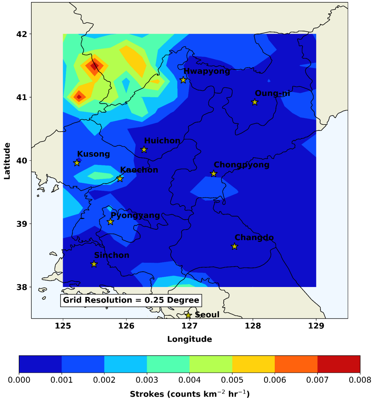
Figure 52. North Korea Observed Strokes JJA 2019.
