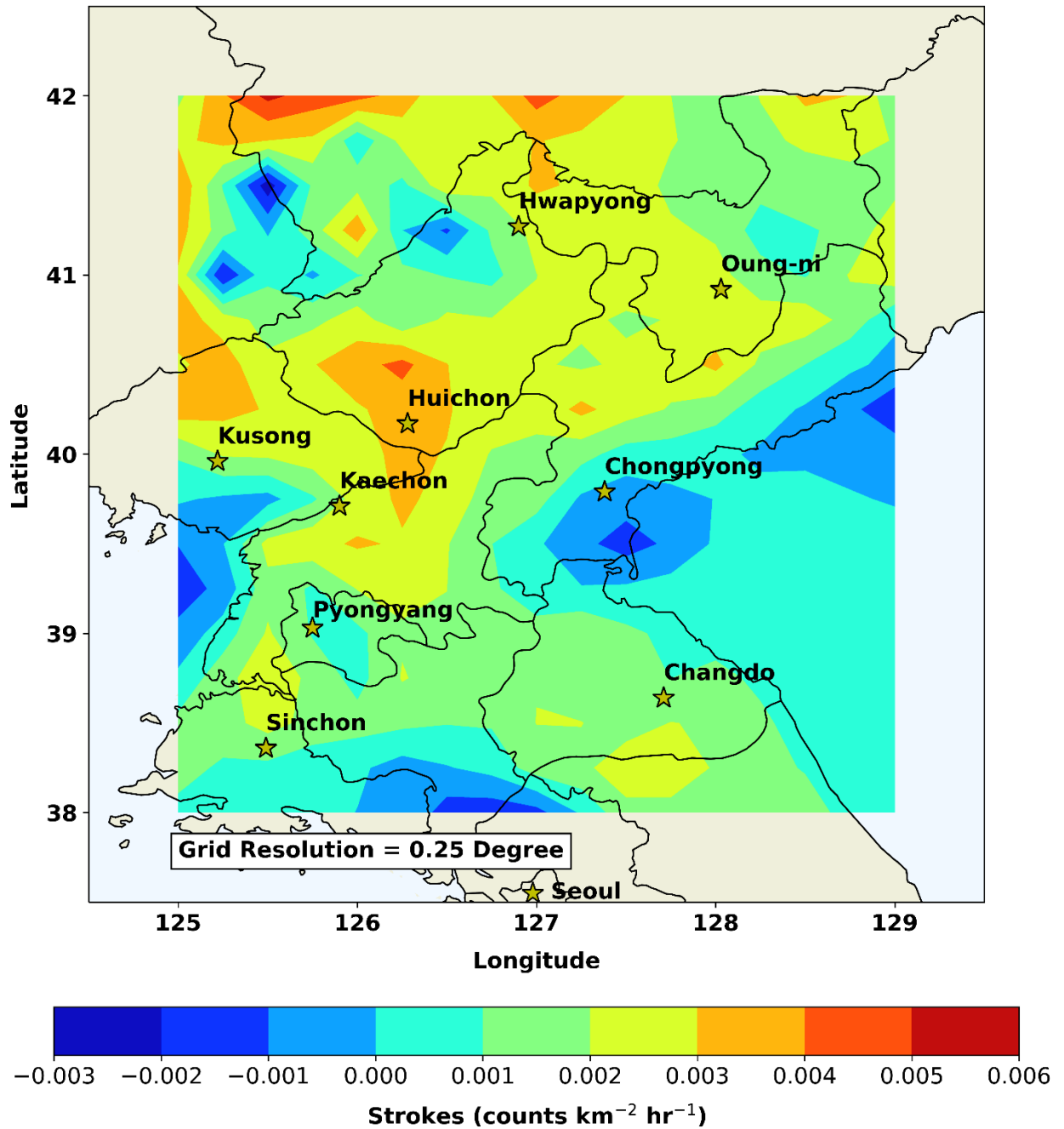
Figure 54. North Korea CP Difference (Forecast – Observed) JJA 2019.
