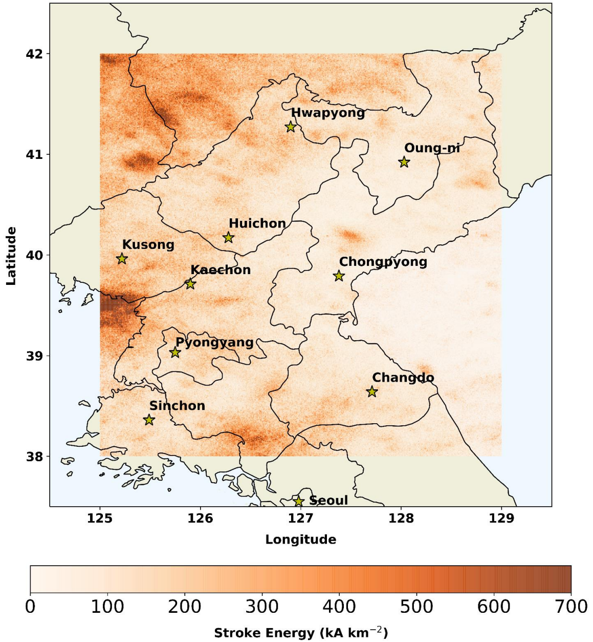
Figure 13. North Korea Stroke Energy 2016-2020.
