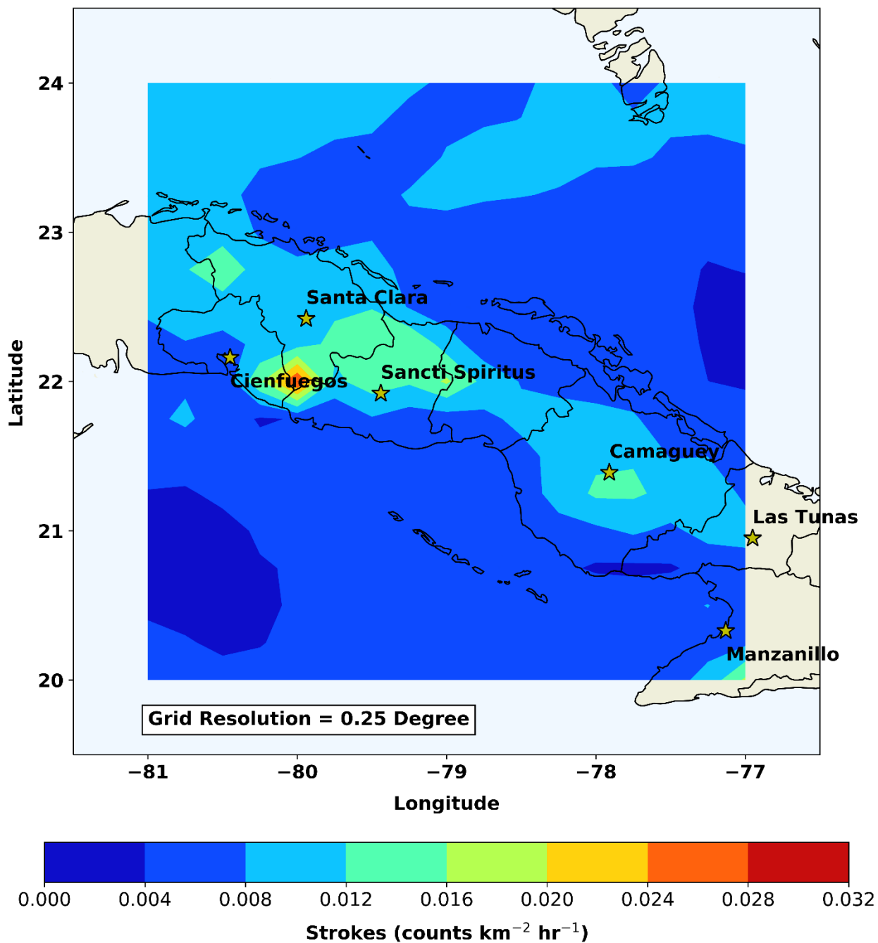
Figure 32. Cuba CP Forecast June 2019.
