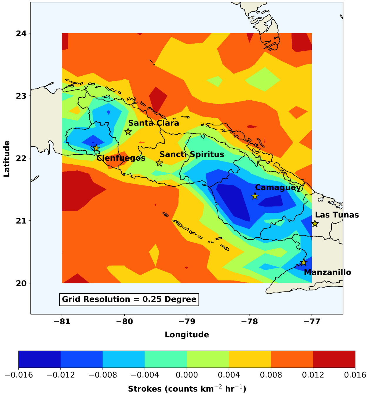
Figure 42. Cuba CP Difference (Forecast – Observed) JJA 2019.
