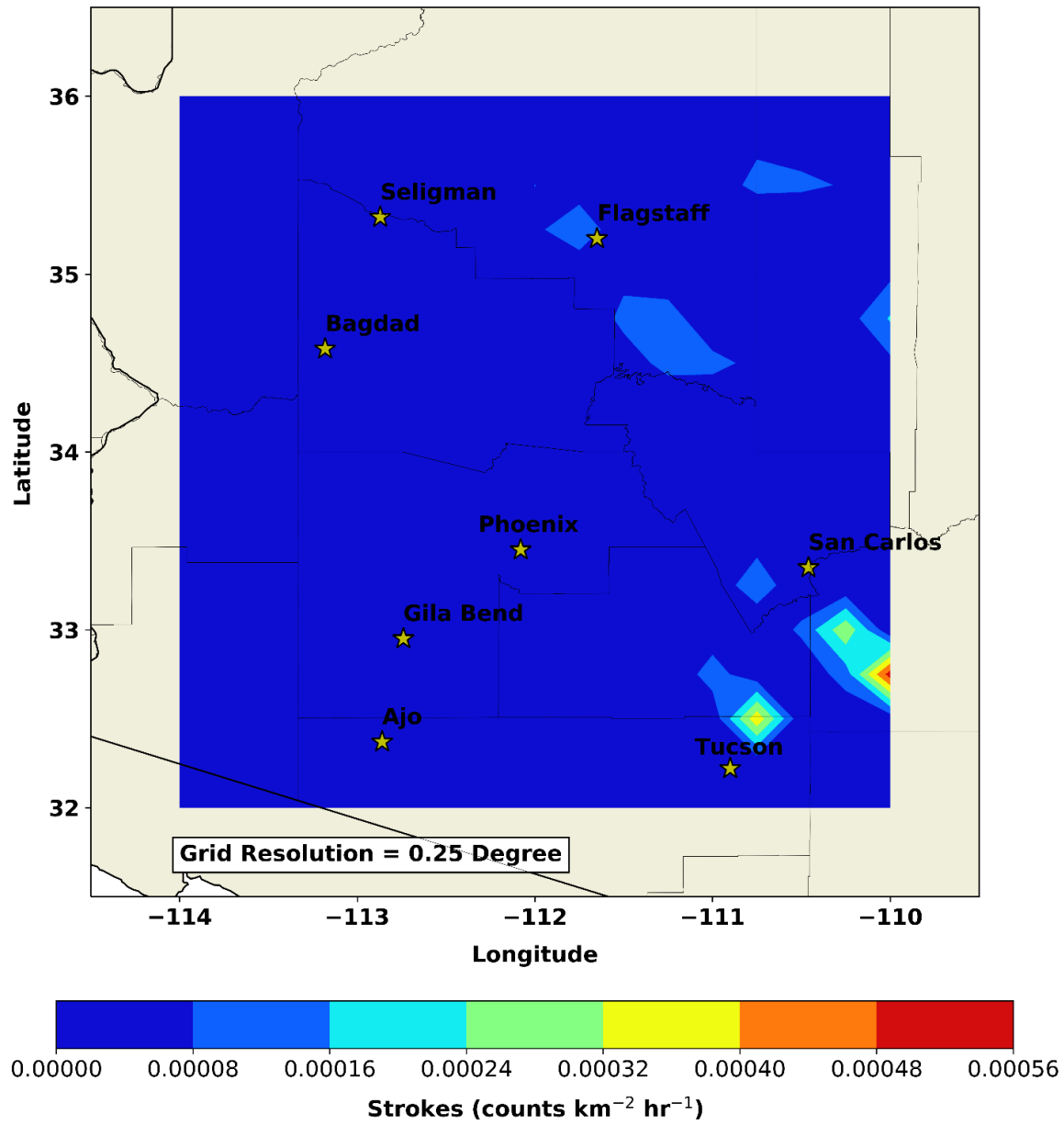
Figure 20. Arizona CP Forecast June 2019.
