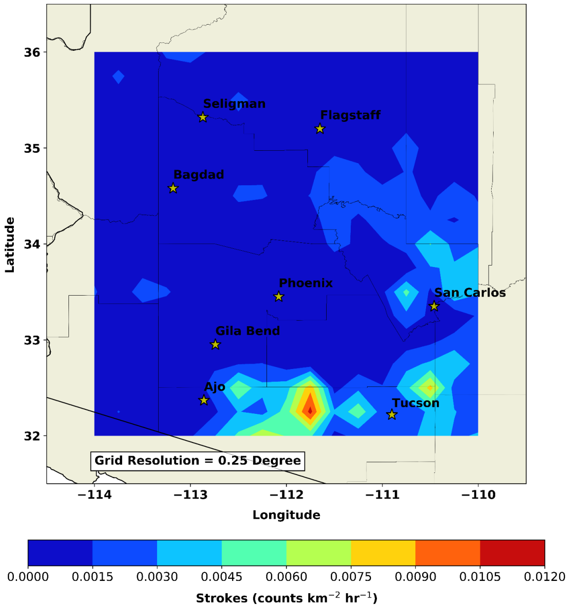
Figure 22. Arizona Observed Strokes July 2019.
