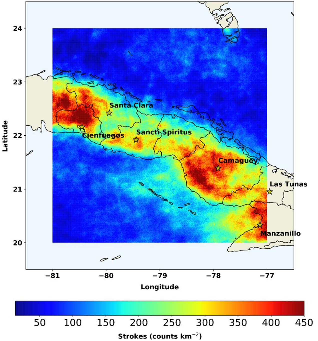
Figure 8. Cuba Stroke Density 2016-2020.
