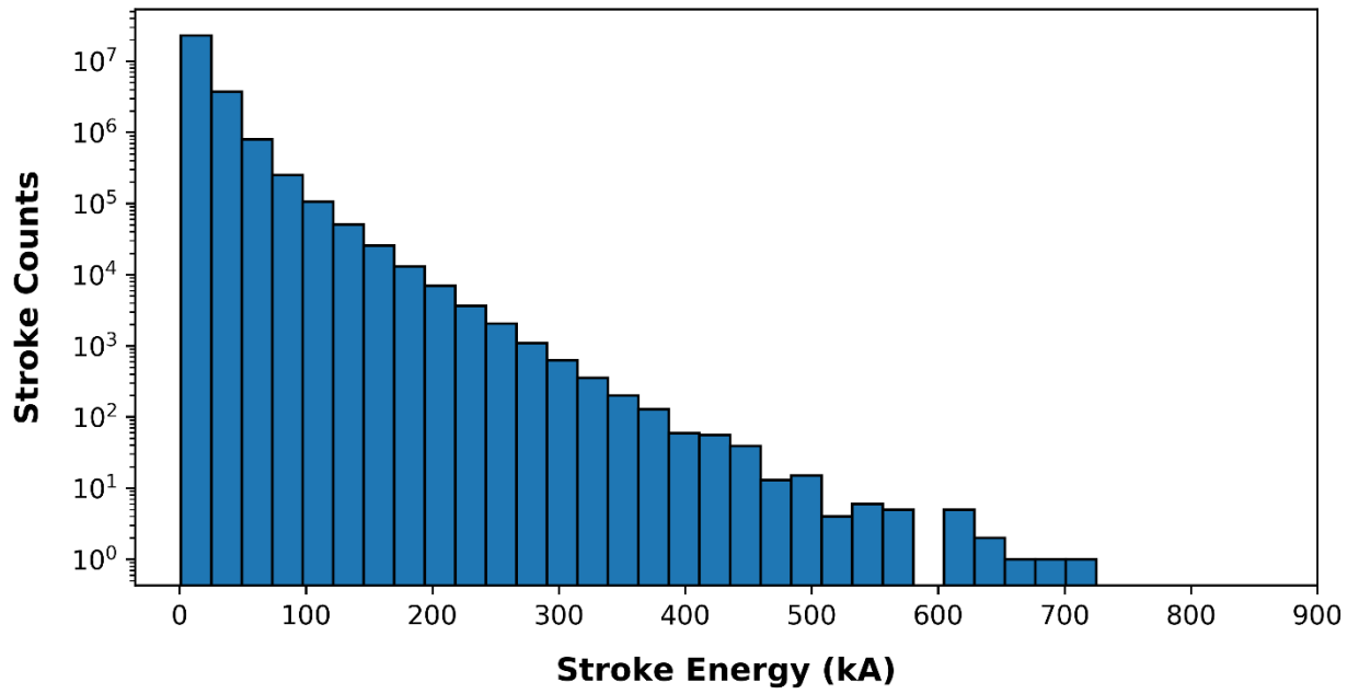
Figure 10. Cuba Stroke Energy Distribution 2016-2020.
