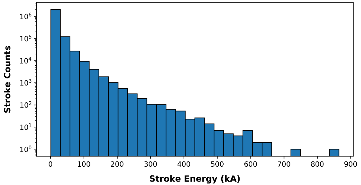
Figure 14. North Korea Stroke Energy Distribution 2016-2020.
