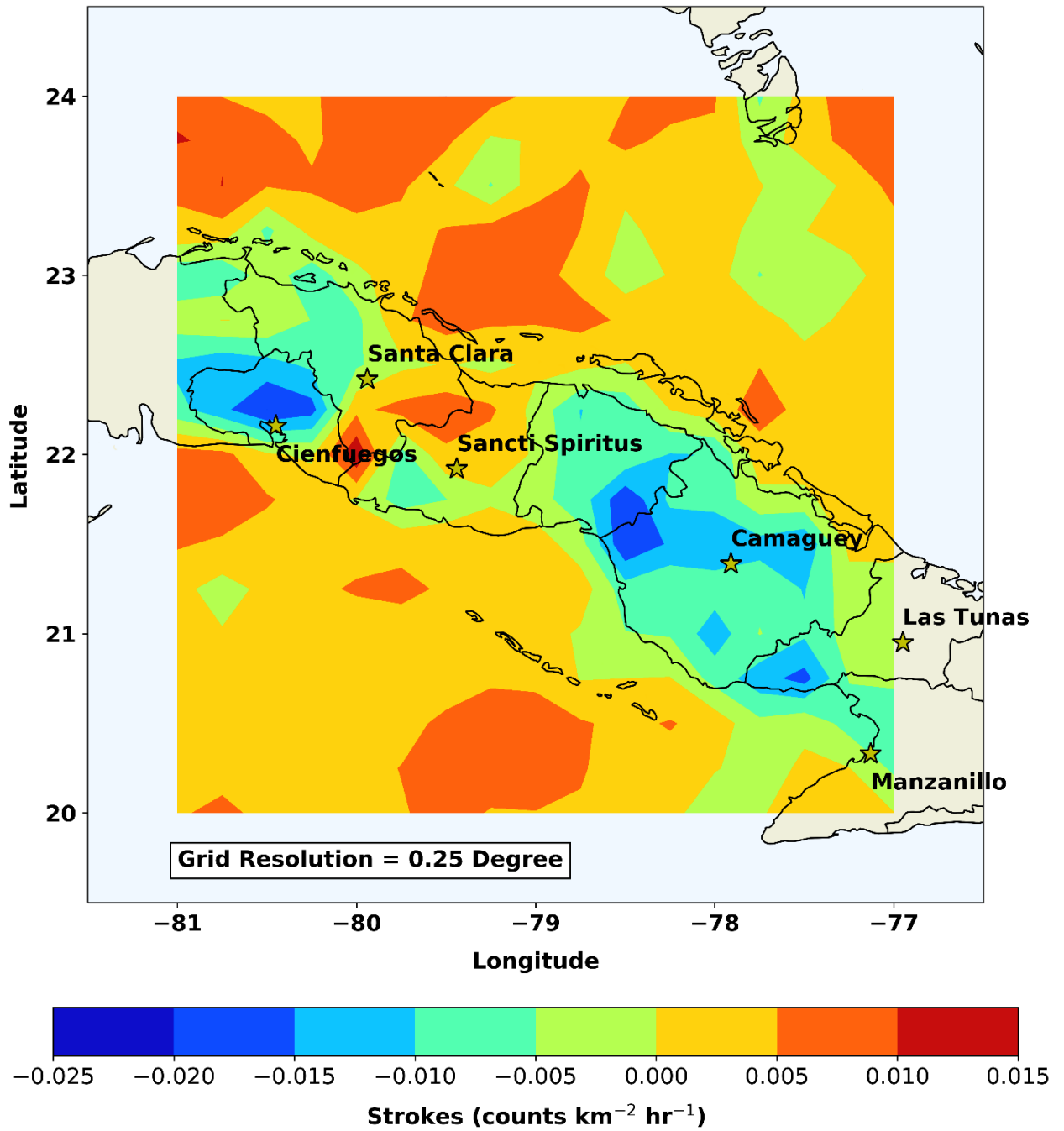
Figure 33. Cuba CP Difference (Forecast – Observed) June 2019.
