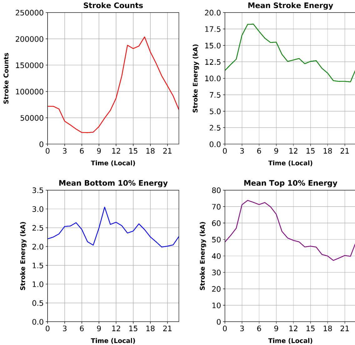
Figure 15. North Korea Stroke Diurnal Cycle 2016-2020: Stroke Counts (top left), Mean Stroke Energy (top right), Mean Bottom 10% Energy (bottom left), Mean Top 10% Energy (bottom right).
