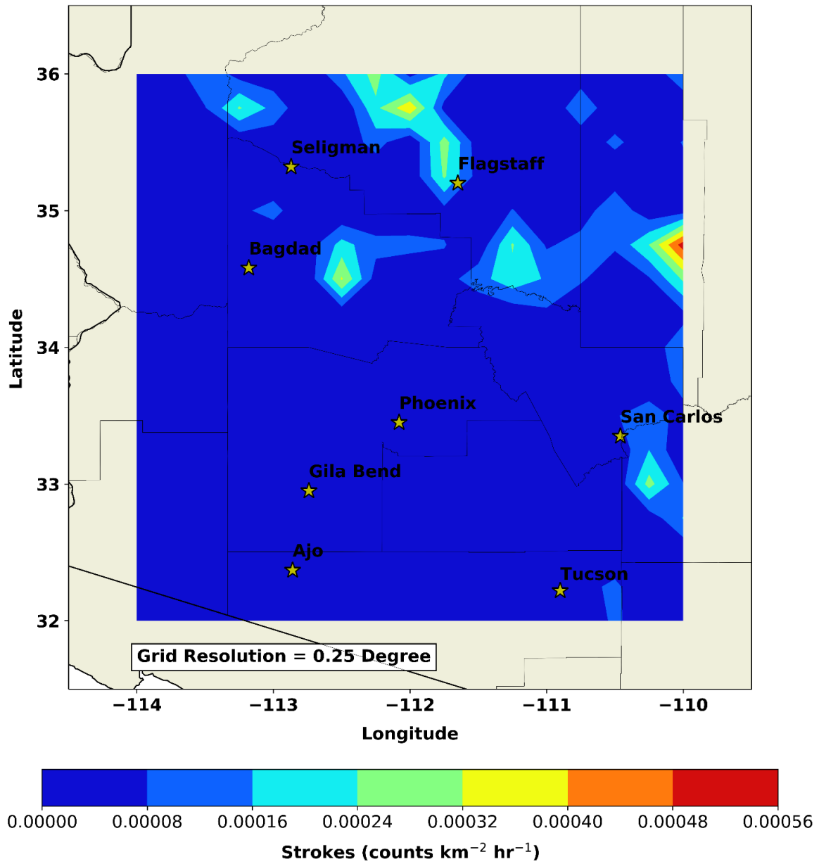
Figure 19. Arizona Observed Strokes June 2019.
