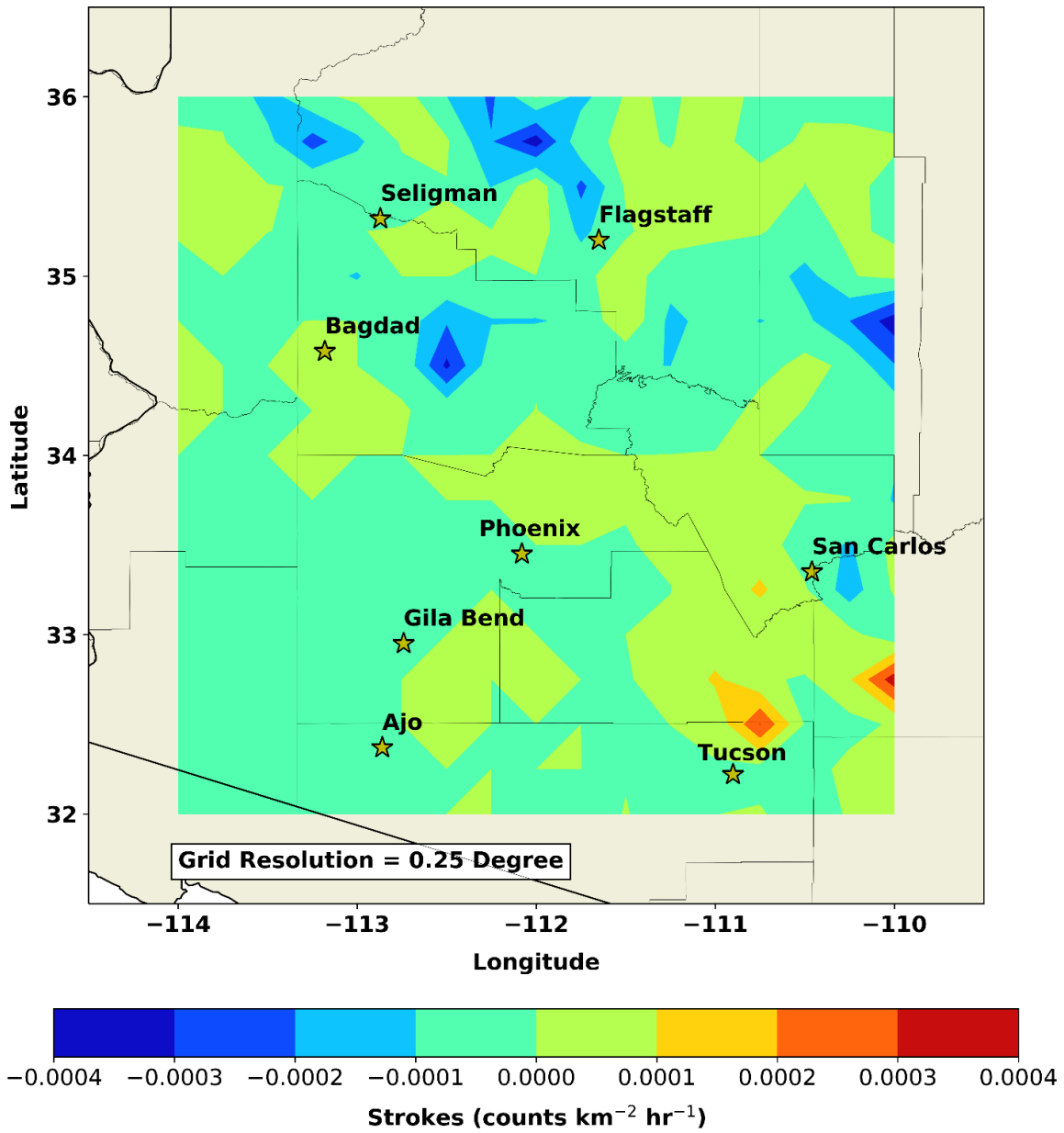
Figure 21. Arizona CP Difference (Forecast – Observed) June 2019.
