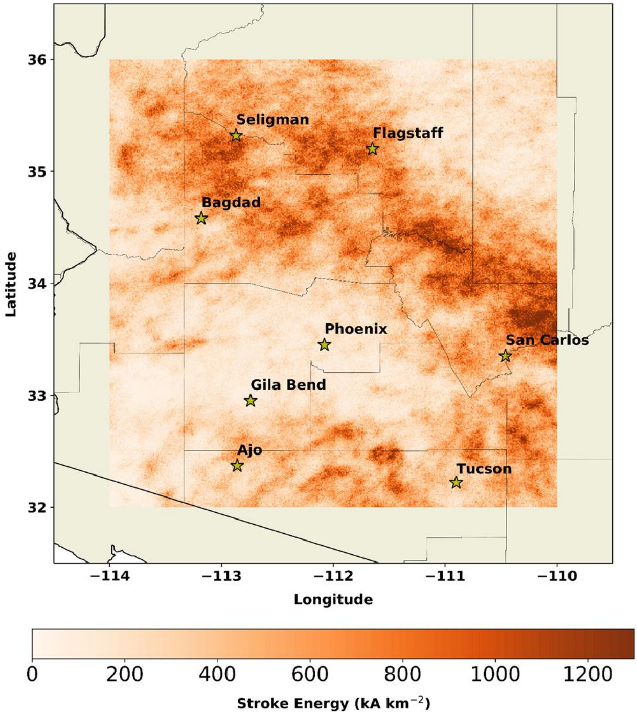
Figure 5. Arizona Stroke Energy 2016-2020.
