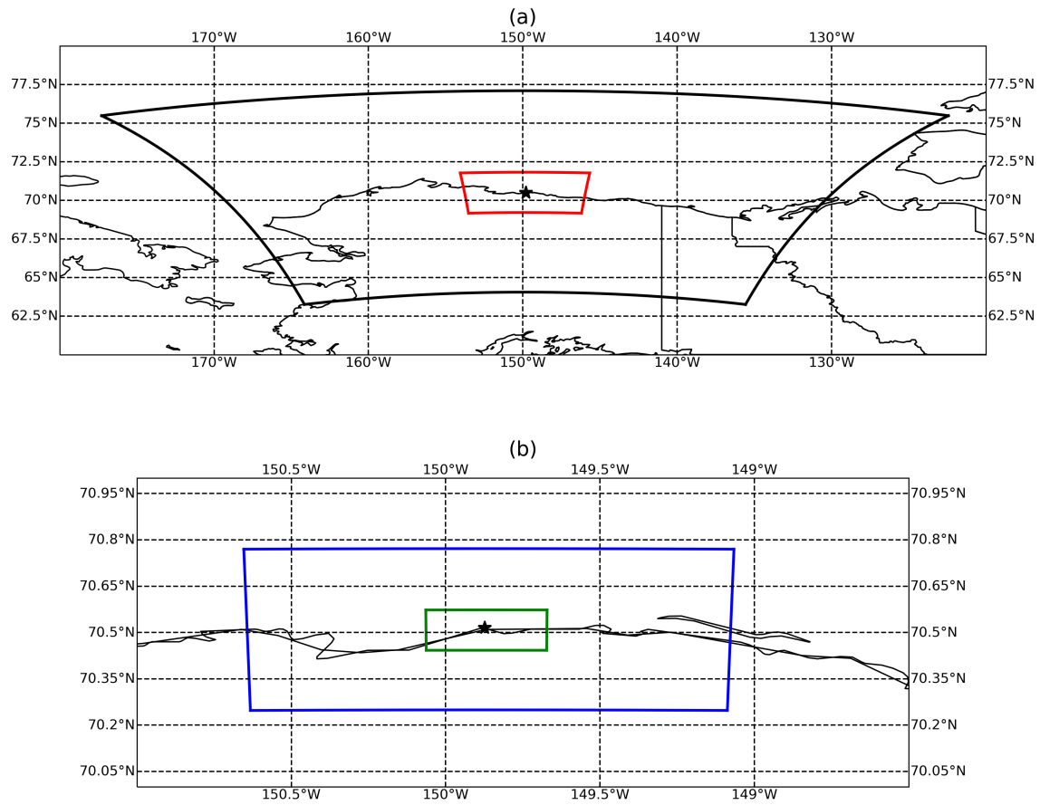
Figure 3. Domain boundaries specified in WRF for domain one (thick, black lines), two (red lines), three (blue lines), and four (green lines). The black star shows the location of OIktok.
