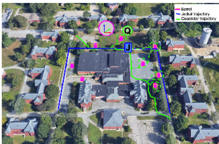
Fig. 37 The test facility at Medfield, Massachusetts, outside Boston. The blue trajectory is the initial trajectory of a Clearpath Jackal, and the green trajectory is the initial trajectory of a quadrotor using the stealthy semantic navigation strategy. When objects of interests are detected by the Jackal, the quadrotor is tasked with deviations to inspect and refine the pose of the objects, denoted by the dashed green lines. This scenario exercises the state estimation, object localization, coordinate frame alignment, and stealth navigation.
