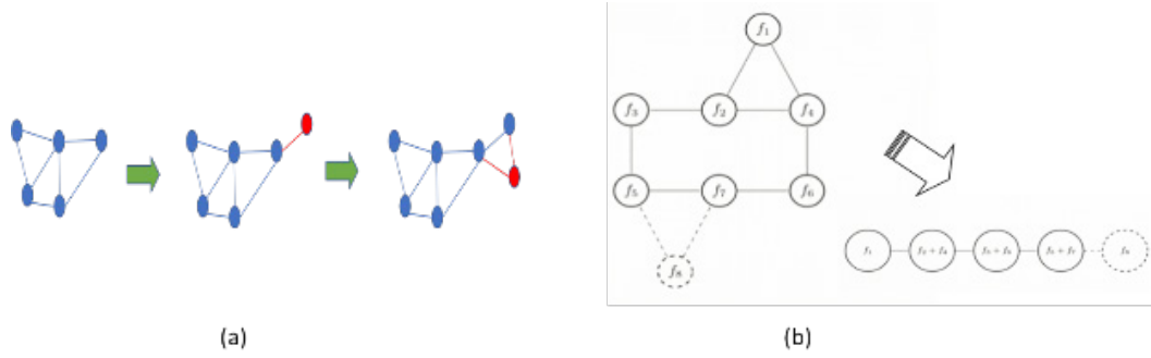
Fig. 8 (a) -G(V,E) and its evolution as new nodes and edges are added—the goal is to update the solution to the associated optimization program efficiently. (b) We reduce the general graph (left) to the chain graph (right); starting from the new node f_8 , expanding one edge outward each time, we collect all unassigned neighbors into a single node.
