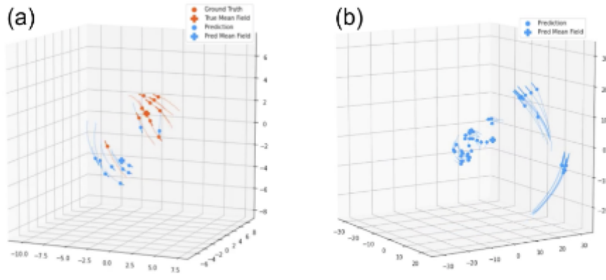
Applying the trained closed-loop dynamics on a swarm with (a) the same number of agents ( N=10 ) as the training data, and (b) more agents ( N=50 ) than the training data. It can be seen that in both cases, flocking behavior emerges in the swarm. For the swarm with 50 agents, sub-swarms form and flock. This is similar to if we simulate such a large swarm with the ground truth flocking controller.
