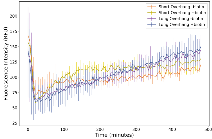
Figure 4. Expression of deGFP in biotinylated and unmodified linear DNA constructs in myTXTL Sigma 70 Master Mix kit reactions. No deGFP production was observed using any of the linear DNA variants.
