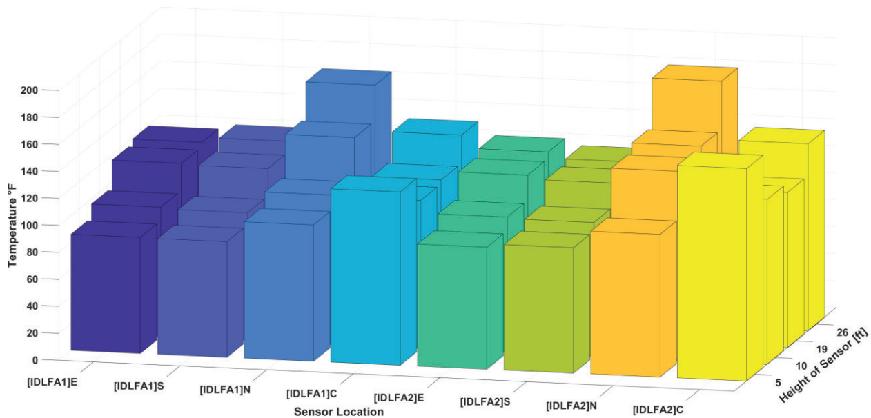
Figure 18. 110 gal ILDFA Mean Peak Temperatures With [IDLFA1] and Without [IDLFA2] Flushing
