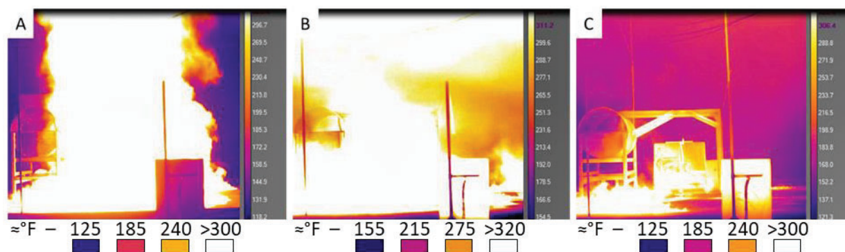
Figure 10. Infrared Images of a 30 gal Concrete Fuel Spill Fire at 15 s (A), 90 s (B), and 180 s (C) Time Points
