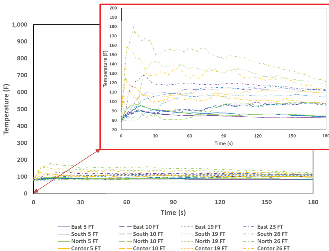
Figure 32. Air Temperatures from ILDFA-Mitigated Fire (Water Flushing Active, 165 gal JP-4)
