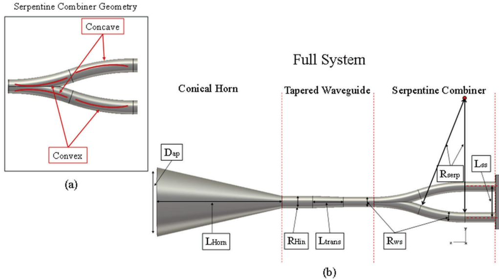
Figure 84. (a) Illustration of the Serpentine Combiner Geometry, (b) Illustration of the Different Parts of the System Combined
