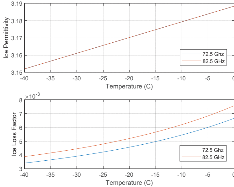
Figure 19. Dielectric Constant of Ice as Function of Temperature
