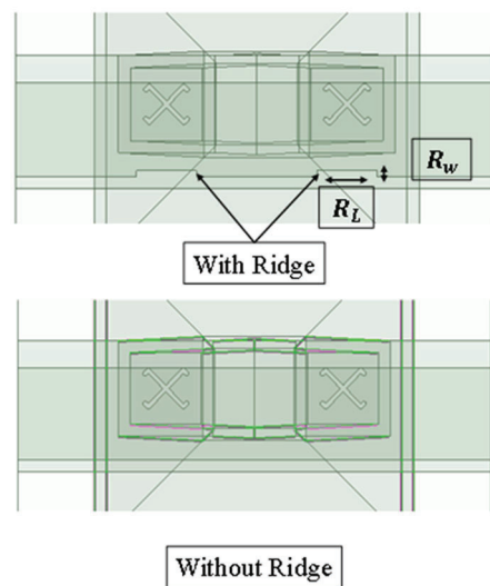
Figure 116. Illustration of the Design with and Without a Ridge in the Rectangular Waveguide
