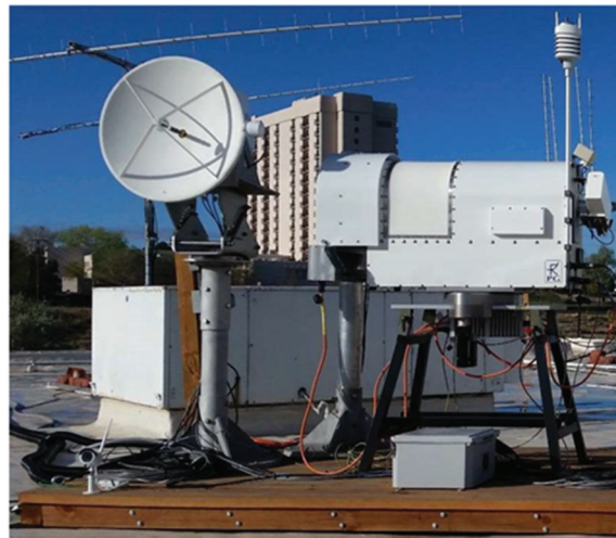
Figure 62. WTLE Receiver Site at COSMIAC
