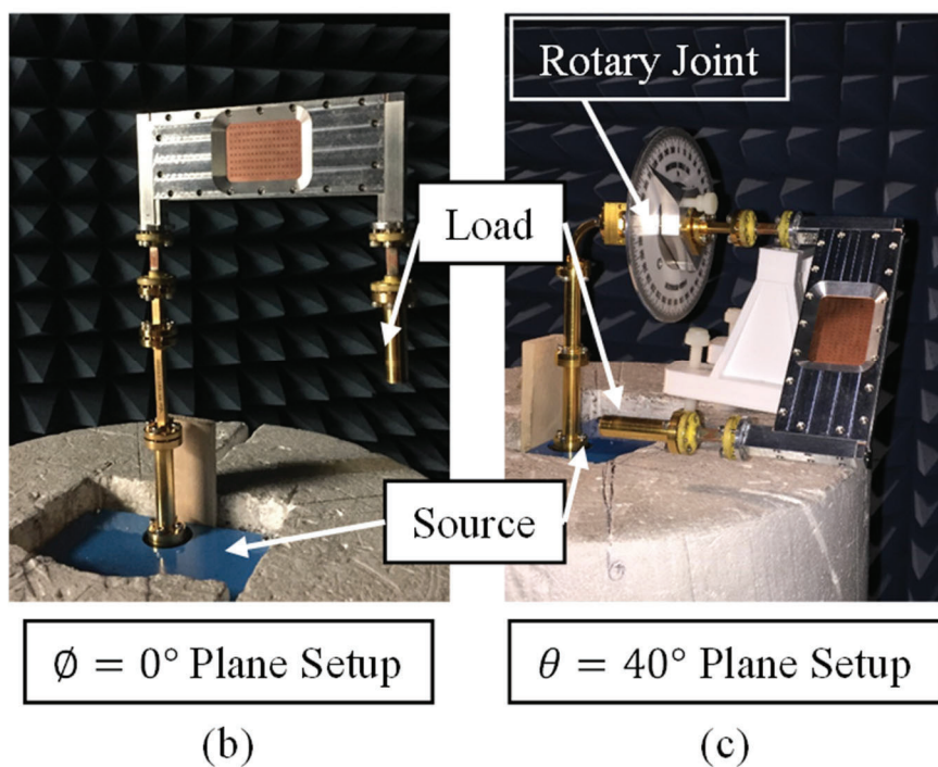
Figure 101. (a) Antenna Prototype, (b) Radiation Pattern Measurement Setup in the Elevation Plane ( \phi = 0^\circ ), and (c) Azimuthal Plane ( \theta = 40^\circ )
