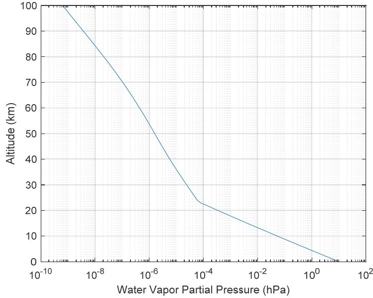
Figure 5. Plot of Water Vapor Partial Pressure as a Function of Altitude for the Standard Atmosphere Model (up to 100 km)
