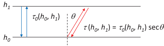
Figure 9. Illustration of Optical Thickness for a Single Layer of Atmosphere
