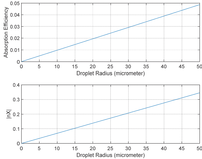
Figure 21. Absorption Efficiency and |n\chi| as a Function of Droplet Radius ( T = 15 \text{ }^\circ\text{C} , f = 82.5 \text{ GHz} )
