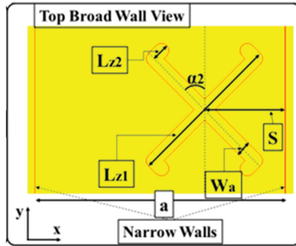
Figure 65. z-shaped Arm Cross-slot Structure
