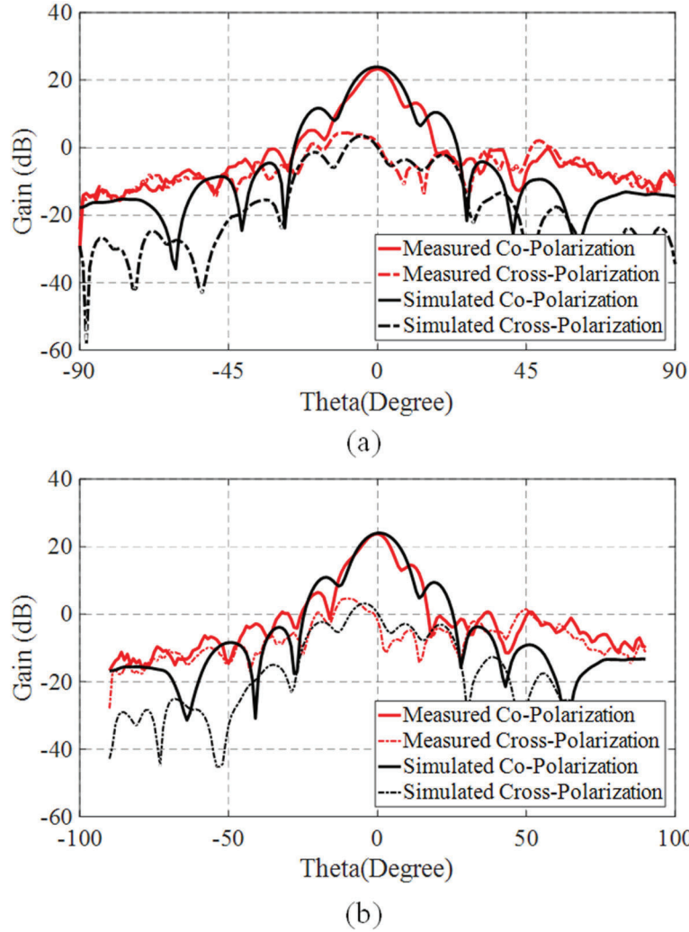
Figure 104. Simulated and Measured Gain Patterns of the Array in the Azimuth Plane ( \theta=40^\circ ) at 85 GHz When (a) Port 1 is Fed, or (b) Port 2 is Fed
