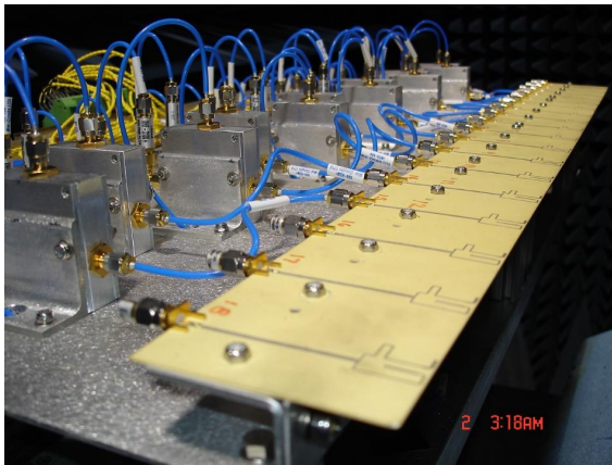
S-band, Linear Array Antenna Code 5317 (Dorsey & Pickles)
