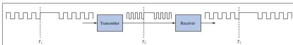
Figure 9-6. Measuring STC Latency
