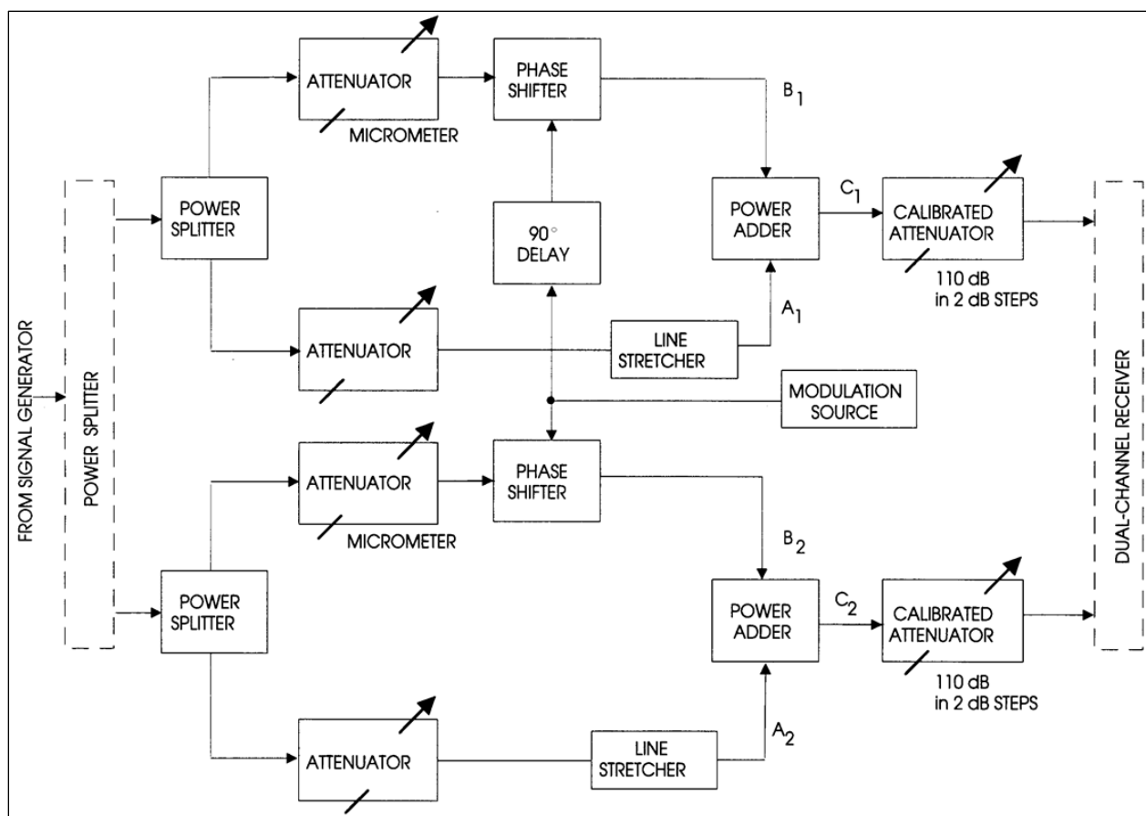
Figure 5-3. Diversity Signal Simulator
