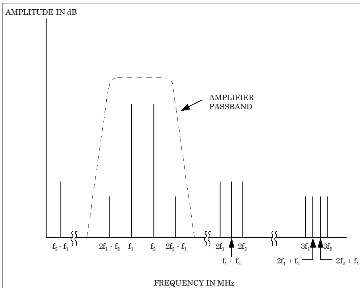
Figure A-1. Illustration of Spectrum for Two Fundamental Frequencies, F1 and F2, with Second- and Third-Order Response
