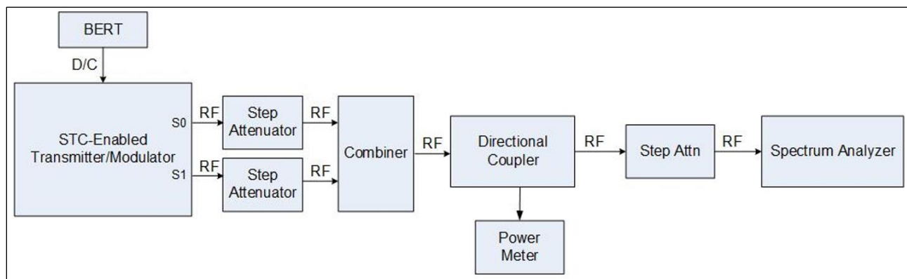
Figure 9-11. Setup for Bandwidth Measurement Test
