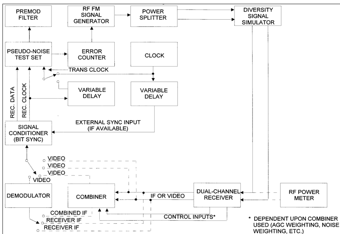
Figure 5-2. Dynamic Evaluation Test Setup for Diversity Signal Combiner
