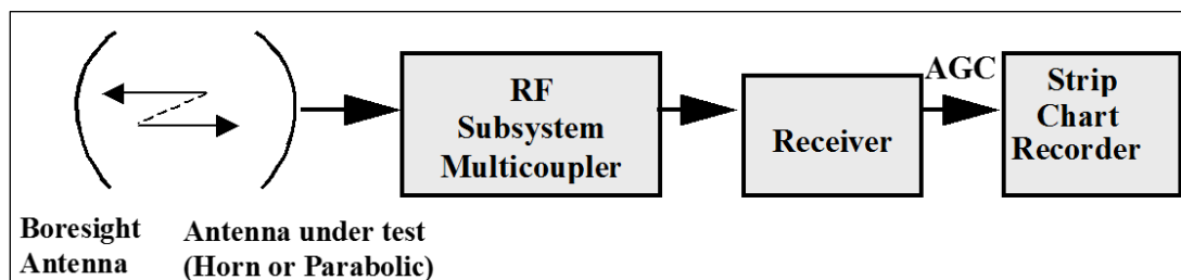
Figure 1-9. Antenna Gain Measurement using a Strip Chart Recorder
