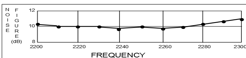
Figure 4-2. Noise Figure Plot
