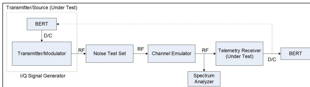
Figure 10-6. Setup using Channel Emulator for Dynamic Channel Multipath Test
