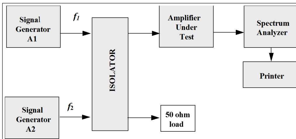
Figure 2-5. Test Setup for Determination of Intercept Point
