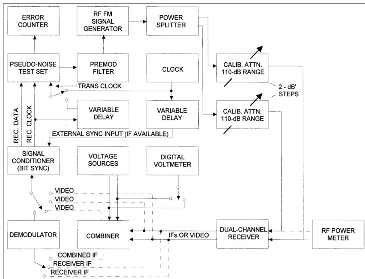
Figure 5-1. Static Evaluation Test Setup for Diversity Signal Combiner
