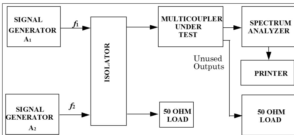
Figure 3-5. Test Setup for Determination of Intercept Point
