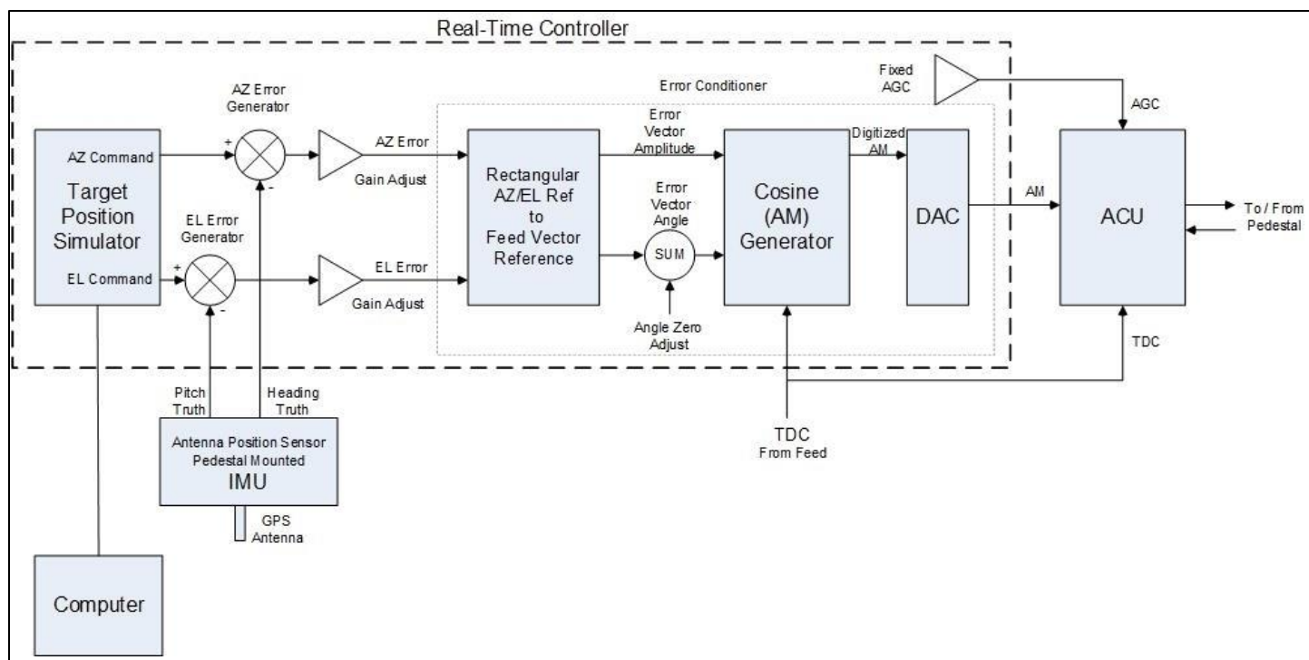
Figure 1-18. Detailed System Configuration
