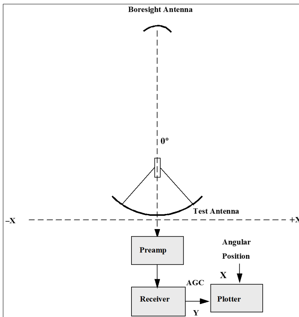
Figure 1-10. Antenna Pattern Measurement Setup
