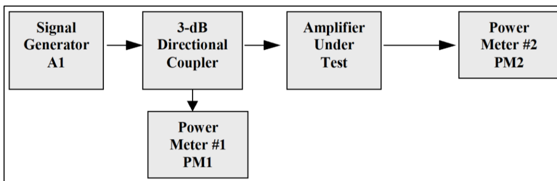
Figure 2-1. Test Setup for Measurement of Amplifier Gain Compression
