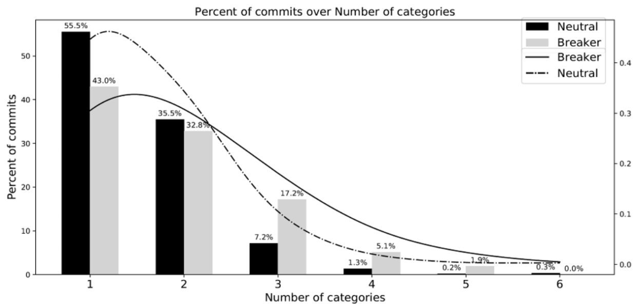
Figure 2. Percent of Commits Over the Number of Categories
