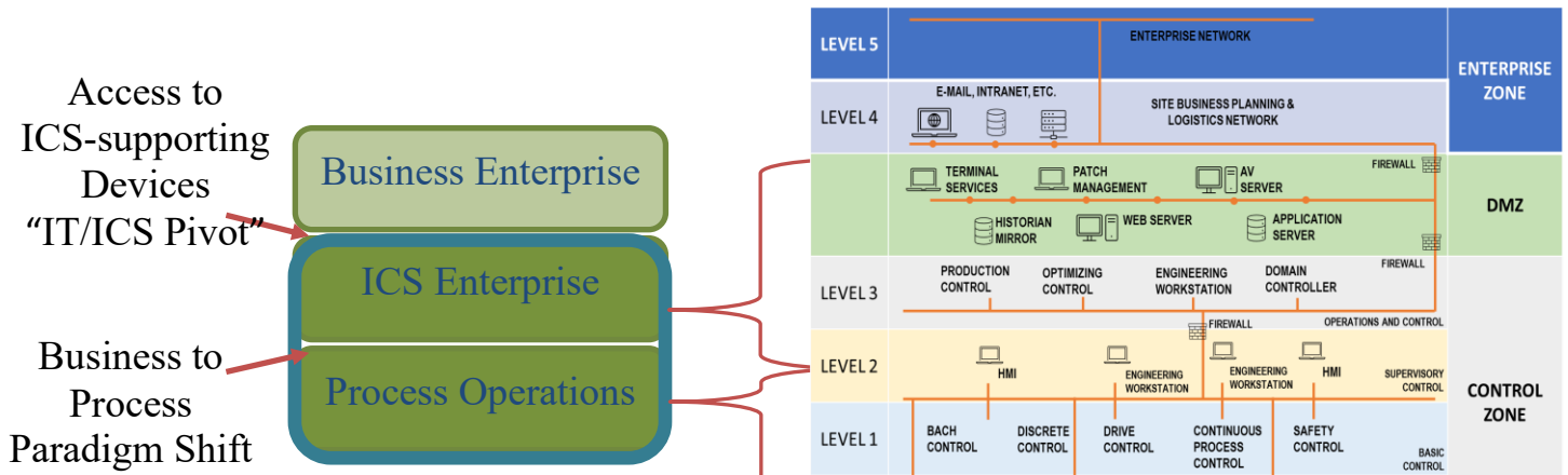
Figure 1-1. Analytic Focus Mapped to Purdue Model
