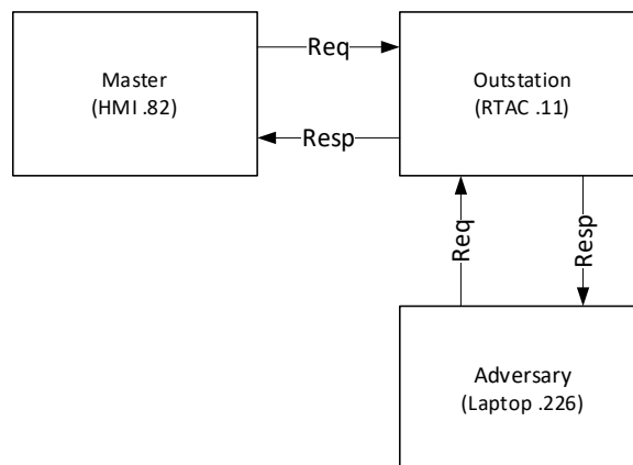
Figure 4-4. Test Setup
