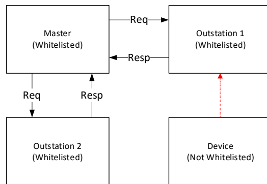
Figure 4-8. Analytic Test Setup
