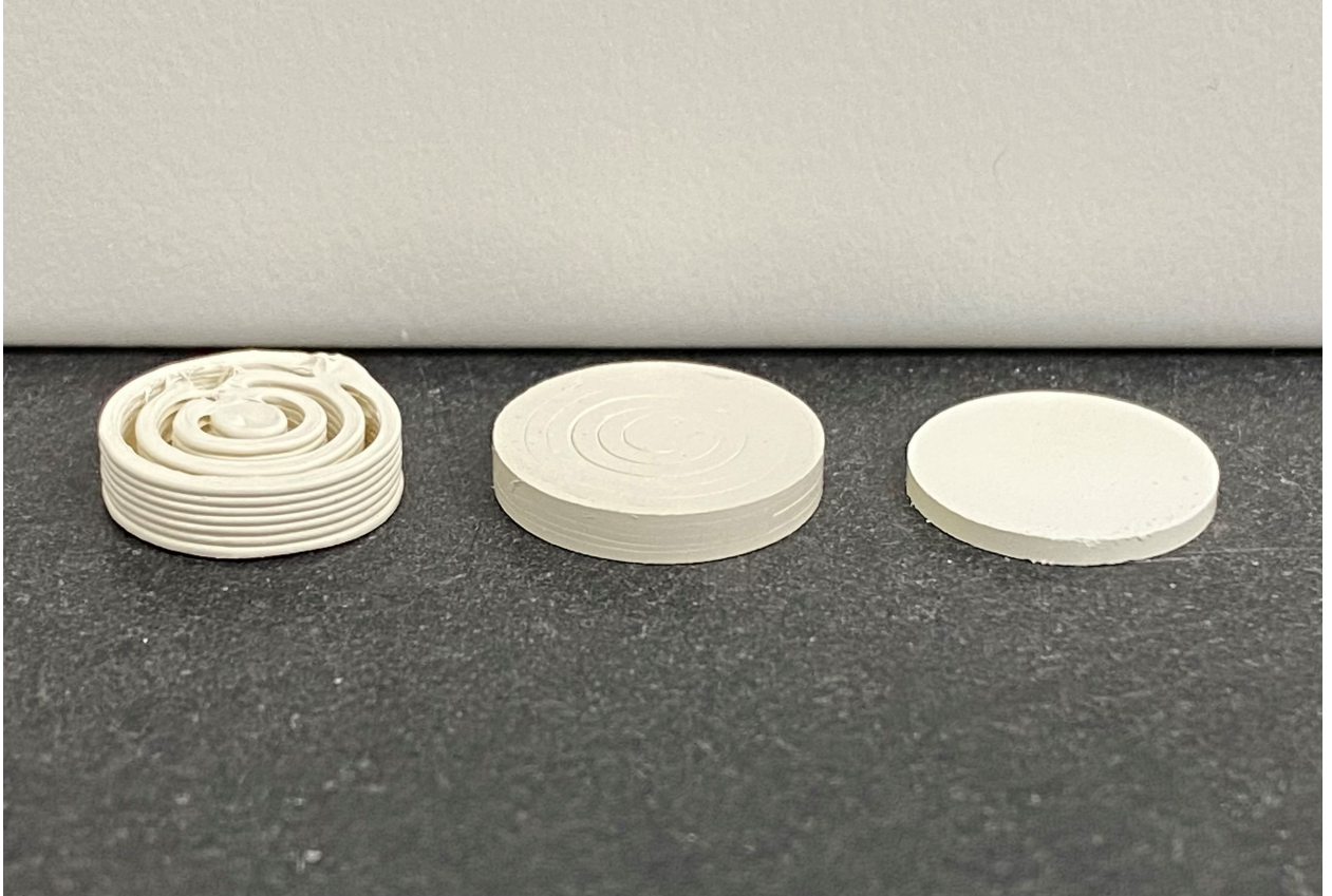
Figure 1. Disc preform consisting of concentric rings (left), disc preform after pressing (middle), and a disc pressed from PZT powder (right).
