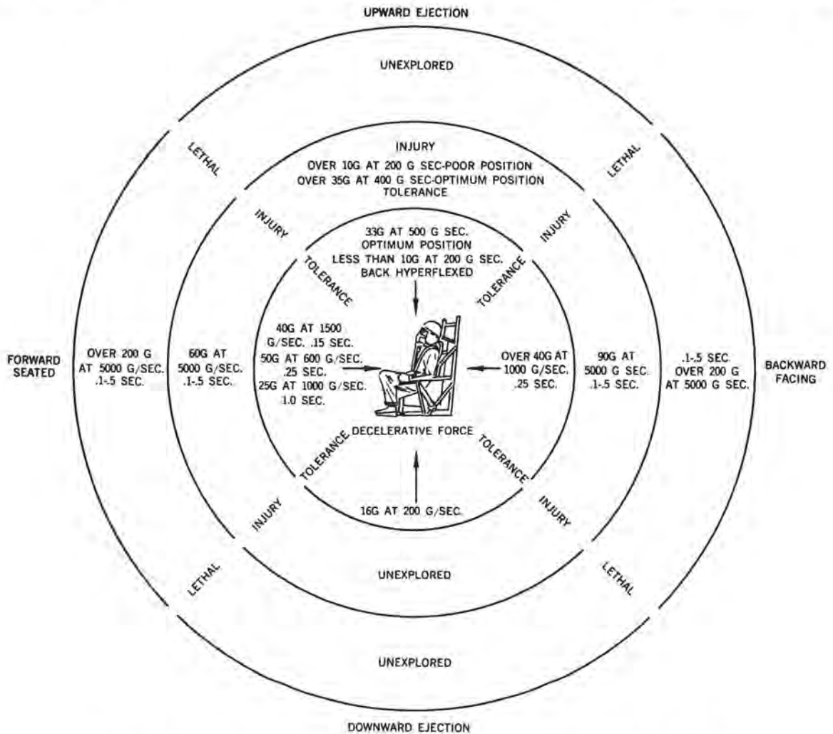
Figure 4-19. Tolerance, Injury and Lethal Limits for Force Applied Through the Principal Axes of Body Orientation.
