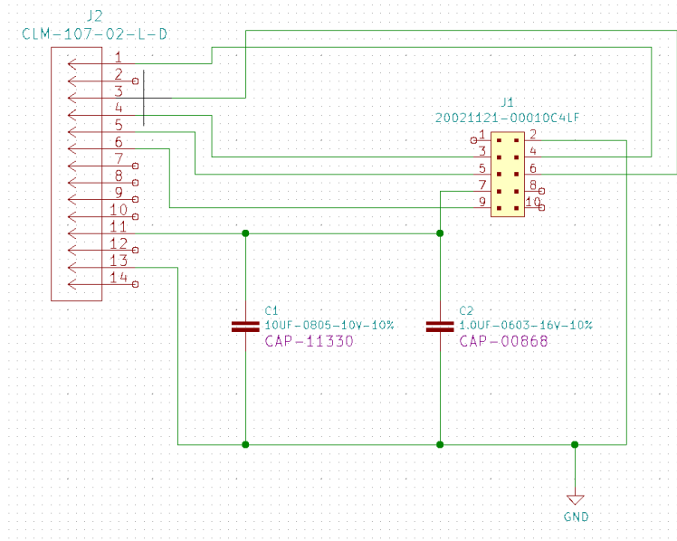
Fig. 4 Schematic for the daughterboard
