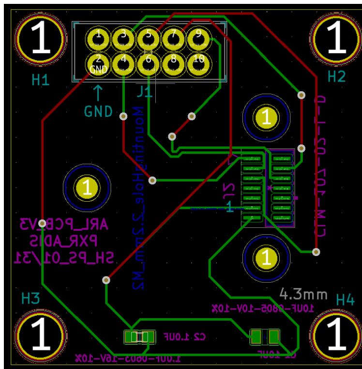
Fig. 5 PCB layout of the daughterboard
