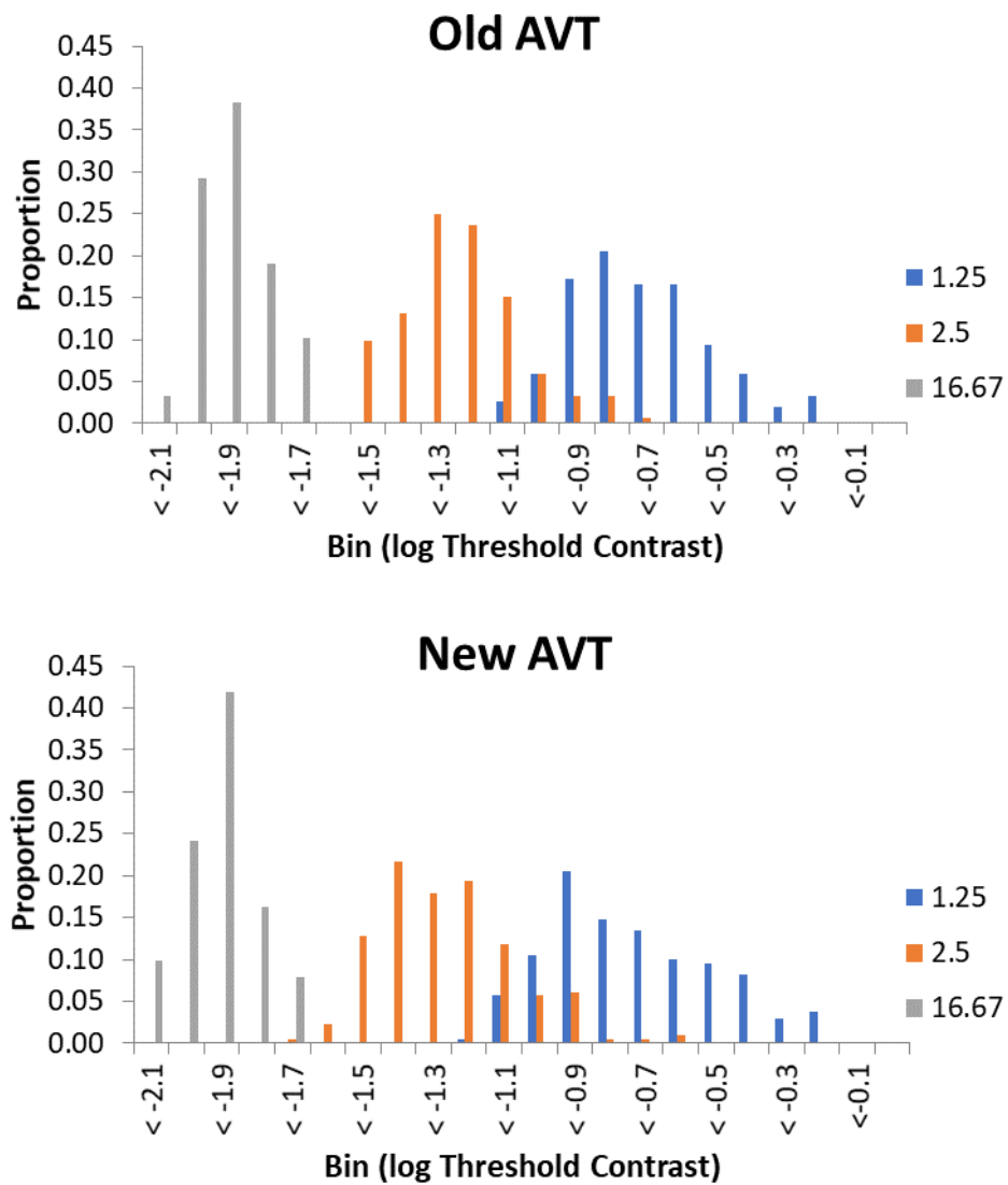
Figure B-1. Contrast sensitivity test histograms. Top: old AVT. Bottom: new AVT.
