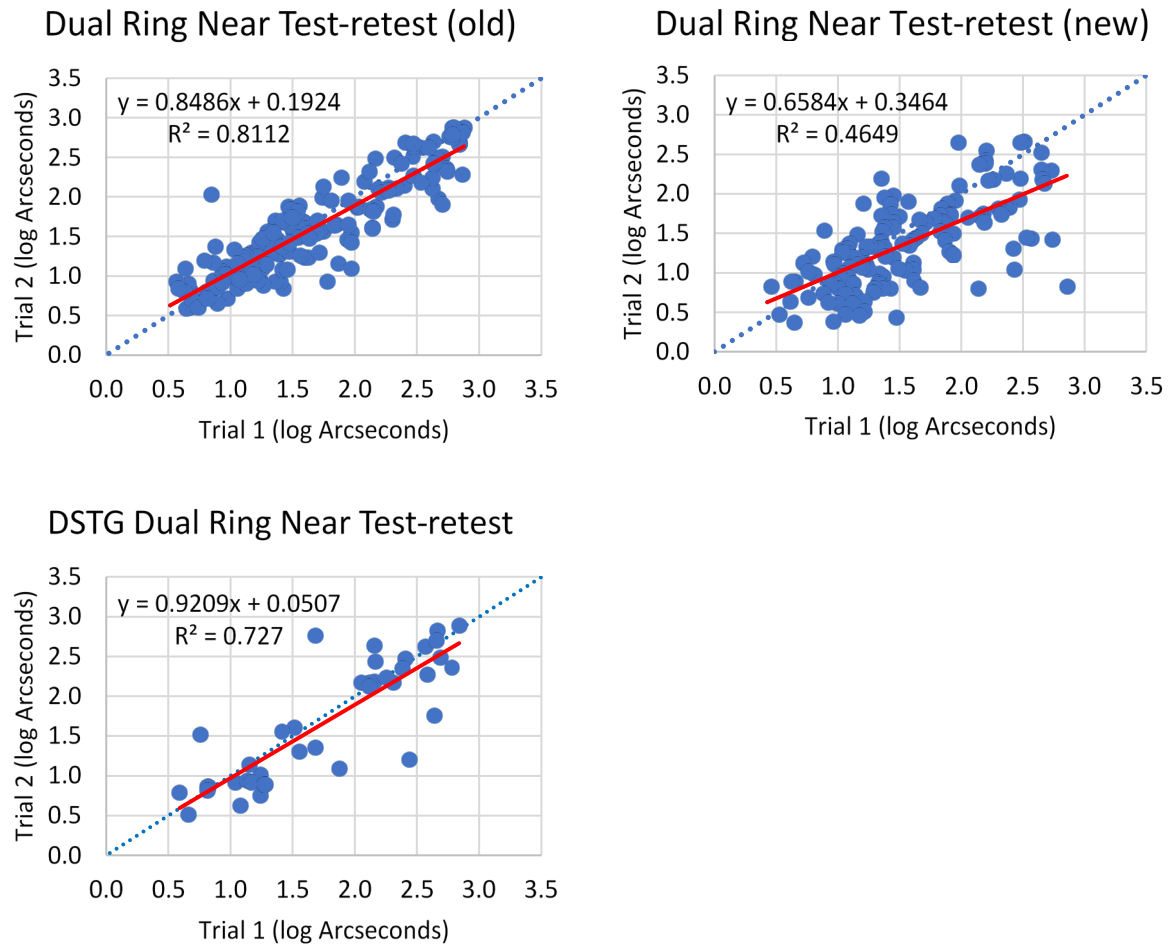
Figure 22. Dual Ring Near test-retest scores for OBVA old AVT, OBVA new AVT, and DSTG old AVT.
