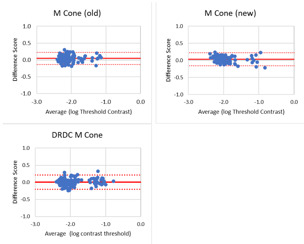
Figure 17. OCCT M cone Bland Altman graphs for OBVA old AVT, OBVA new AVT, and DRDC old AVT.
