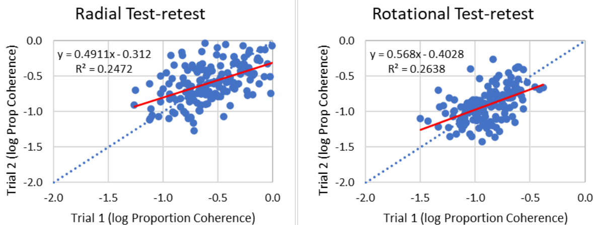
Figure 32. Motion test-retest scores.
