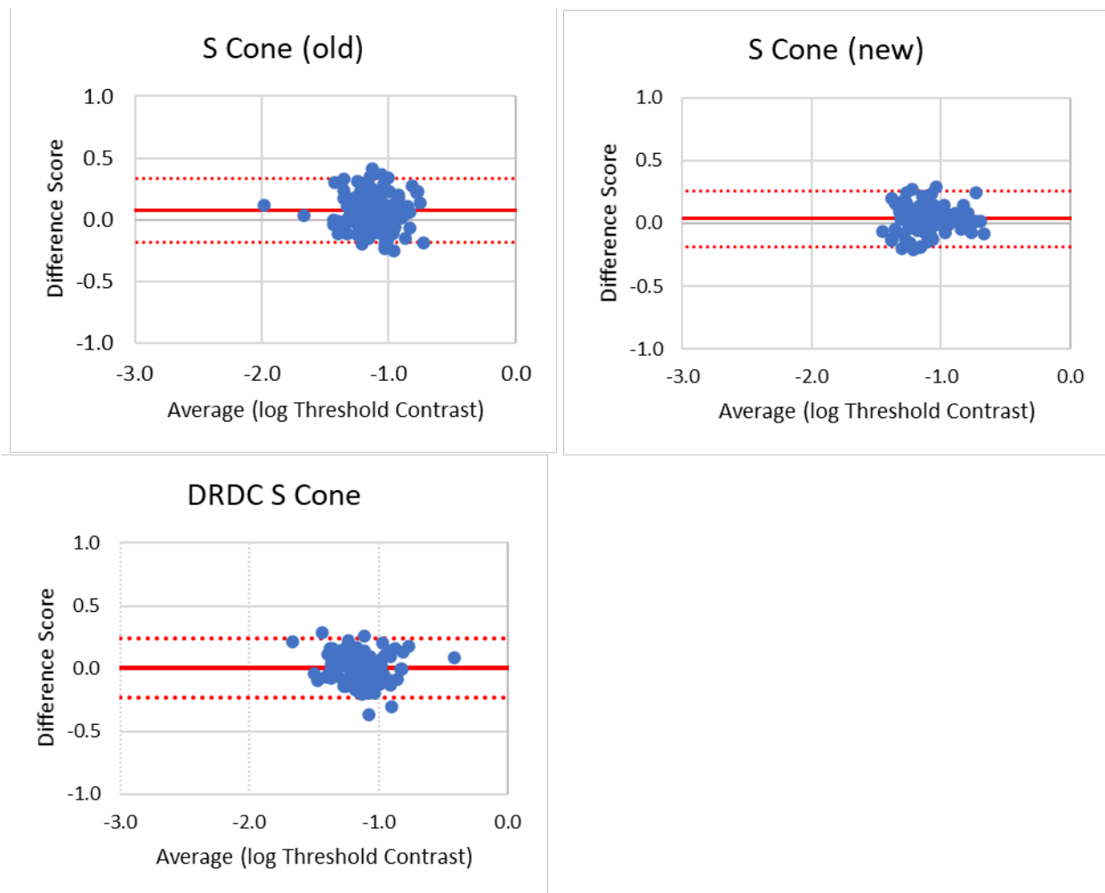
Figure 18. OCCT S cone Bland Altman graphs for OBVA old AVT, OBVA new AVT, and DRDC.
