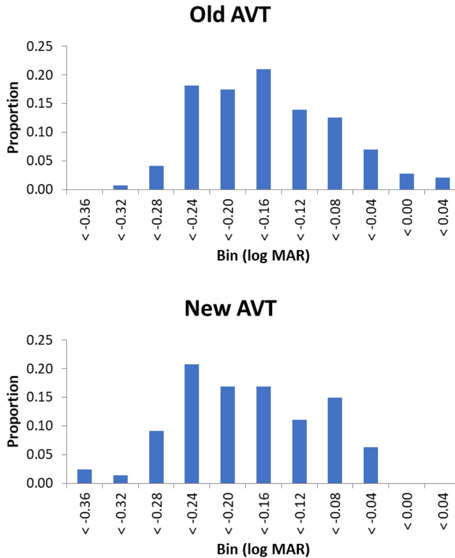
Figure B-2. 4M acuity test histograms. Top: old AVT. Bottom: new AVT.
