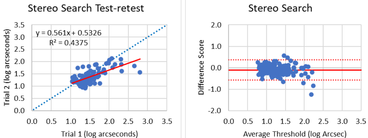
Figure 27. Left: Stereo search test-retest scores. Right: Stereo search Bland-Altman graph
