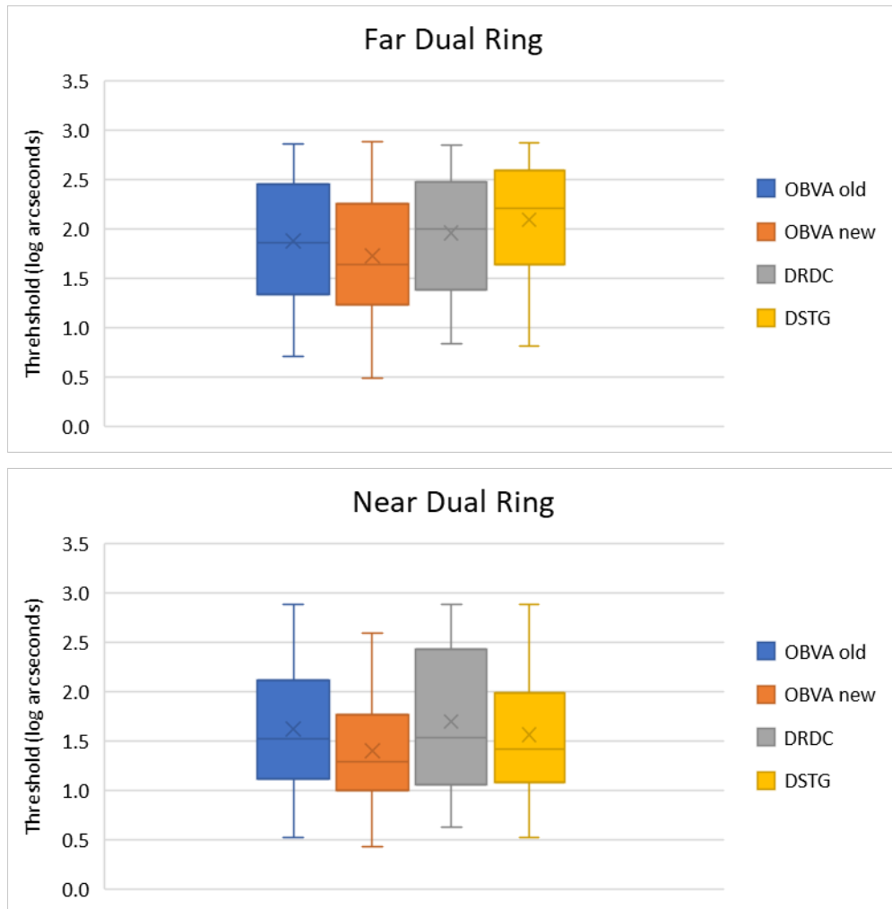
Figure 25. Dual Ring Far and Near boxplots for OBVA old AVT, OBVA new AVT, and DSTG old AVT.
