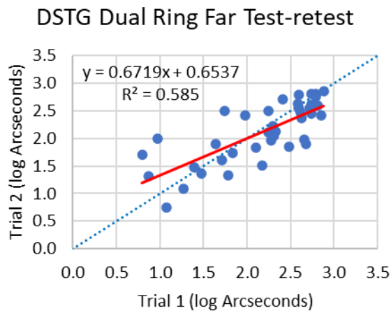
Figure 21. Dual Ring Far test-retest scores for OBVA old AVT, OBVA new AVT, and DSTG old AVT.
