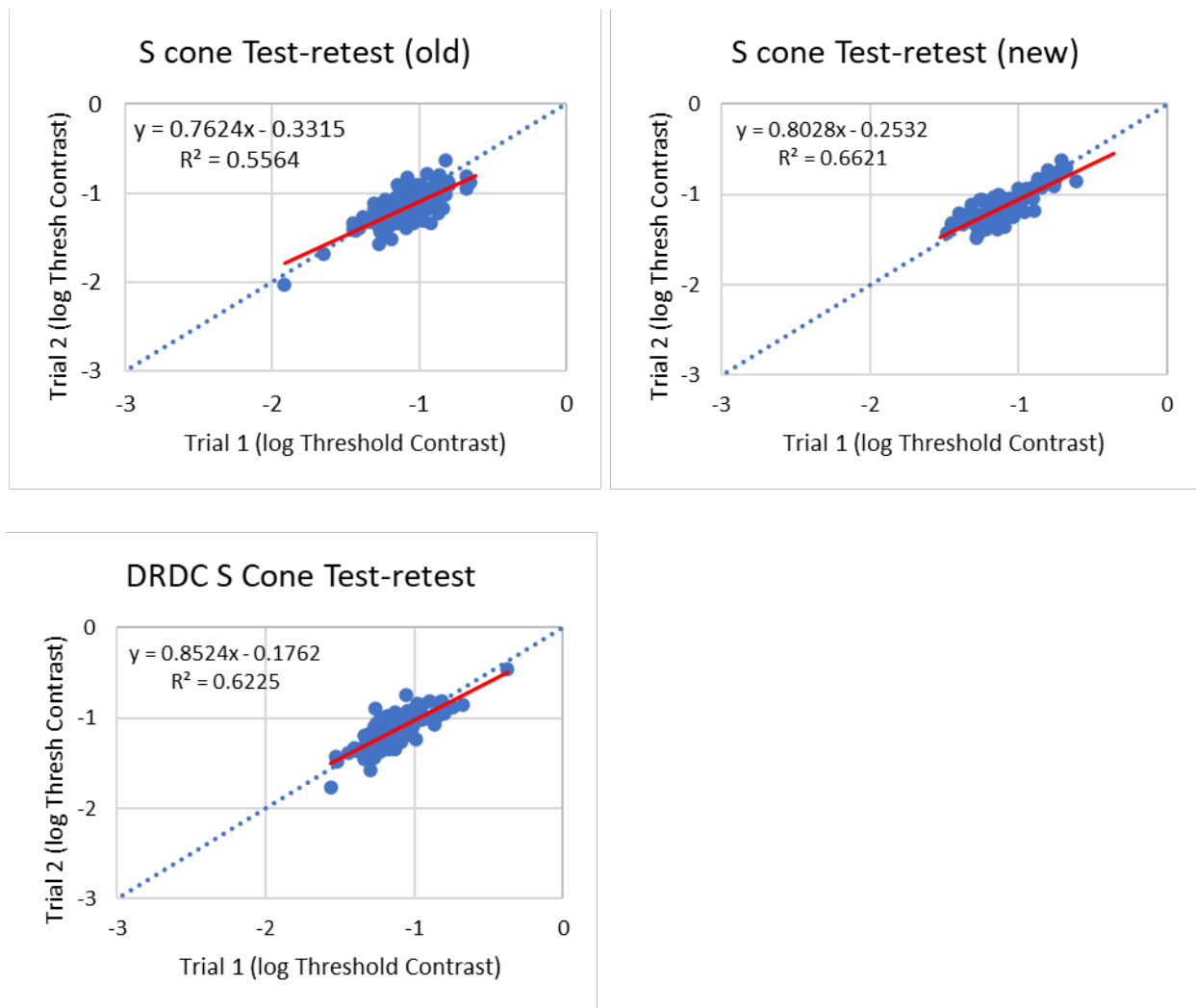
Figure 15. OCCT S cone test-retest scores for OBVA old AVT, OBVA new AVT, and DRDC old AVT.
