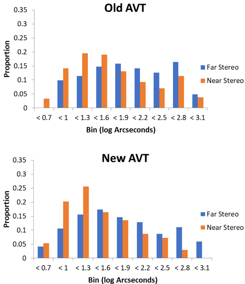
Figure B-5. Dual ring test histograms. Top: old AVT. Bottom: new AVT.
