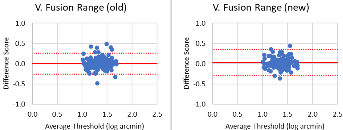
Figure 31. Vertical fusion range Bland-Altman graphs for OBVA old AVT and new AVT
