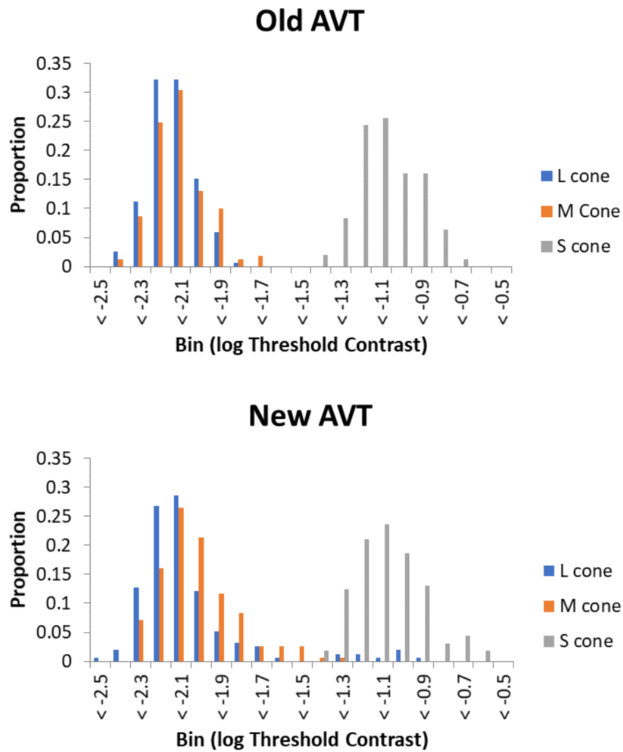
Figure B-3. OCCT test histograms. Top: old AVT. Bottom: new AVT.
