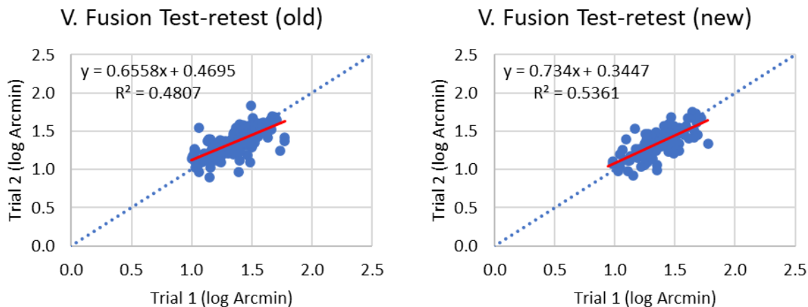
Figure 29. Vertical fusion range test-retest scores for OBVA old AVT and new AVT
