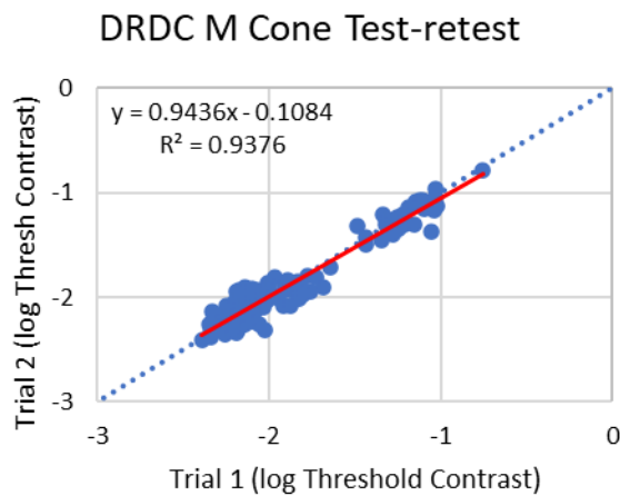
Figure 14. OCCT M cone test-retest scores for OBVA old AVT, OBVA new AVT, and DRDC old AVT.
