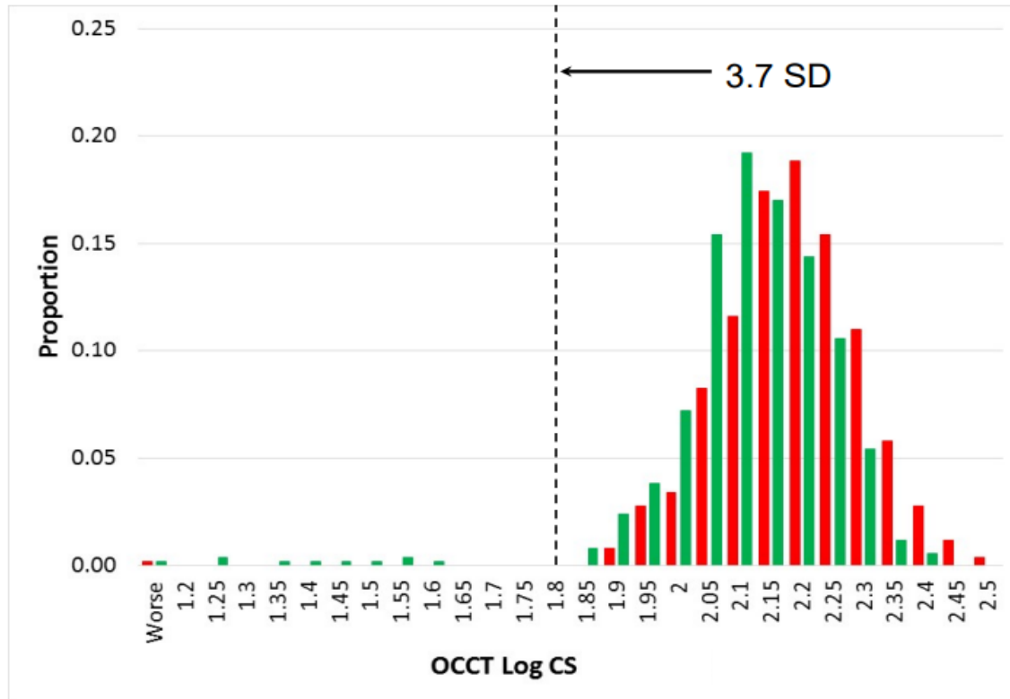
Figure 19. Histogram showing spread of binocular OCCT L cone (red) and M cone (green) scores. Cutoff score for color vision abnormals is 3.7 standard deviations from the mean. From Winterbottom, Gaska, Wright, & Hadley, 2017. International Color Vision Society 24th Symposium.
