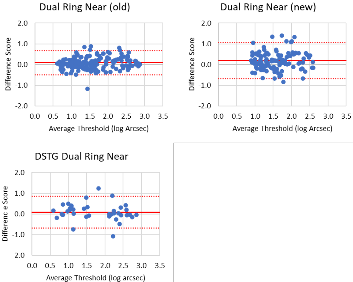
Figure 24. Dual Ring Near Bland Altman graphs for OBVA old AVT, OBVA new AVT, and DSTG old AVT.
