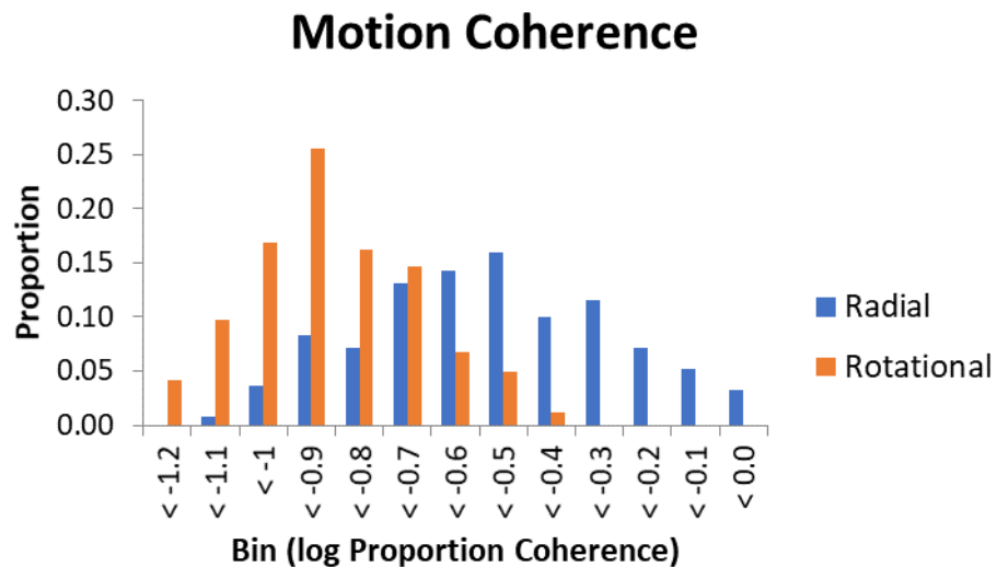
Figure B-10. Motion test histogram.
