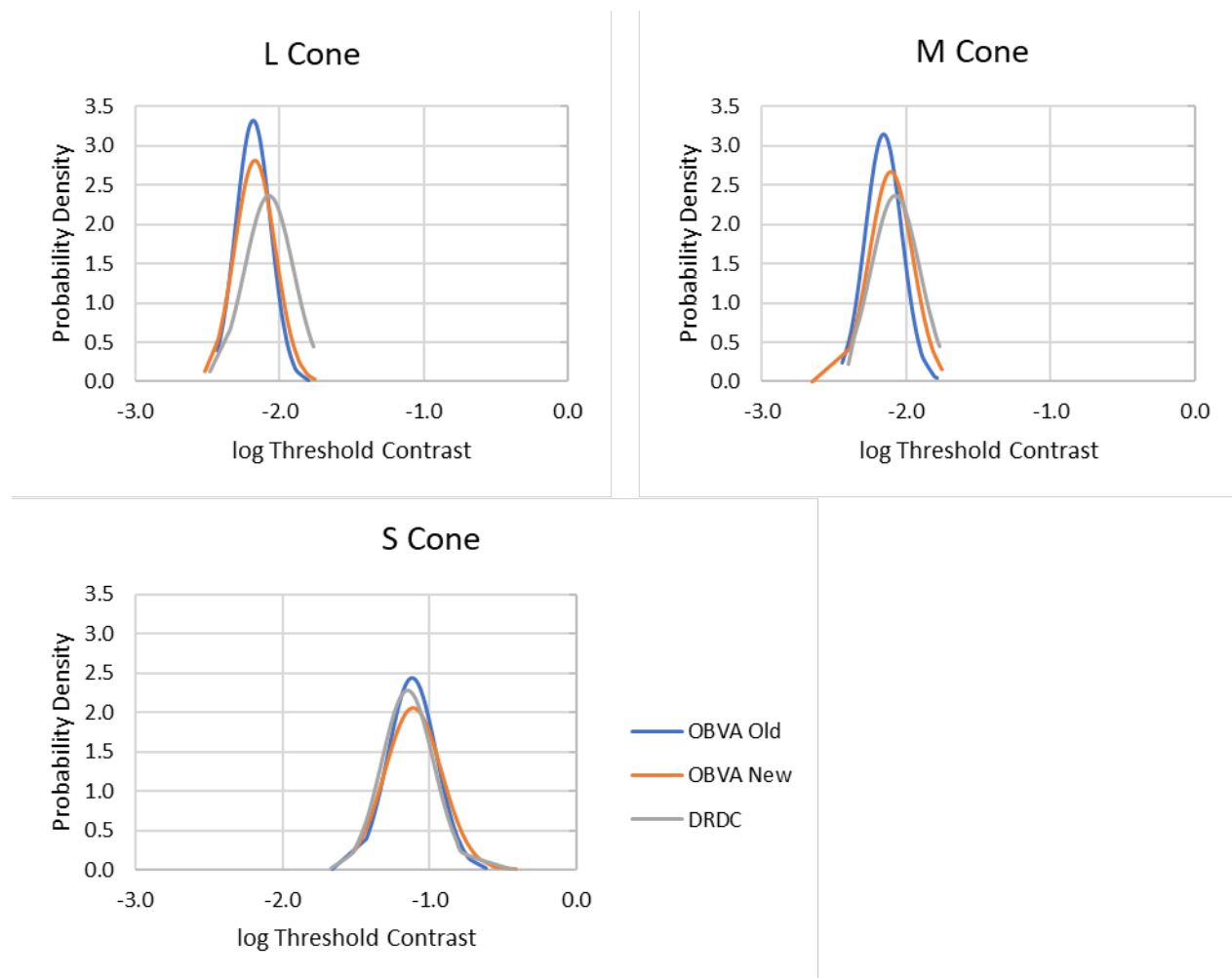
Figure 20. OCCT probability density graphs for OBVA old AVT, OBVA new AVT, and DRDC.
