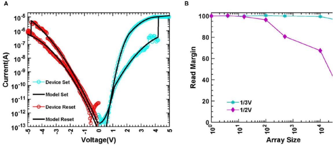
Figure 20. Circuit Level Modeling of 1S1R-based Crossbar Array. (A) SPICE simulation of single device IV sweep (solid line). (B) Normalized Readout Margin for different array sizes. [18]
