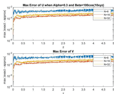
Figure 19: \alpha = 0.3
