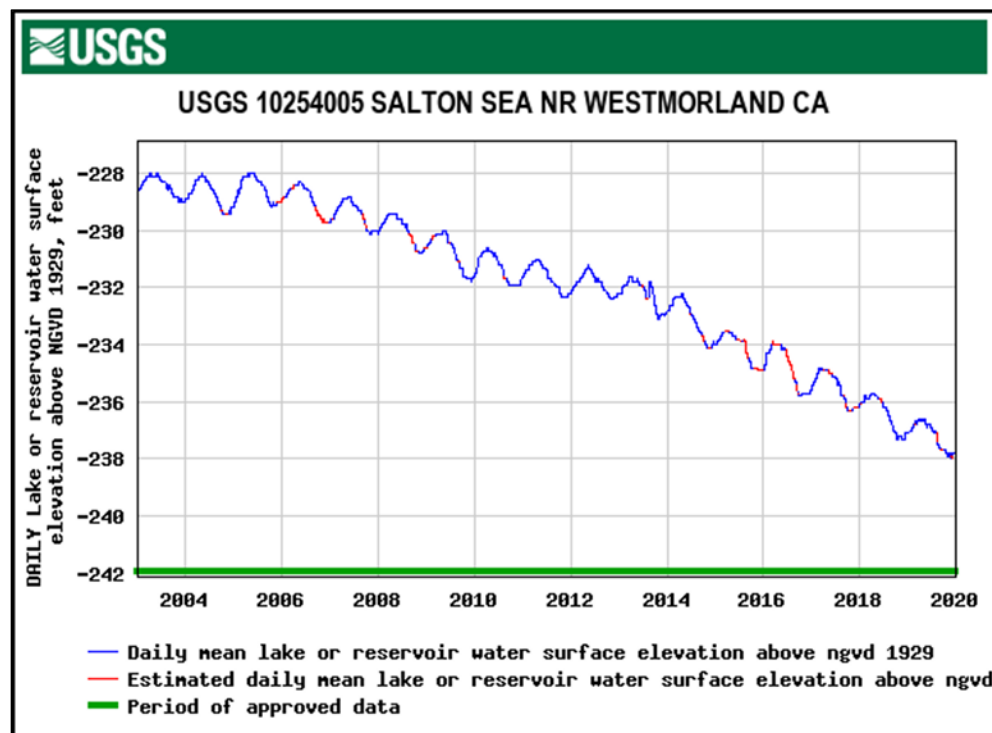
Figure 2. Salton Sea Elevation, 2003-2020
