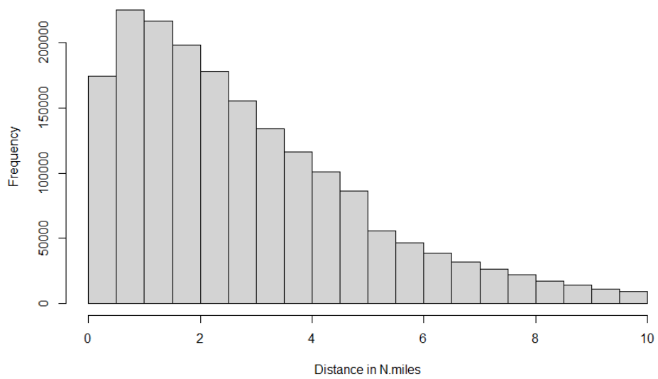
Figure 43. Cold Season of 2019 for Cloud-to-Ground
