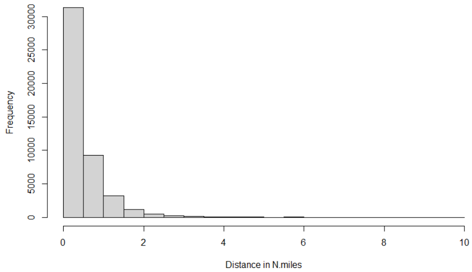
Figure 47. Warm Season of 2019 for Total Lightning
