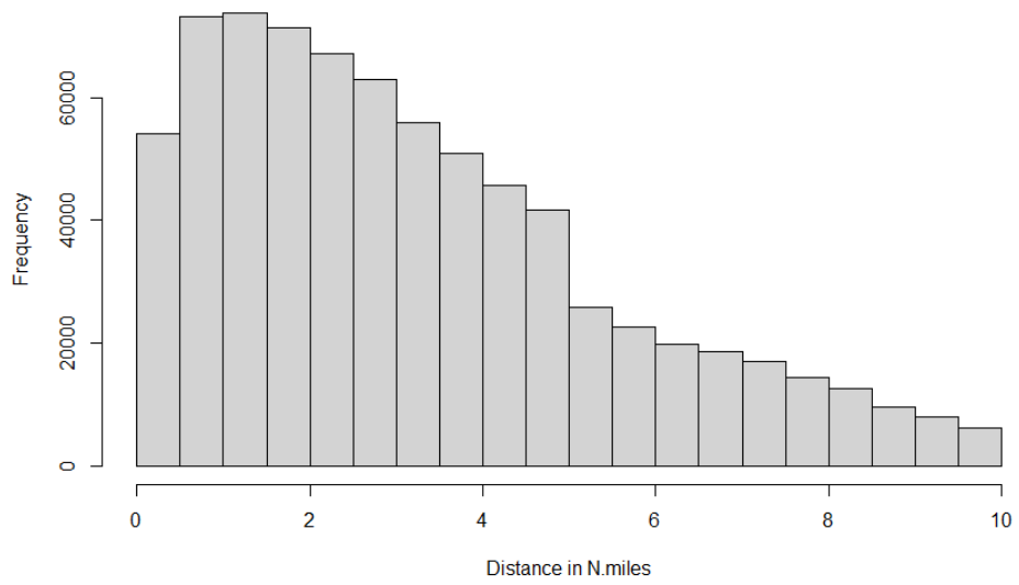
Figure 44. Cold Season of 2020 for Cloud-to-Ground
