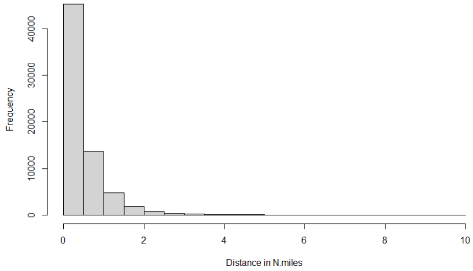
Figure 25. Histogram for 2019 Using Total Lightning
