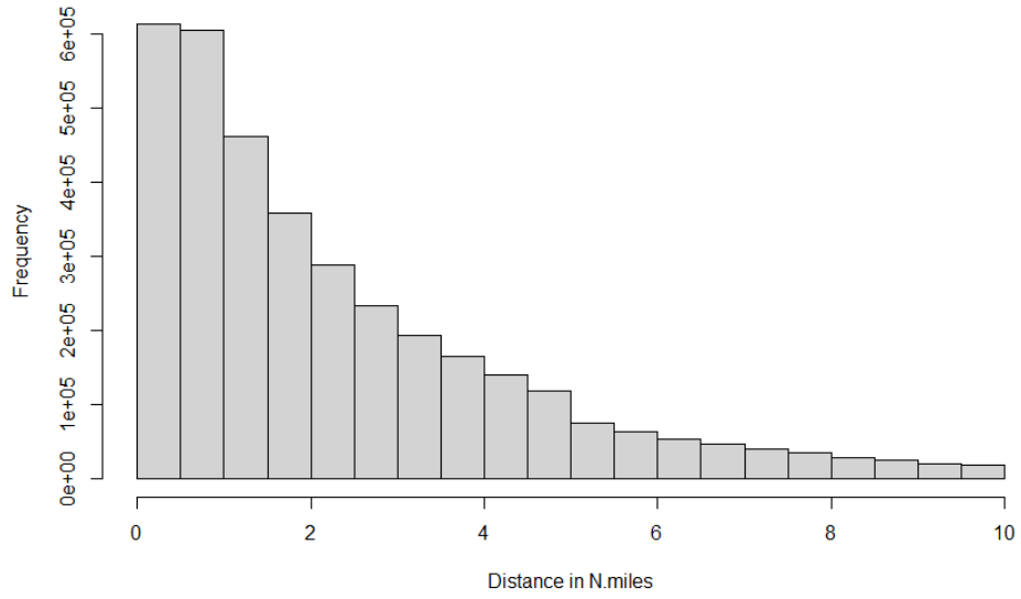
Figure 40. Warm Season of 2020 for Cloud-to-Ground
