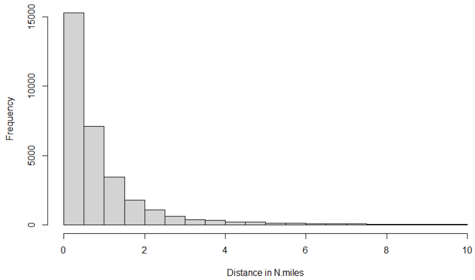
Figure 46. Warm Season of 2018 for Total Lightning
