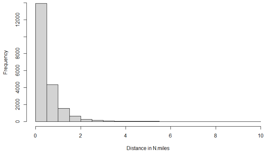
Figure 51. Cold Season of 2019 for Total Lightning
