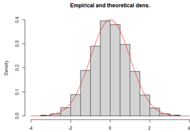
Figure 8. Empirical vs. Theoretical Density Examples
