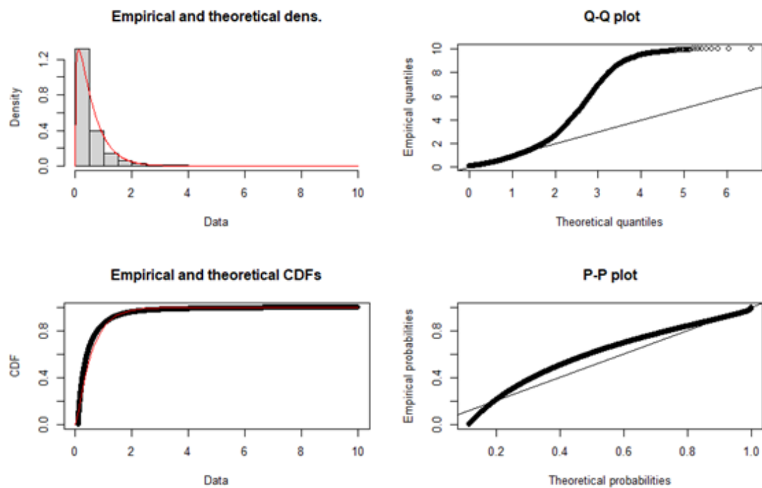
Figure 29. Gamma Distribution for the Warm Season
