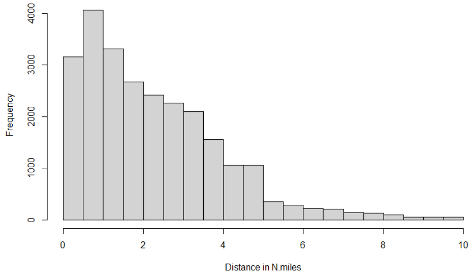
Figure 42. Cold Season of 2018 for Cloud-to-Ground
