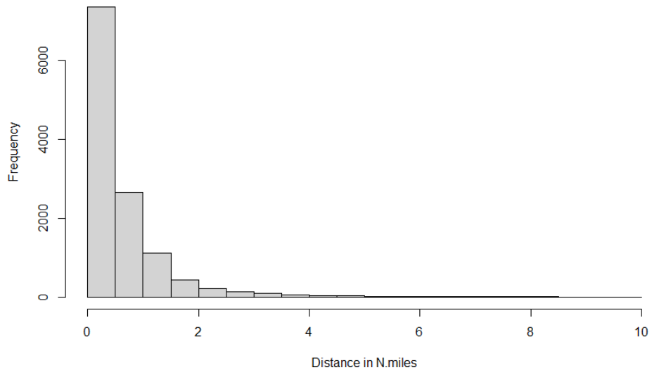
Figure 50. Cold Season of 2018 for Total Lightning
