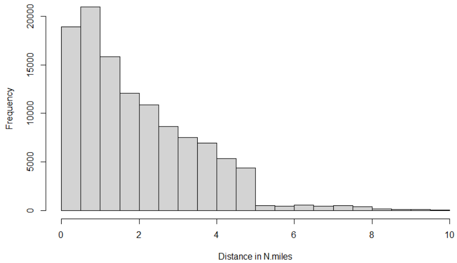
Figure 41. Cold Season of 2017 for Cloud-to-Ground
