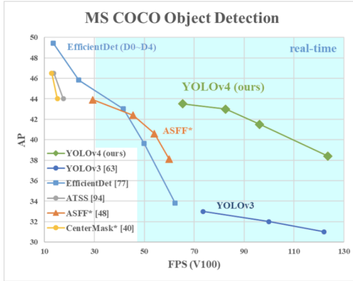
Figure 12: The performance of YOLOv4 compared to other models. [23]
