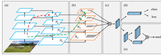
Figure 11: Path Aggregation Network Framework from [42]: (a) Feature Pyramid Network Backbone. (b) Bottom-up Path Augmentation. (c) Adaptive Feature Pooling. (d) Box Branch (e) Fully-connected Fusion.
