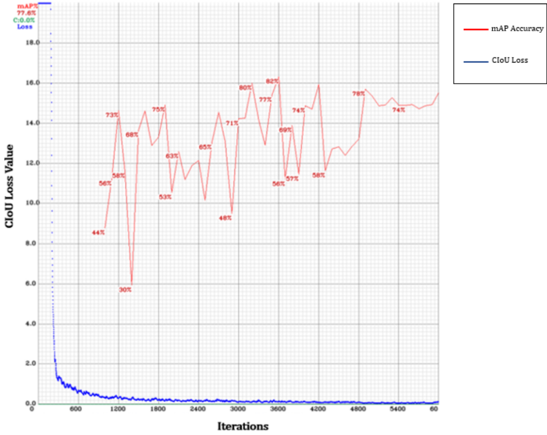
Figure 71: Experiment I: mAP vs. Clou Loss: Combined Dataset + DCGAN + Alien Test Set
