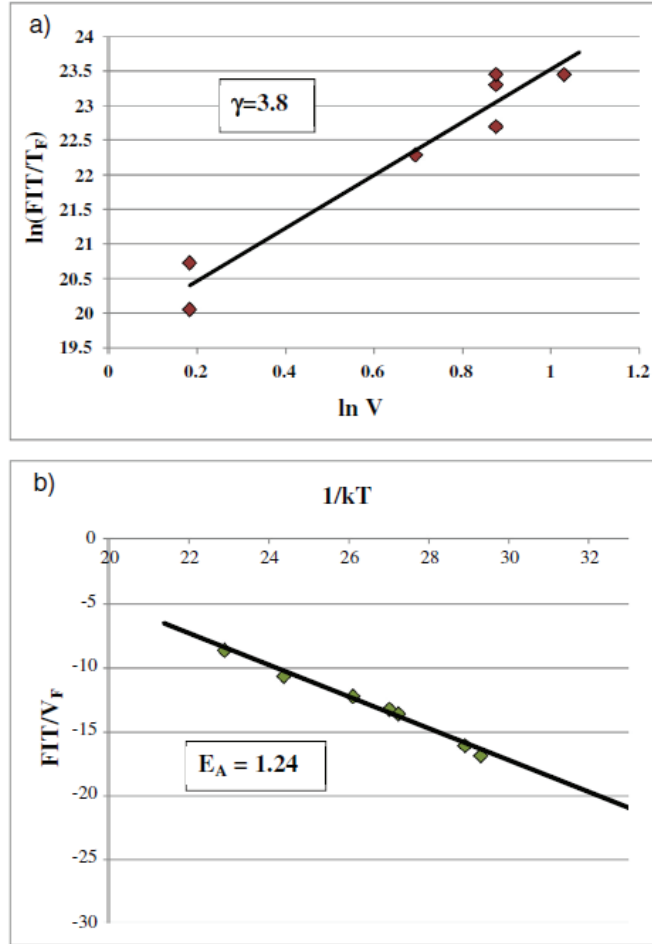
Figure 6. a) Gamma plot for EM at 45 nm. b) Activation energy plot for EM at 45 nm
