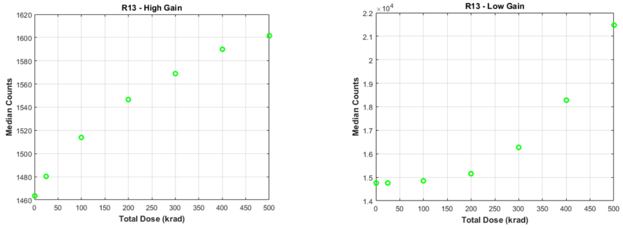
Figure 28. ROIC median counts increased with total dose, high and low gain.
