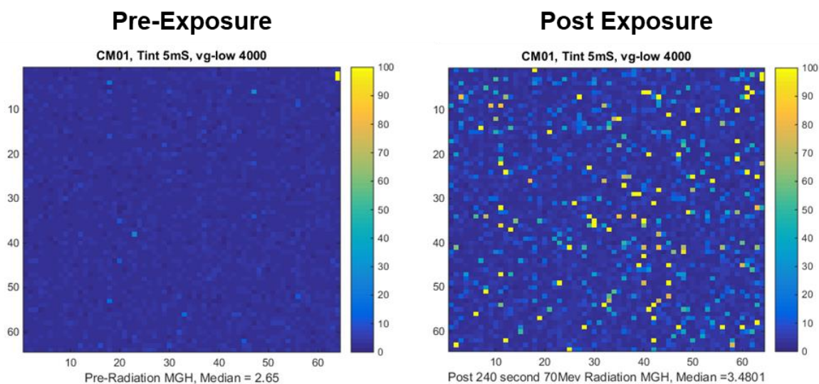
Figure 35. Maps of dark current in an InGaAs DFPA hybrid before and after proton exposure. Pixels with high dark current after exposure likely caused by extended cascade of displaced atoms.
