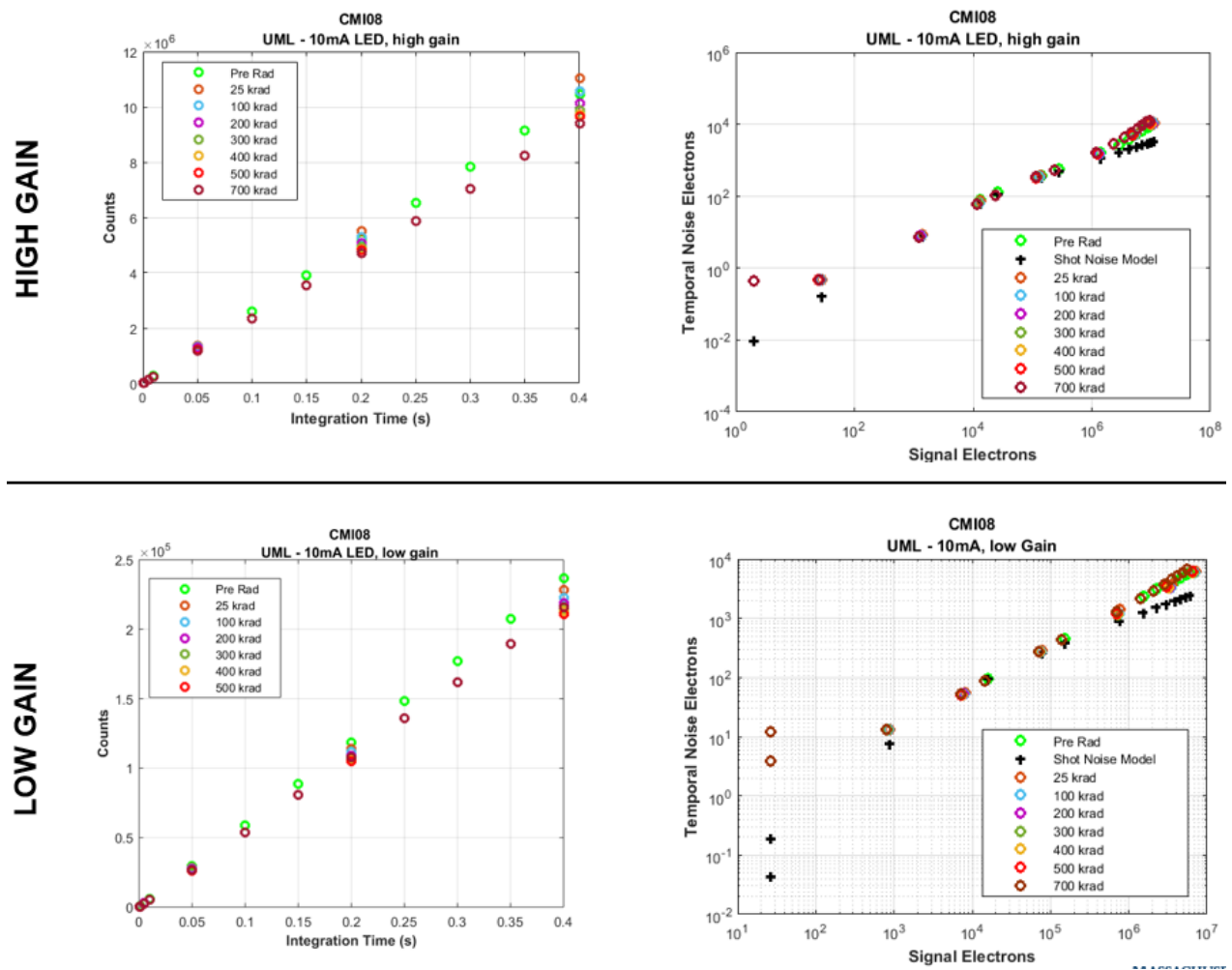
Figure 29. Hybrid counts and noise vs. signal after each dose for high and low gain.
