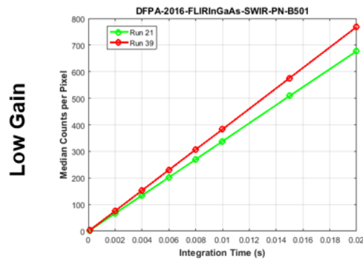
Figure 36. Median dark counts per pixel pre (green) and post (red) radiation for hybrids. Some curves of pre and post data exactly overlap, indicating no change from irradiation.
