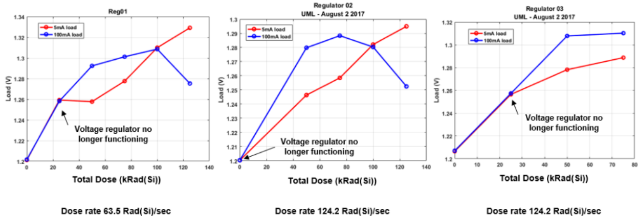
Figure 41. Voltage regulator performance as a function of total dose.
