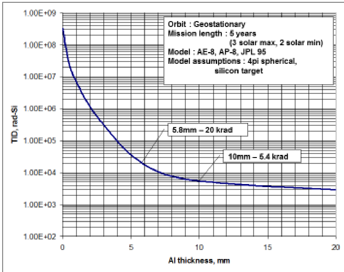
Figure 8. Geo TID dose-depth curve: the relationship between shielding thickness and total ionizing dose for aluminum shielding and silicon target for a 5-year mission.
