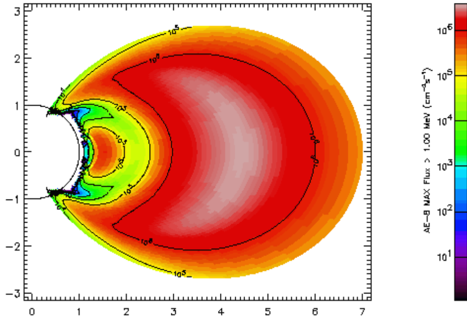
Figure 4. AE-8 cross-section flux map of trapped electron concentrations in a geomagnetic coordinate system.
