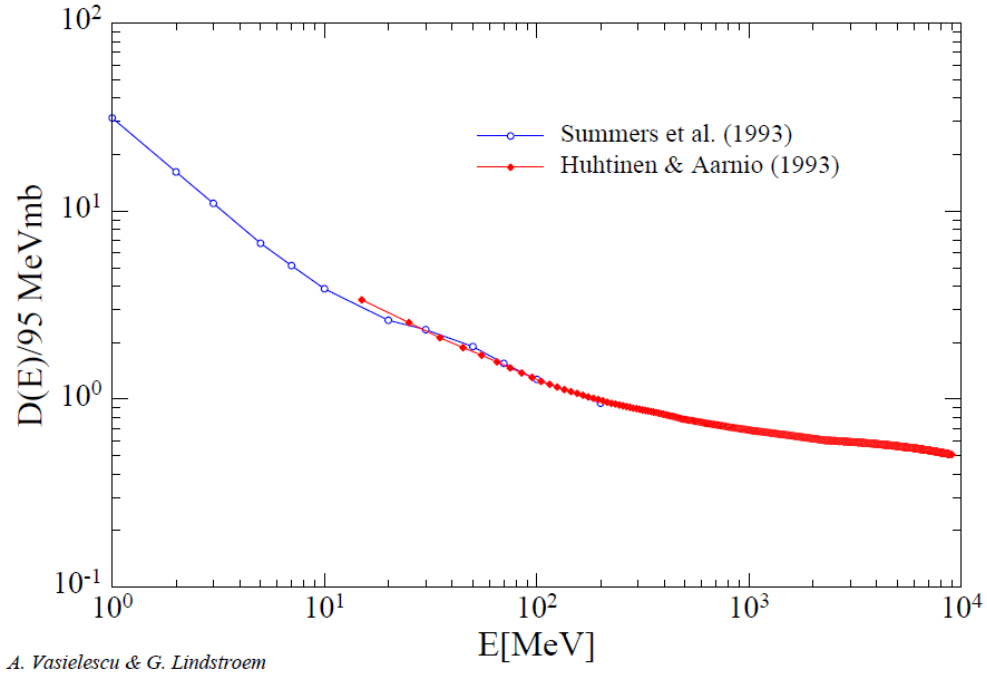
Figure 10. Proton displacement damage in Si. (Vasilescu & Lindstroem, 2000)
