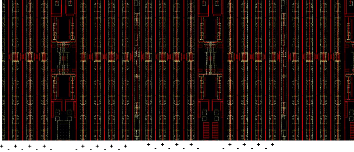
Figure 14. Layout example of substrate contacts showing the proximity of transistors to substrate contacts: the yellow-delineated areas are n-wells, and the red lines indicate long rows of contacts to substrate and n-wells. The spacing between the red vertical lines is 5 \mu\text{m} .
