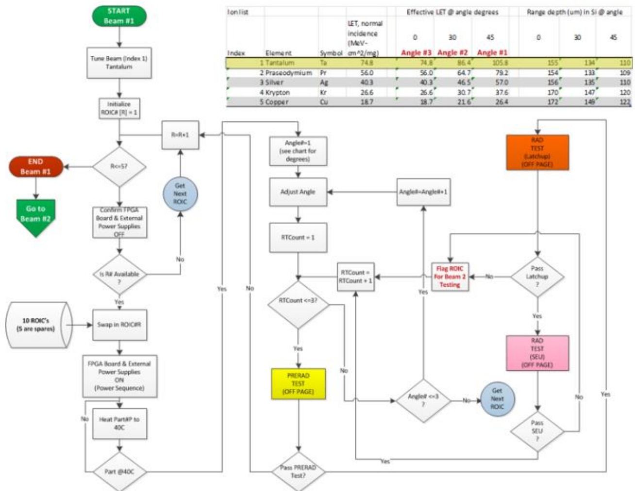
Figure 20. Selected beams and test protocol.
