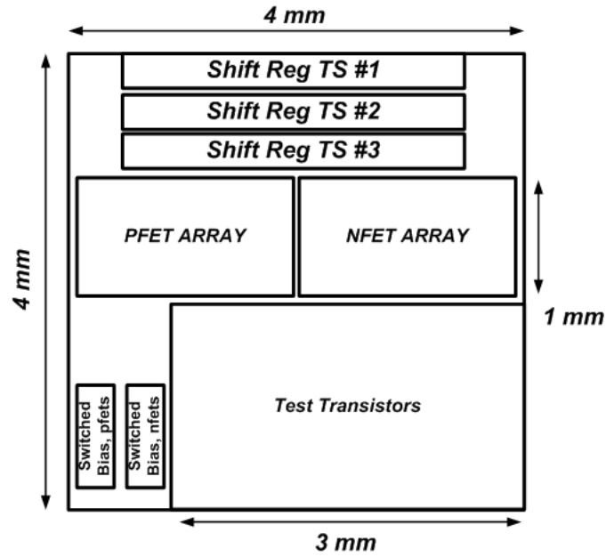
Figure 12. Test chip function blocks.
