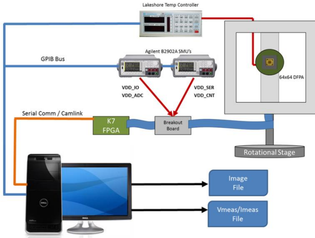
Figure 21. Test block diagram.
