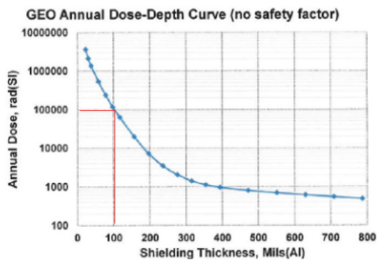
Figure 3.9-9. "Units internal to the host may take credit for 100 Mils of Al shielding"
