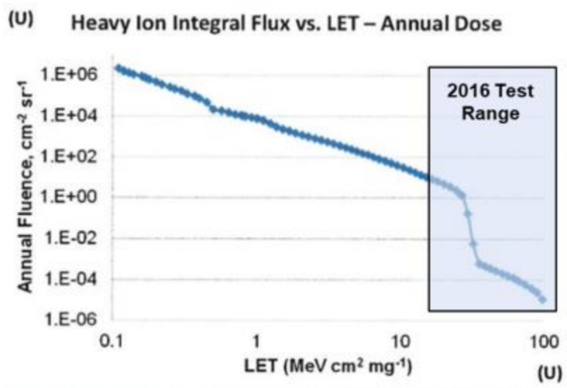
Figure 19. 2016 LET Test Range.
