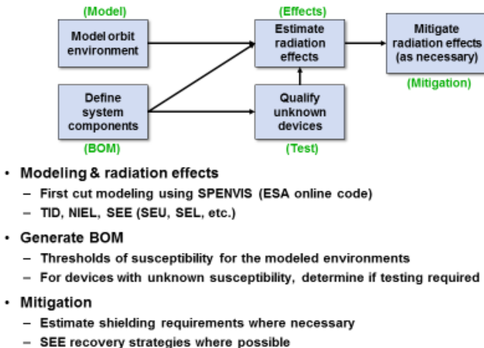
Figure 1. Radiation hardness assurance process. *Acronyms: Bill of Materials (BOM); SPace ENVironment Information System (SPENVIS); European Space Agency (ESA); Total ionizing dose (TID); Non-ionizing energy loss (NIEL); Single-event effect (SEE); Single-event upset (SEU); Single-event latch-up (SEL).
