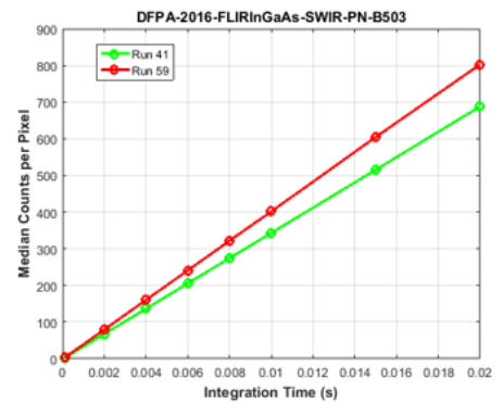
Figure 36. Median dark counts per pixel pre (green) and post (red) radiation for hybrids. Some curves of pre and post data exactly overlap, indicating no change from irradiation.
