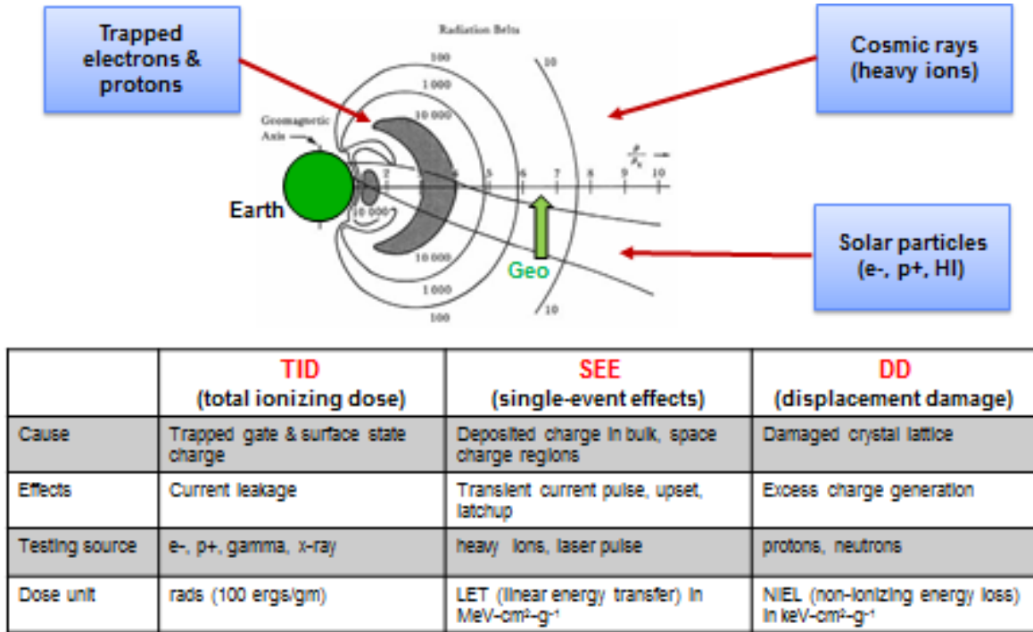
Figure 2. Space radiation environment and effects.
