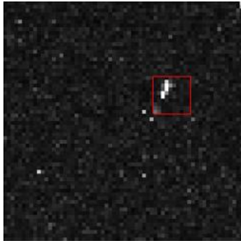
Figure 34. An example of single event effects observed during proton irradiation.
