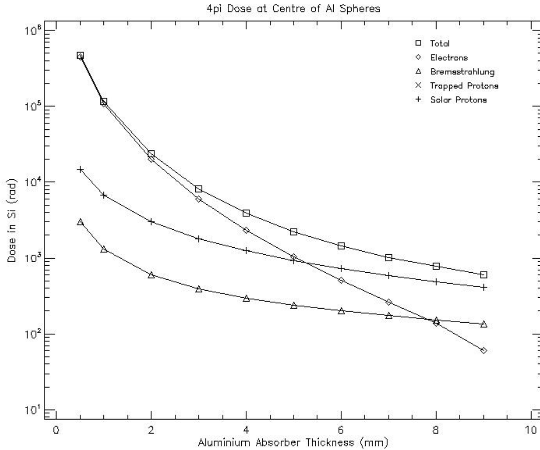
Figure 7. TID radiation components, depth-dose for 1-year mission.
