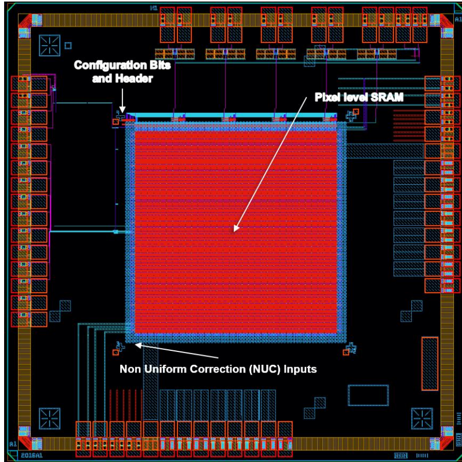
Figure 13. Location of storage registers of the DTA ROIC.
