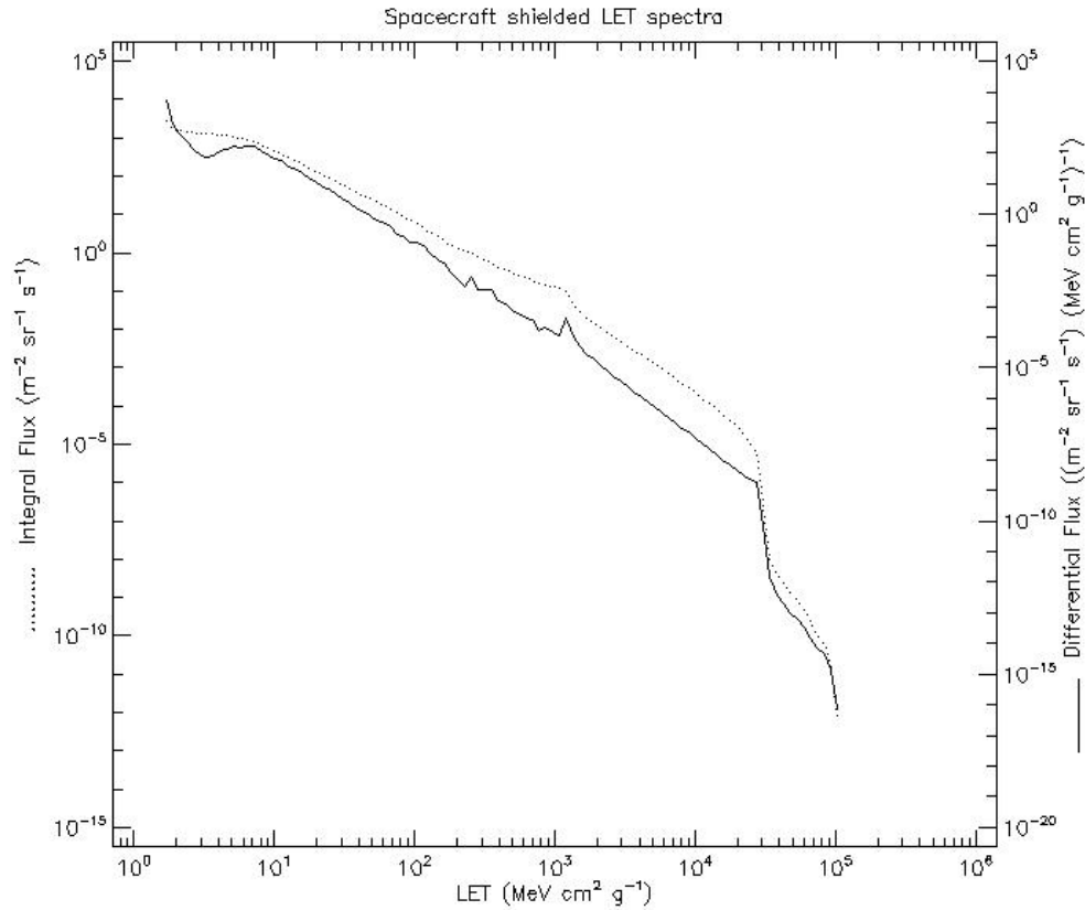
Figure 9. LET spectral flux.
