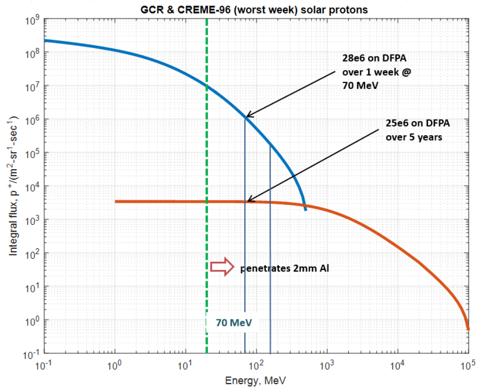
Figure 11. Solar proton energy spectrum.
