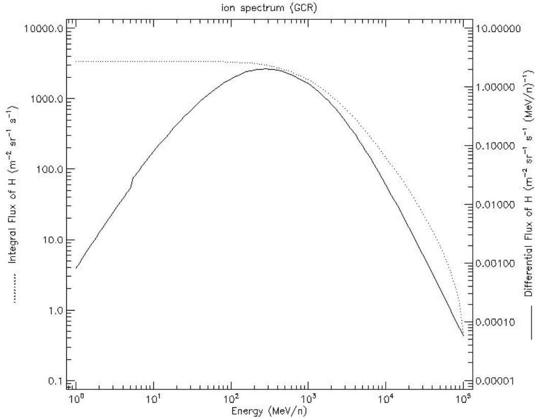
Figure 6. Cosmic ray spectral energy flux.
