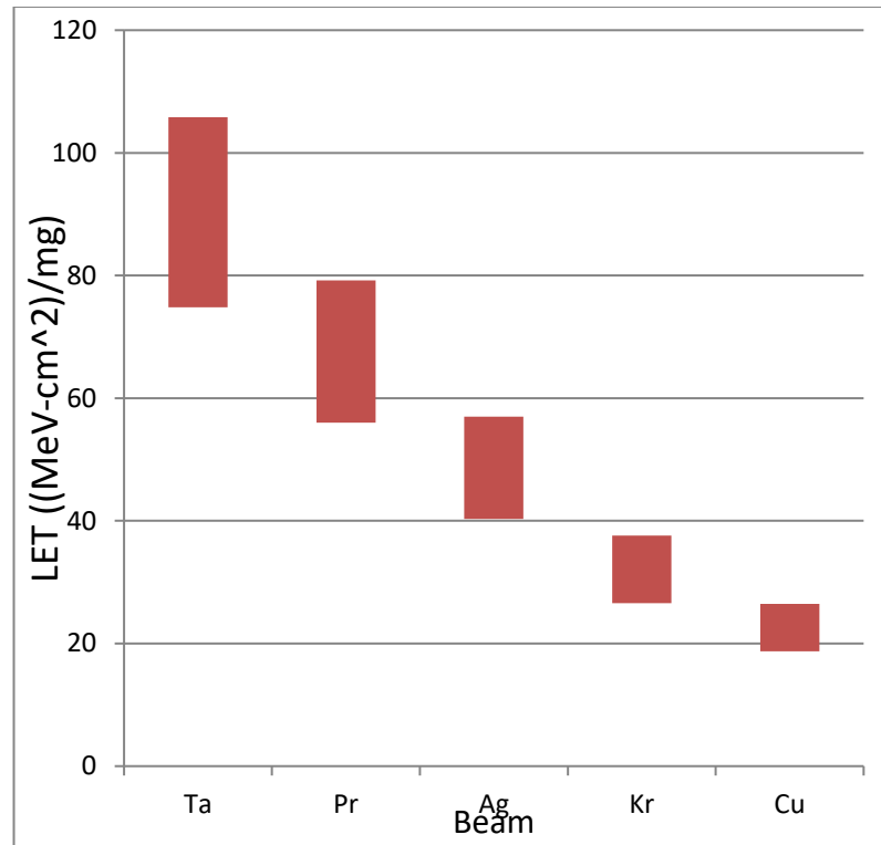
Figure 17. Selected ion LET coverage.
