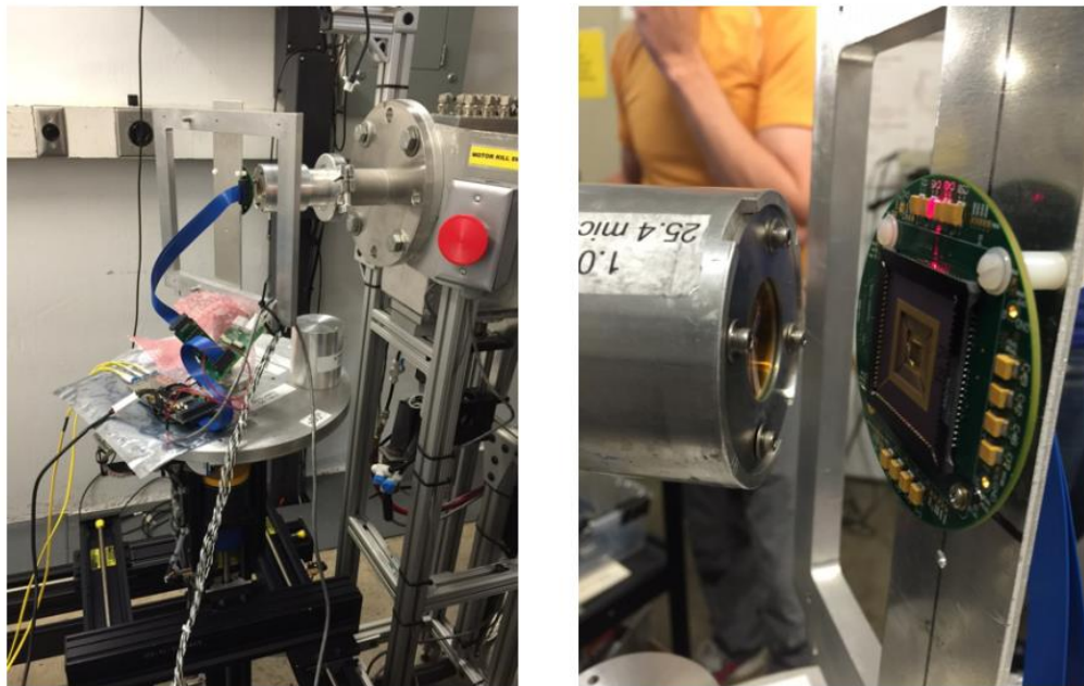
Figure 23. Alignment of DUT with beam.
