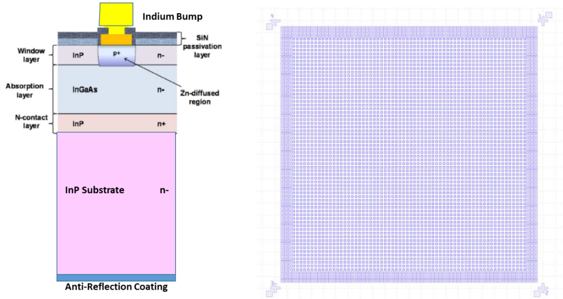
Figure 15. (Left) Typical cross-section of InGaAs photodiode (based on SPIE Proceedings 945105-1, A. Rouvie et al, 2015); (right) 64 x 64 array layout showing pixel contacts and common contacts around periphery.
