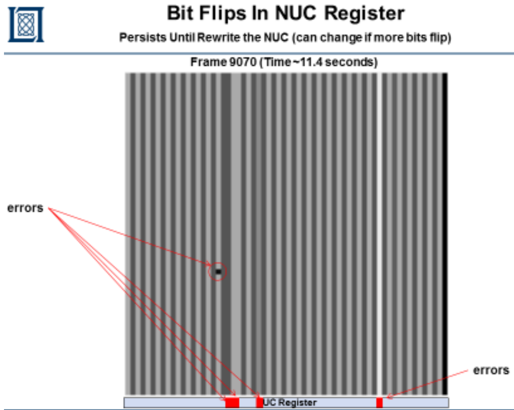
Figure 24. Heavy ion tests 2016 - SEFI bit flips.
