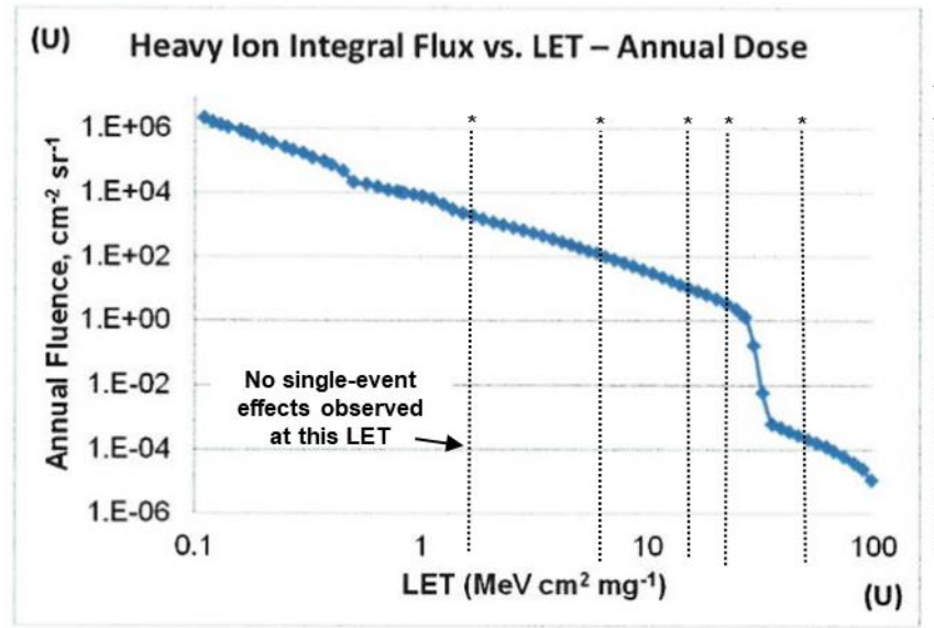
Figure 30. LET levels selected for this round of radiation testing (TAMU May 2017).
