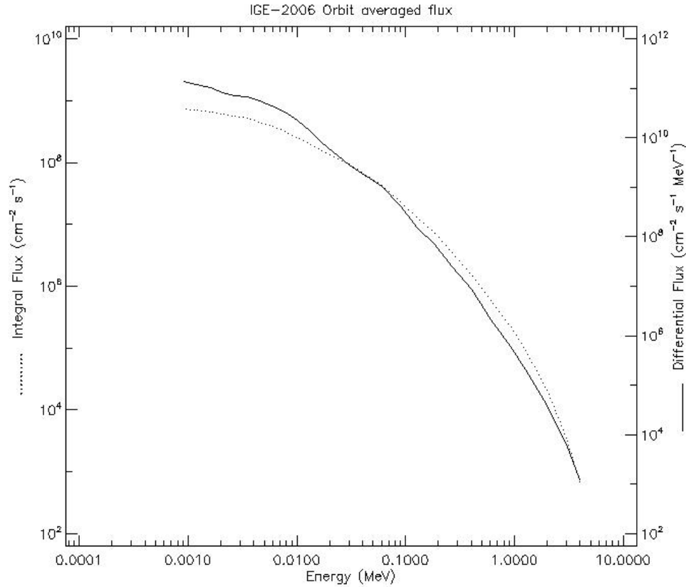
Figure 3. Trapped electron spectral flux from an IGE-2006 model assuming a geosynchronous orbit.
