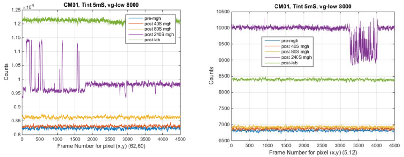
Figure 27. Dark counts per pixel over 4500 frames for hybrid CM01 at the pre-radiation test and after each level of irradiation for the 70 MeV beam energy, high gain. “Post-lab” means the data was taken several days after the radiation testing at MIT LL.
