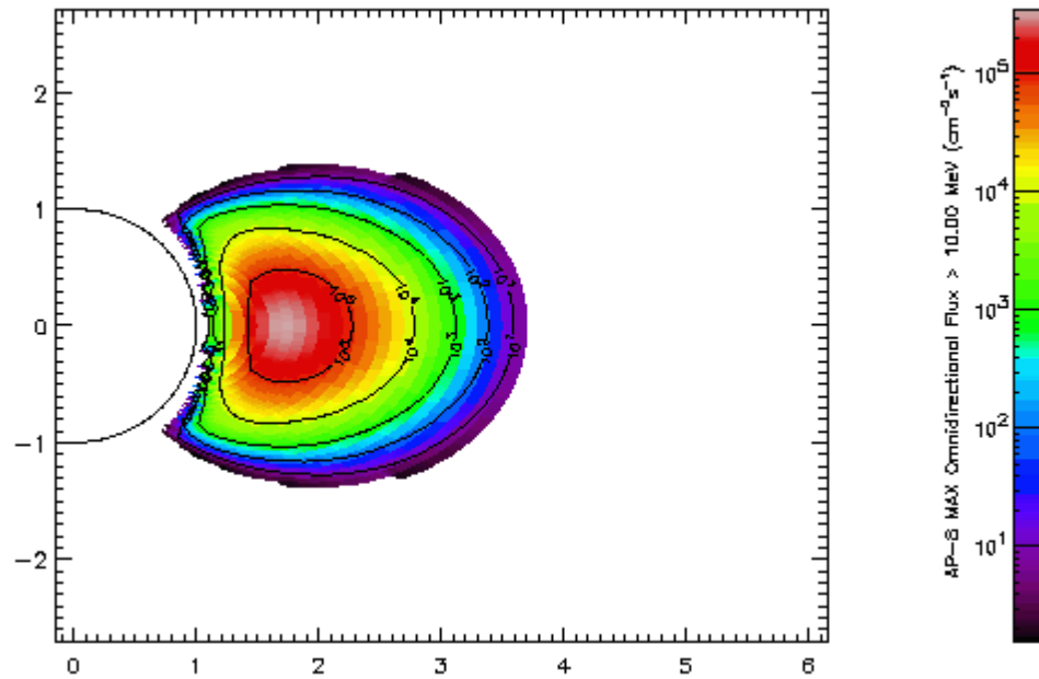
Figure 5. AP-8 cross-section flux map of trapped proton concentrations in a geomagnetic coordinate system.
