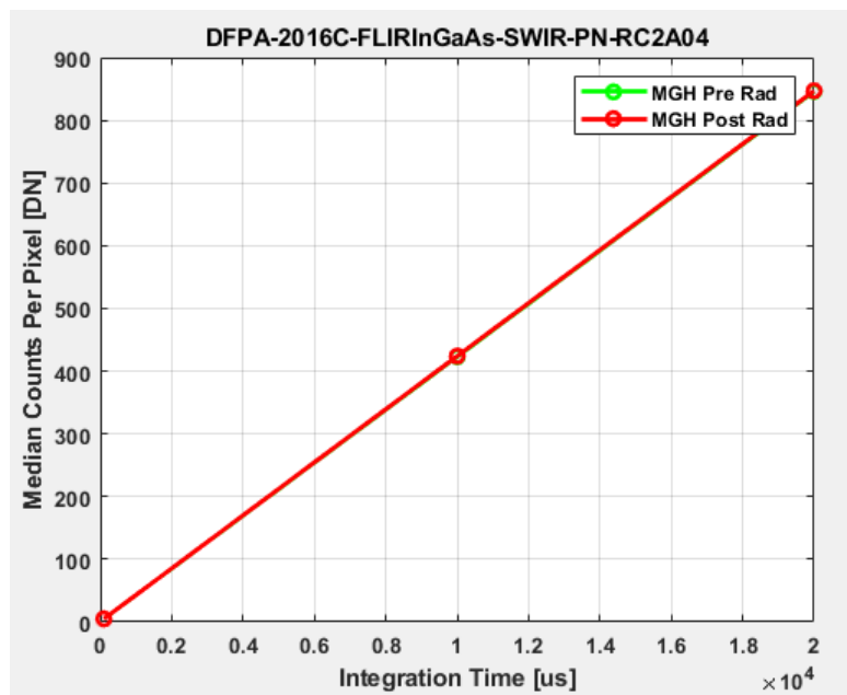
Figure 42. Leakage counts pre- and post-radiation.
