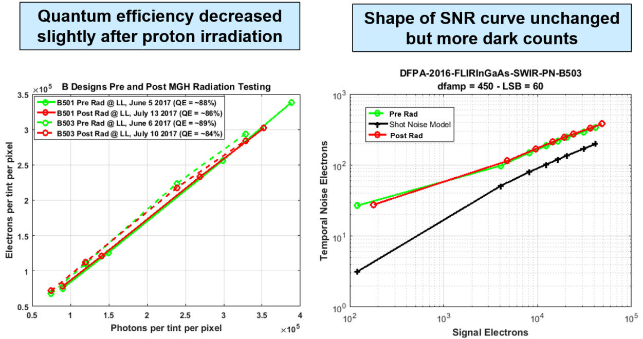
Figure 37. Quantum efficiency and signal-temporal noise curves for hybrids.
