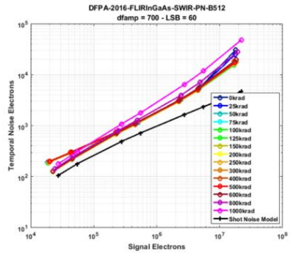
Figure 40. Quantum efficiency and signal-noise over course of radiation exposure.
