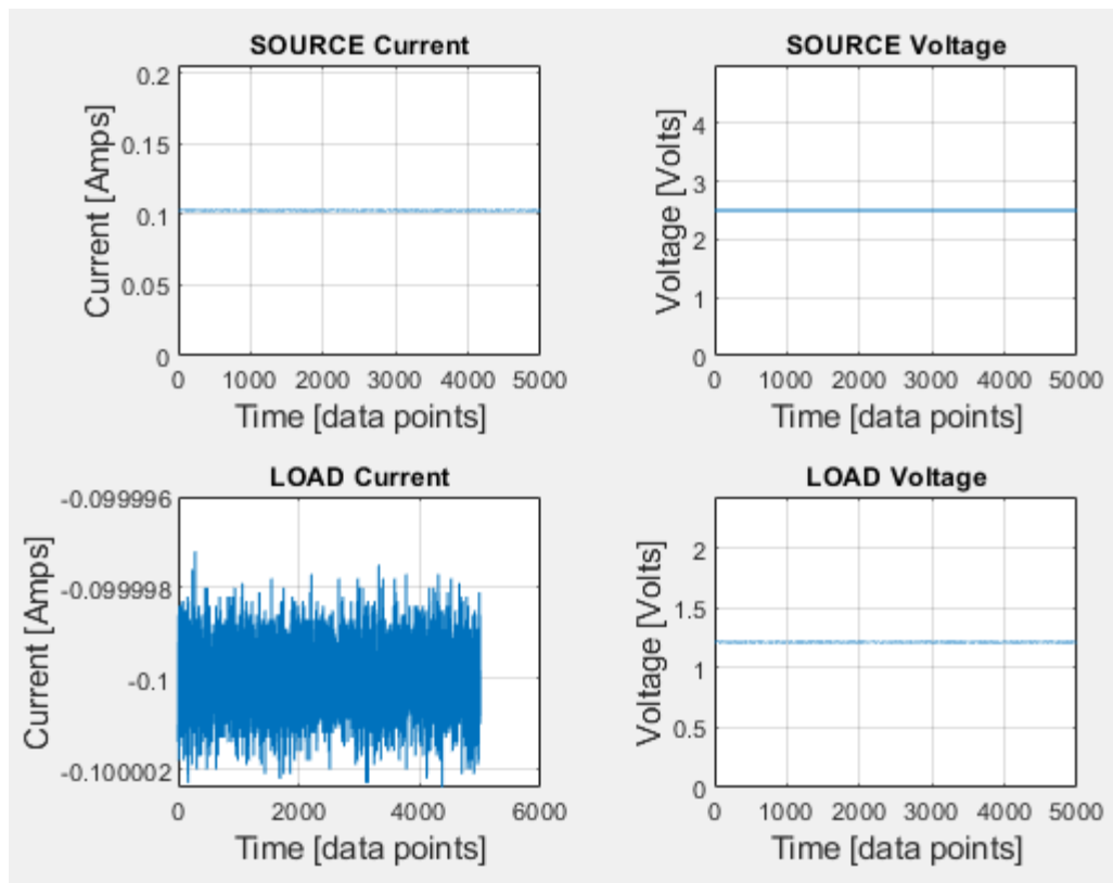
Figure 43. "Left" regulator after 10 kRad total dose.
