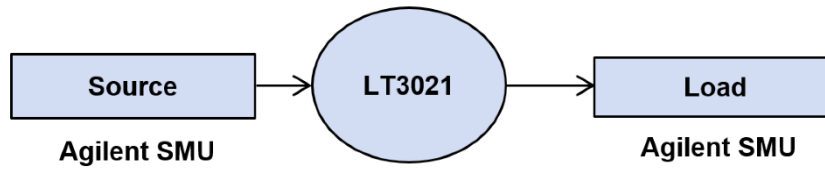
Figure 32. Voltage regulator test block diagram.
