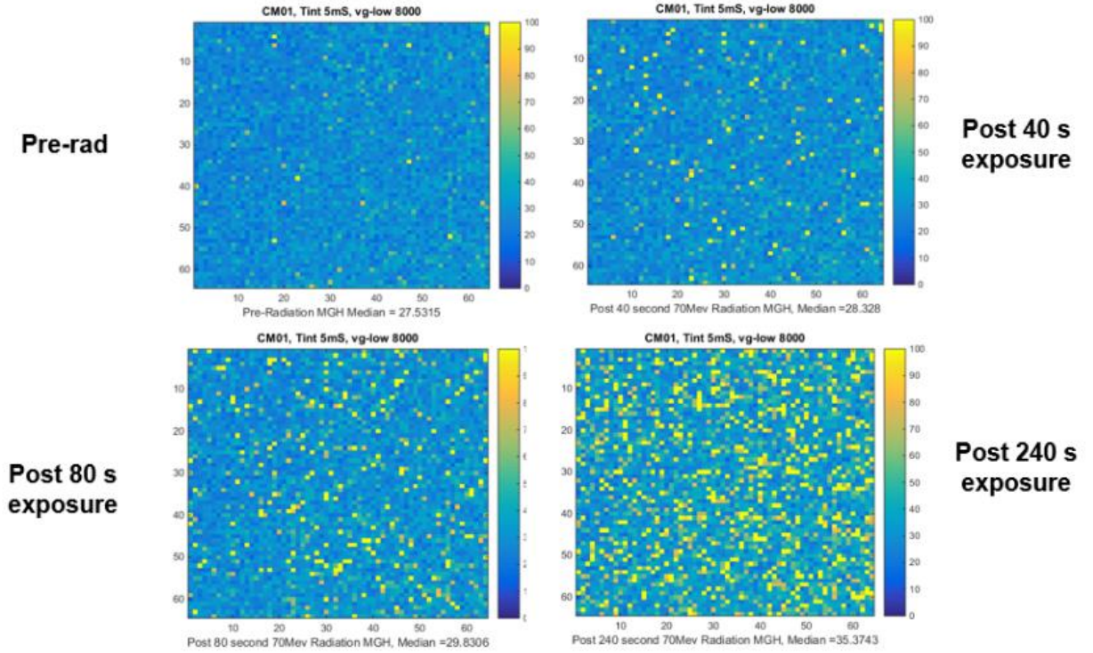
Figure 26. Pixel standard deviation for hybrid CM01 at the pre-radiation test and after each level of irradiation for the 70MeV beam energy, high gain.
