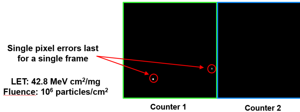
Figure 31. This image shows the single pixel errors that were observed during irradiation. These effects were not persistent and only appeared for one frame before being resolved.
