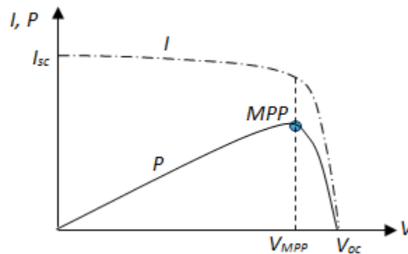
Figure 47. PV array typical I-V and P-V features. Source: [48].
