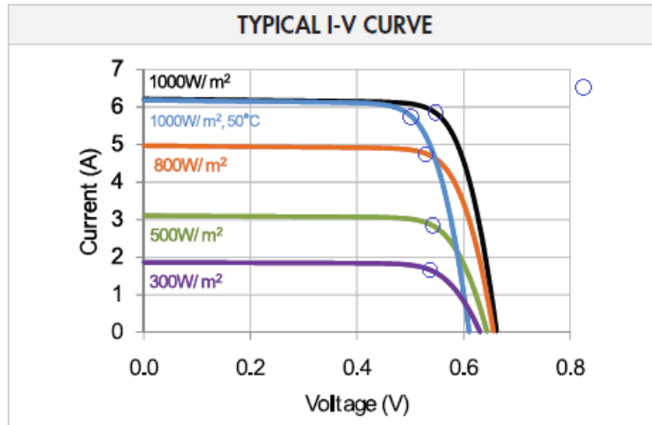
Figure 48. Sun-power solar cell voltage-current curve. Source: [50].
