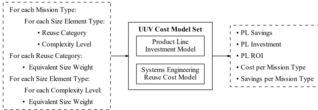
Figure 3.5. Inputs and Outputs for COSYSMO Analysis. Source: [20].
