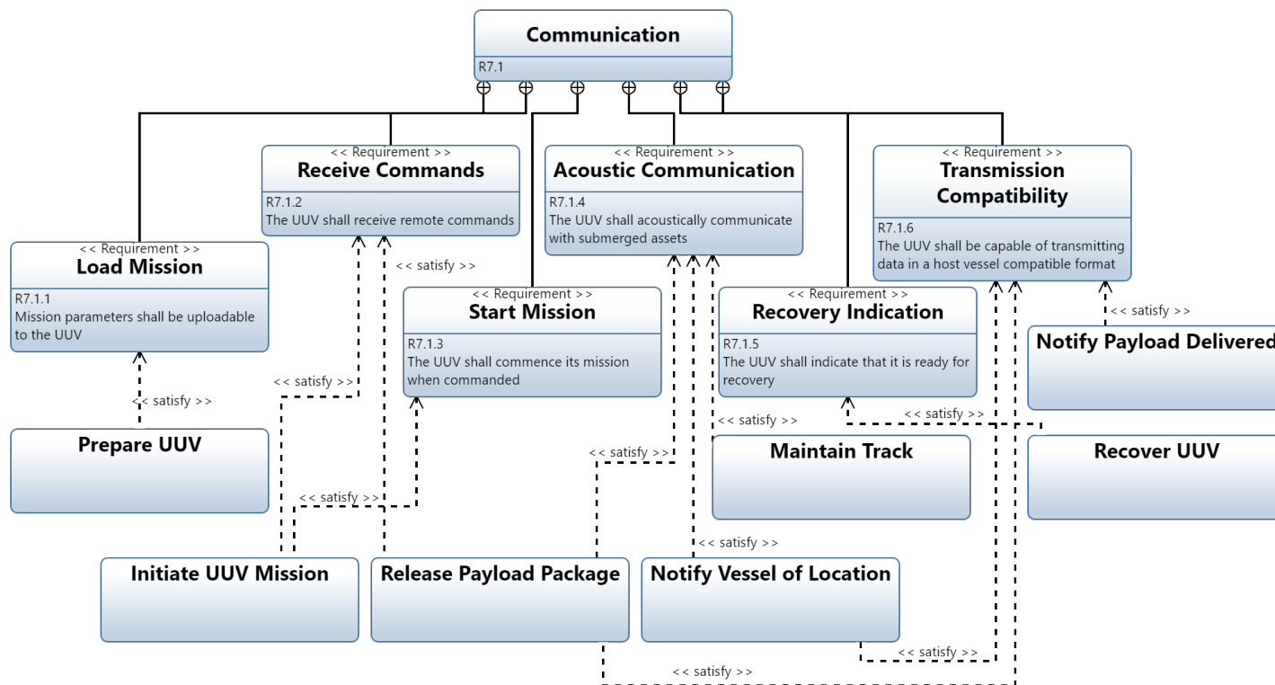
Figure A.59. PD Communication Requirement Decomposition Diagram
