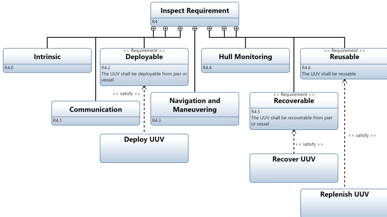
Figure A.42. INID Requirement Diagram
