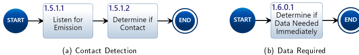
Figure A.2. ISR Activity Decomposition Diagrams
