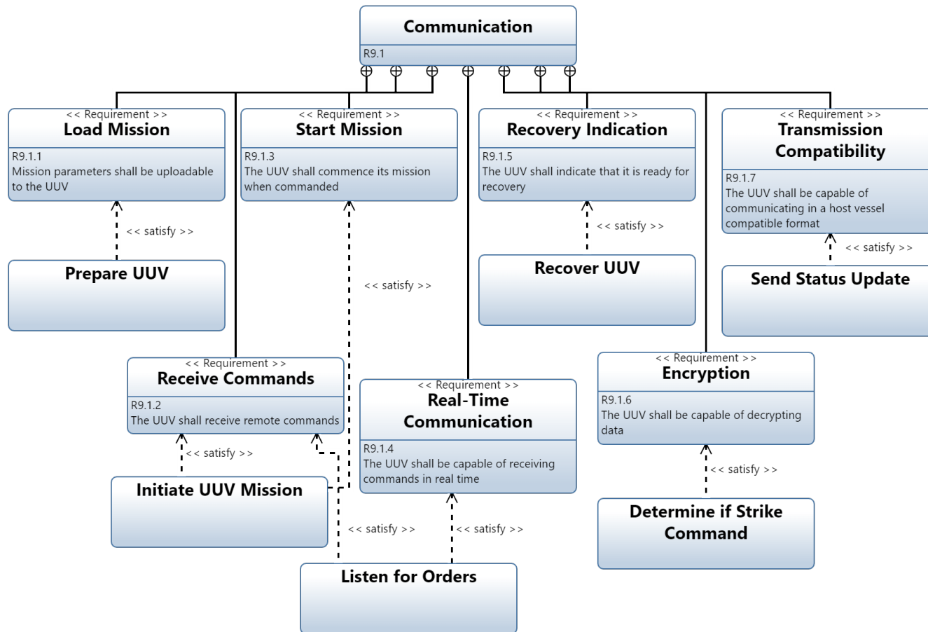
Figure A.70. TCS Communication Requirement Decomposition Diagram
