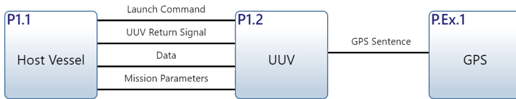
Figure A.17. ISR Interface Diagram
