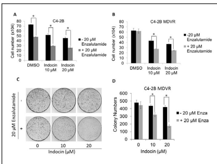
Figure 15 Growth inhibition of C4-2B parental (A) and MDVR (B) cells by indocin in combination with enza. Clongenic assays: C. Colony pictures of of C4-2B cells treated with Indocin and enza, and D. results
