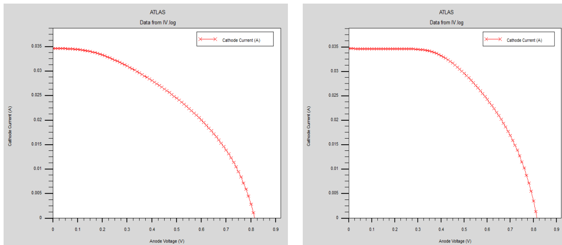
Figure 48. Increasing CdS thickness. Left: 0.10 \mu\text{m} , right: 0.30 \mu\text{m} .
