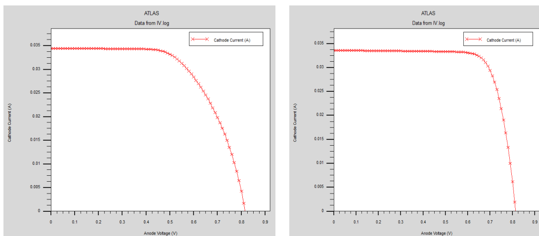
Figure 47. Increasing ZnO thickness. Left: 0.10 \mu\text{m} , right: 0.30 \mu\text{m} .
