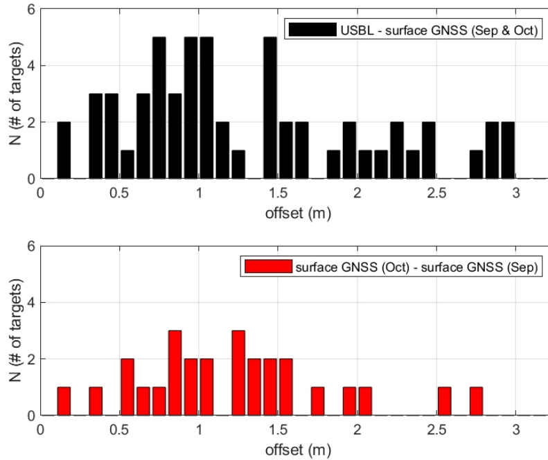
Figure 13. Empirical distributions of measured spatial differences for each target between the geolocation techniques (upper graph) and survey times (lower graph).
