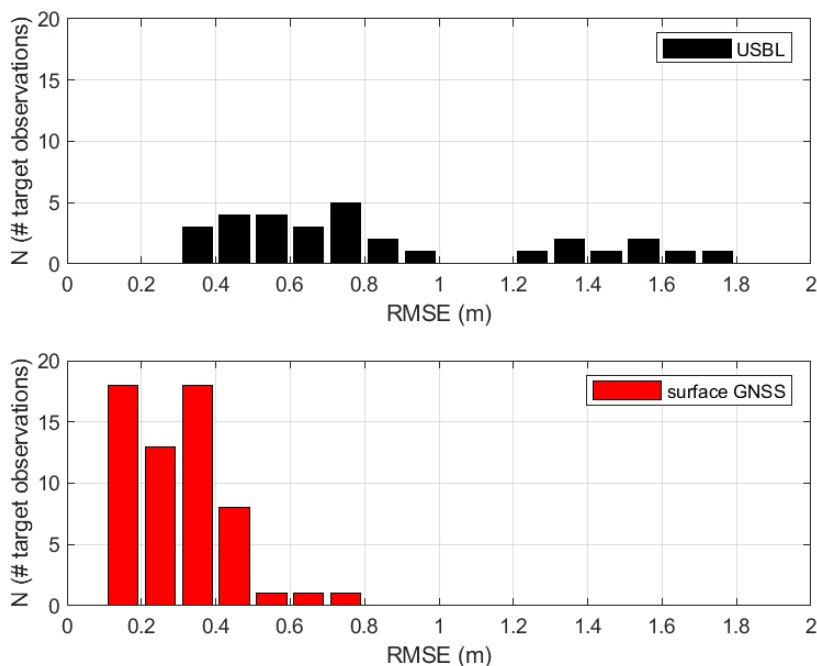
Figure 14. Distributions of root mean square error (RMSE) for each target position derived from the USBL and surface GNSS buoy geolocation techniques.
