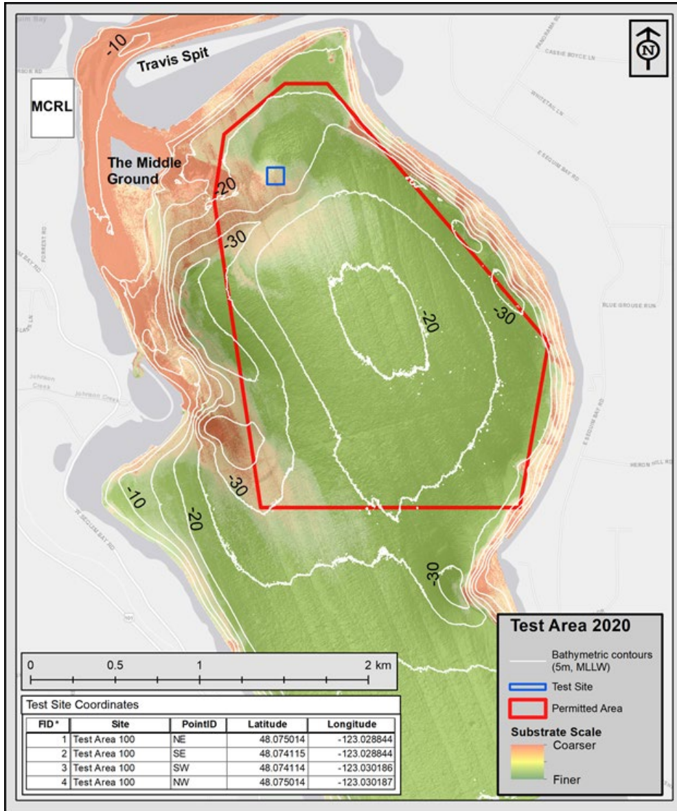
Figure 1. Location of the Sequim Bay Underwater Testbed (blue box) for the 2020 field season.
