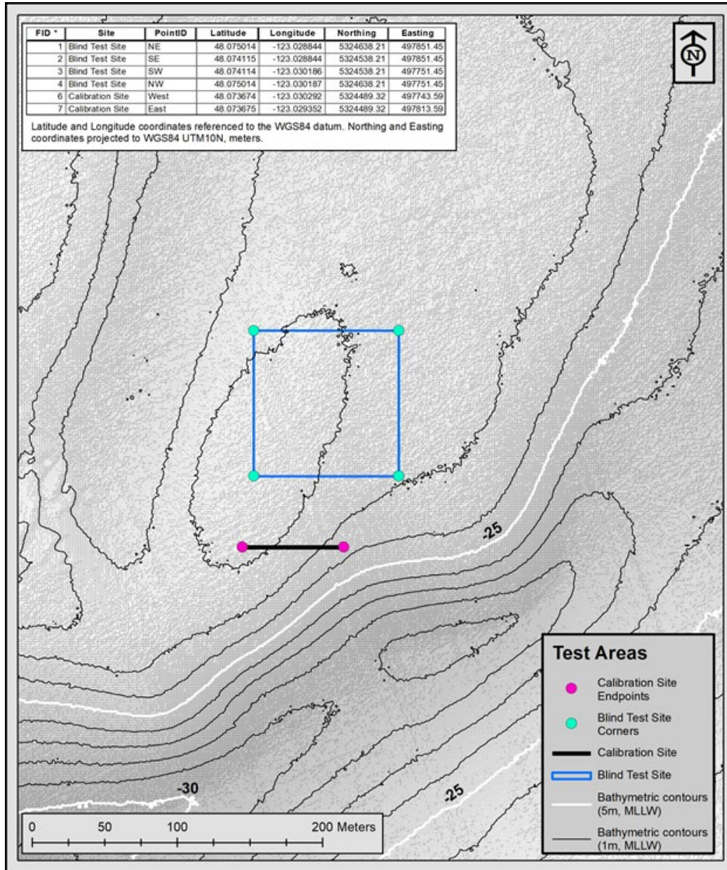
Figure 2. Location of the calibration site (black line) and blind site (blue box) in Sequim Bay for 2020.
