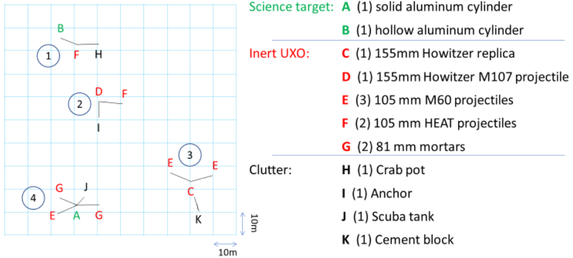
Figure 6. Blind site design showing the approximate locations of the 15 targets in the 100 x 100 m blind test grid. Circled numbers indicate the cluster number. The list on the right provides the target key and the number of each target type in parentheses ( ).
