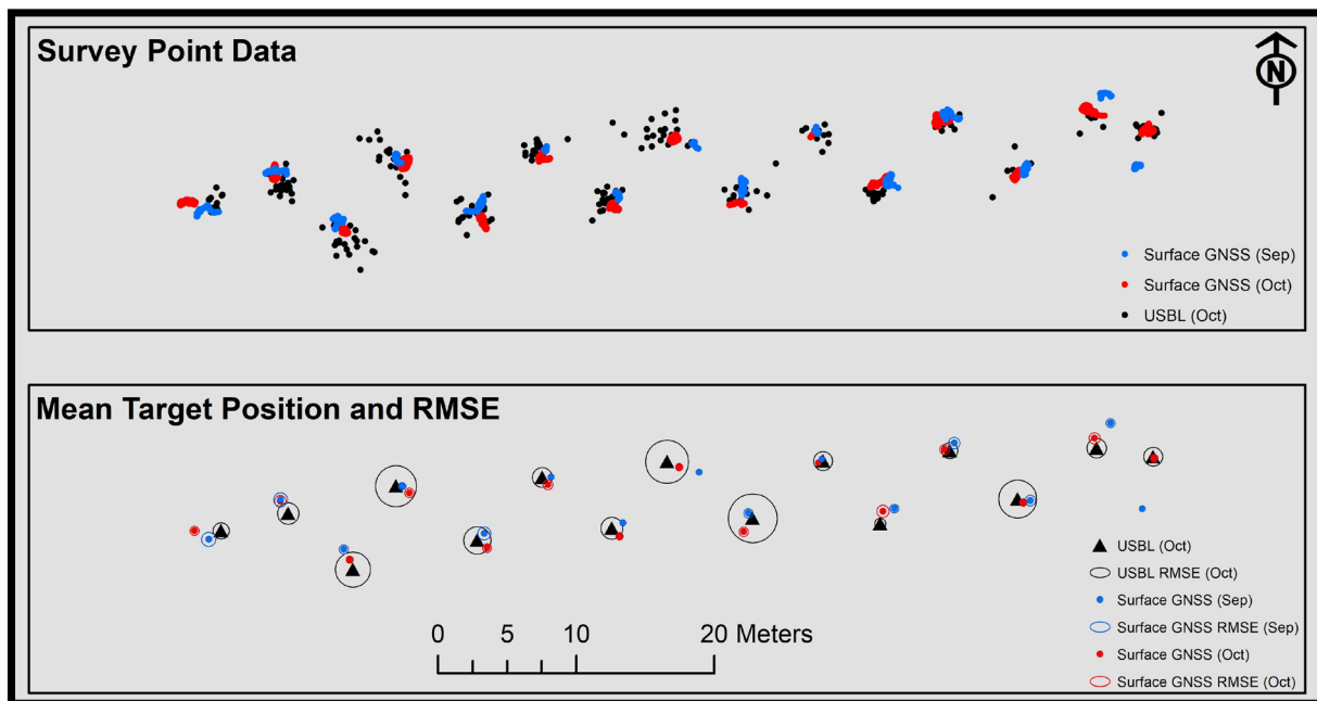
Figure 9. Maps of target geolocation positions along the calibration site baseline derived from the surface GNSS buoy surveys and the USBL positioning systems.
