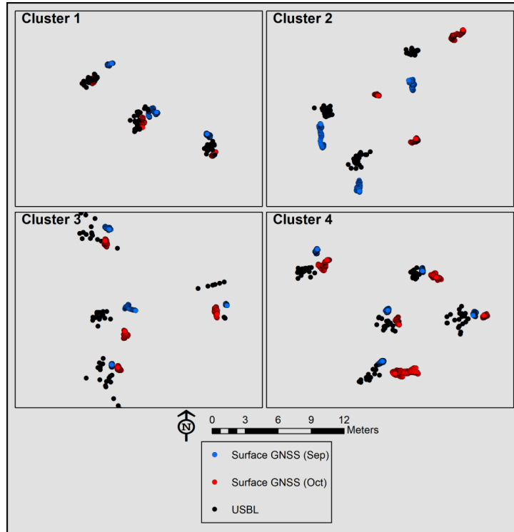
Figure 10. Target point clouds from processed positions for each cluster at the blind site, collected by the surface GNSS and USBL systems.
