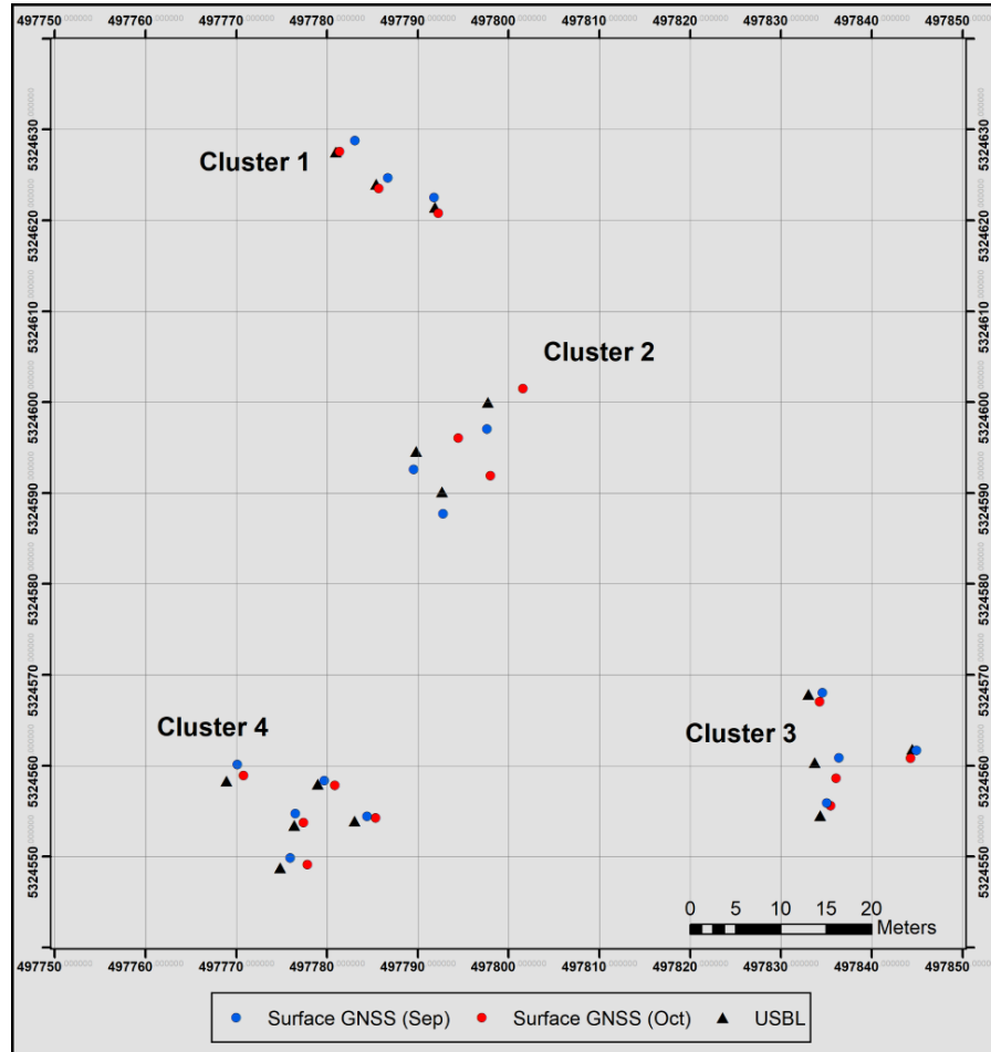
Figure 12. Blind site cluster locations relative to the 100 x 100 m site grid. Points represent mean target position as determined by the surface GNSS and USBL systems in September and October.
