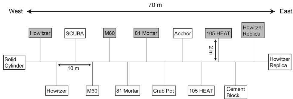
Figure 4. Layout of the targets at the calibration site. Targets shaded gray were buried flush with the sediment surface. Targets shown in white were placed proud on the surface. Numbers indicate the distance along the baseline.
