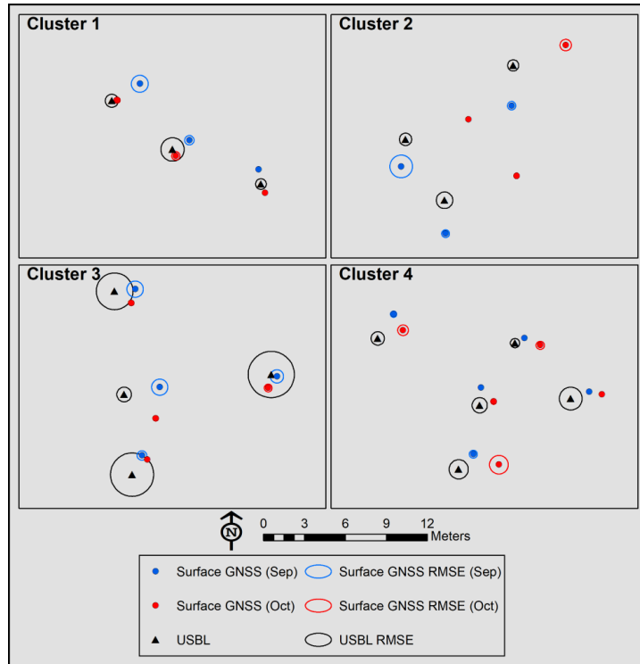
Figure 11. Relative mean target positions and associated RMSE for targets within each cluster at the blind site.
