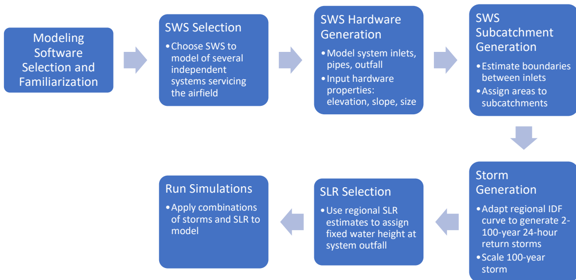
Figure 6: Methodology Flowchart
