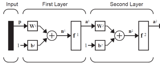
Figure 5. Neural Network Conceptual Model with One Neuron in the First Layer and One Neuron in the Second Layer for each Element of the Input Column Vector \mathbf{p} [37].
