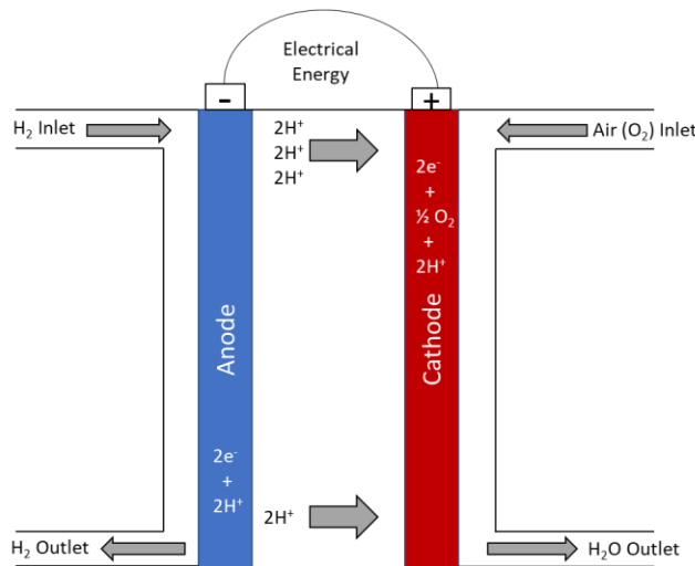
Figure 3: Fuel Cell Schematic
