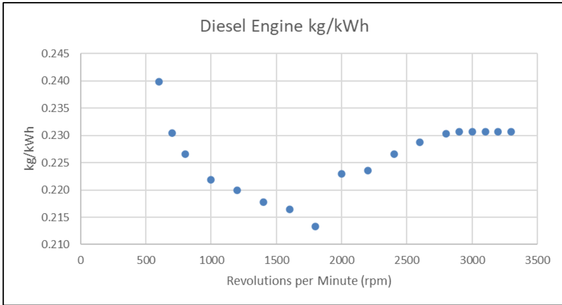
Figure 11: Diesel Engine kg/kWh versus rpm (Data obtained from (Cummins, 2013))
