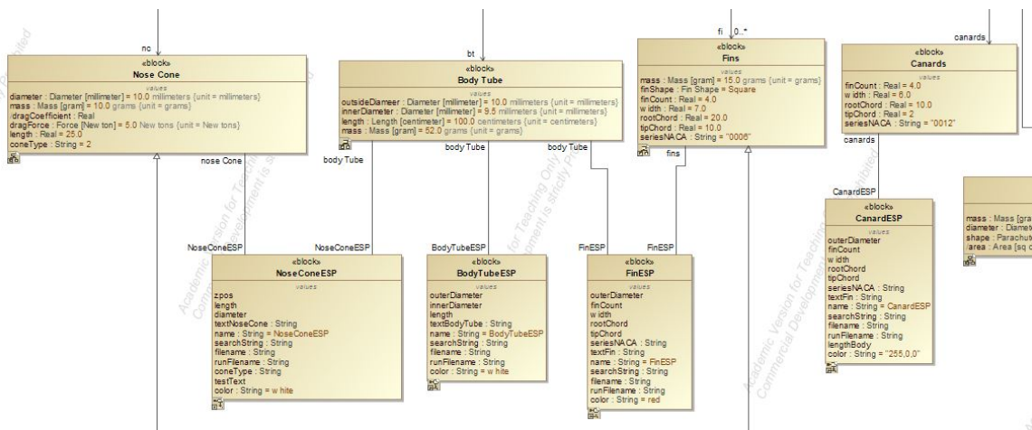
Figure 25: Rocket Model Physical Decomposition Showing Multiple Association Paths
