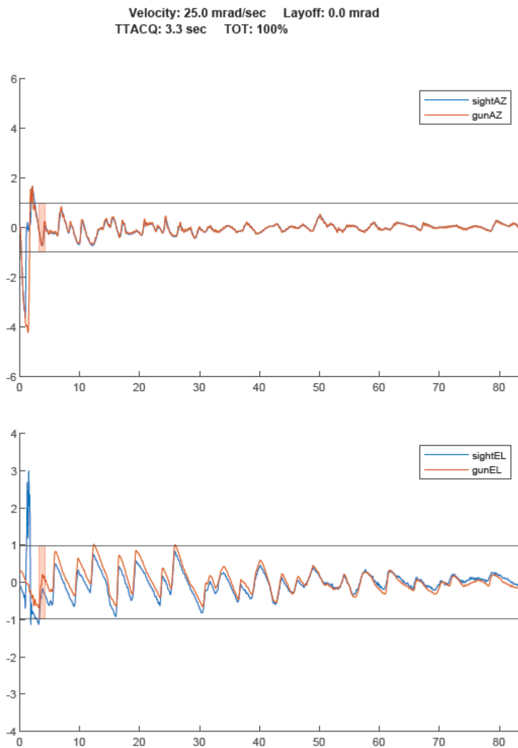
Figure 8. Target tracking plot.
