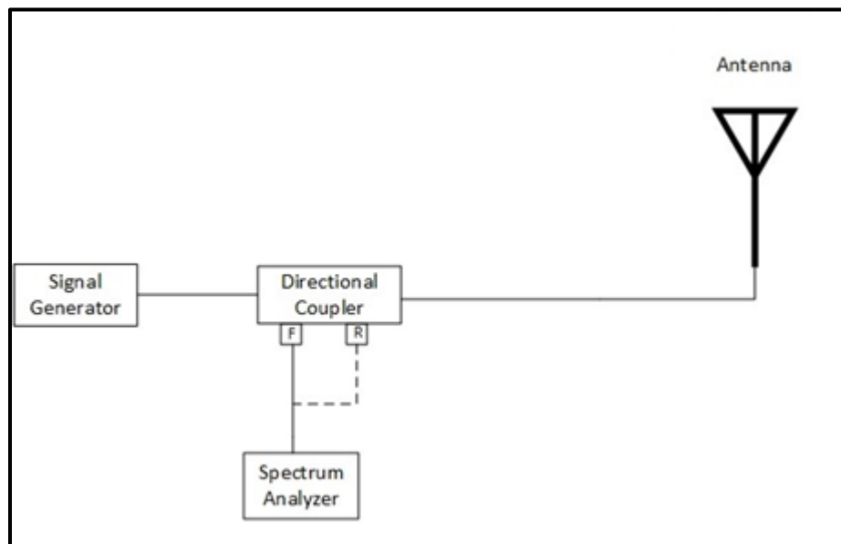
Figure 2. VSWR manual method measurement setup.
