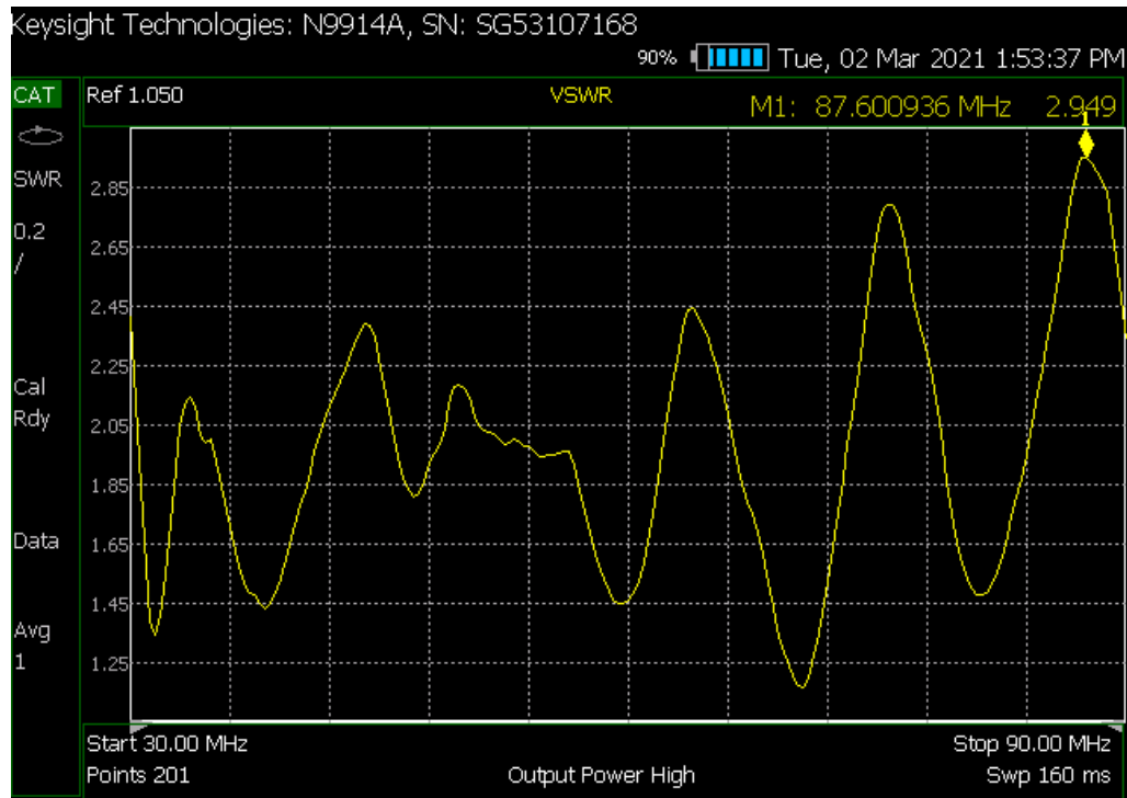
Figure 5. VSWR plot.
