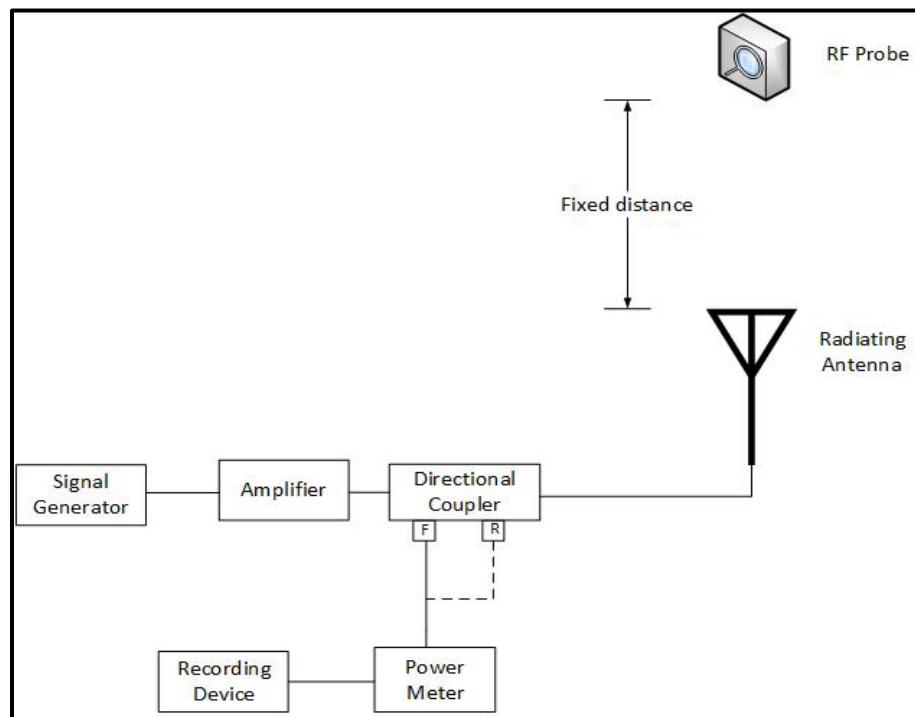
Figure 3. Recorded method calibration setup.
