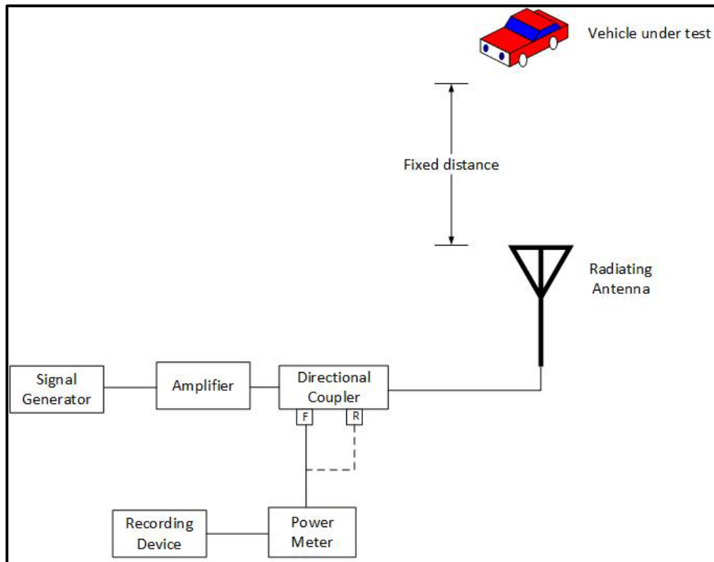
Figure 4. Recorded method testing setup.
