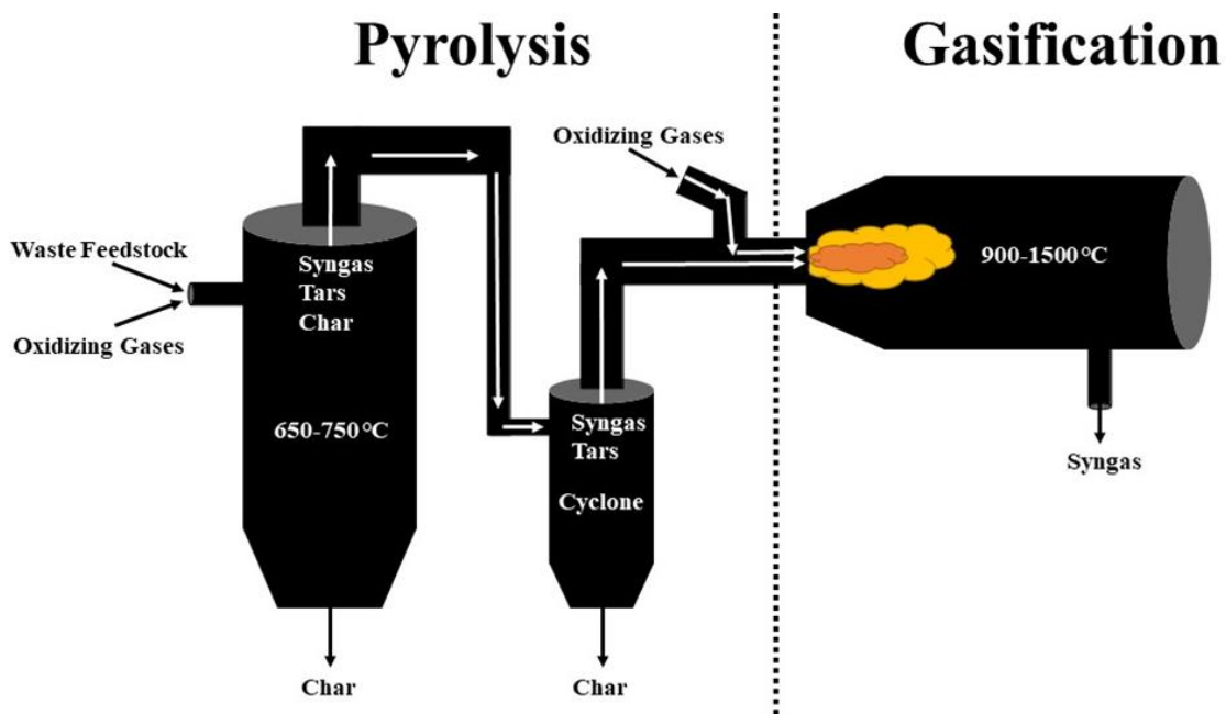
Figure 4. Schematic representation of a multi-stage gasification process
