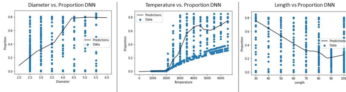
Figure 16. DNN model for diameter, temperature, and length predictions vs. dataset
